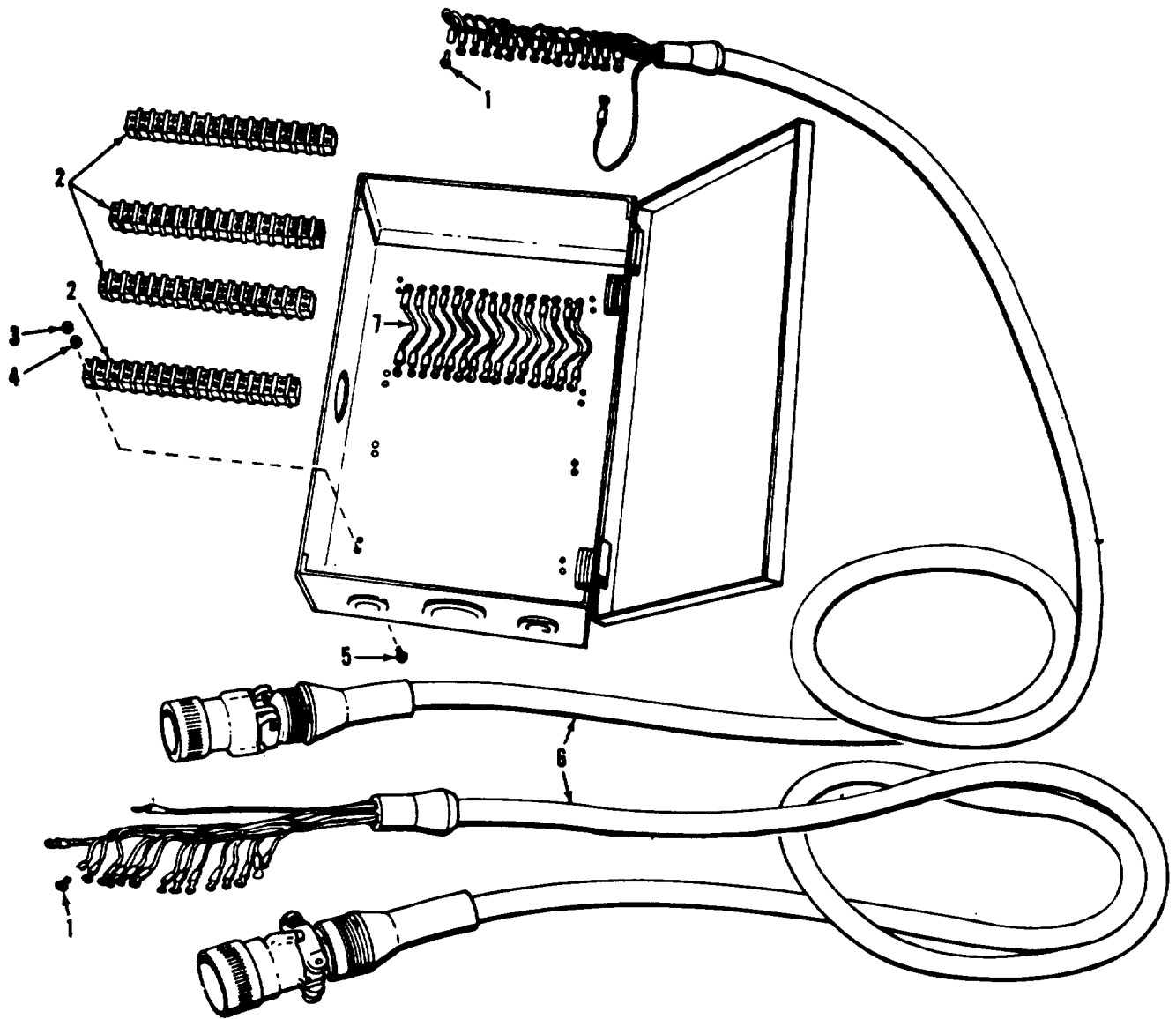
Figure 7. Terminal box assembly-partially exploded view.
