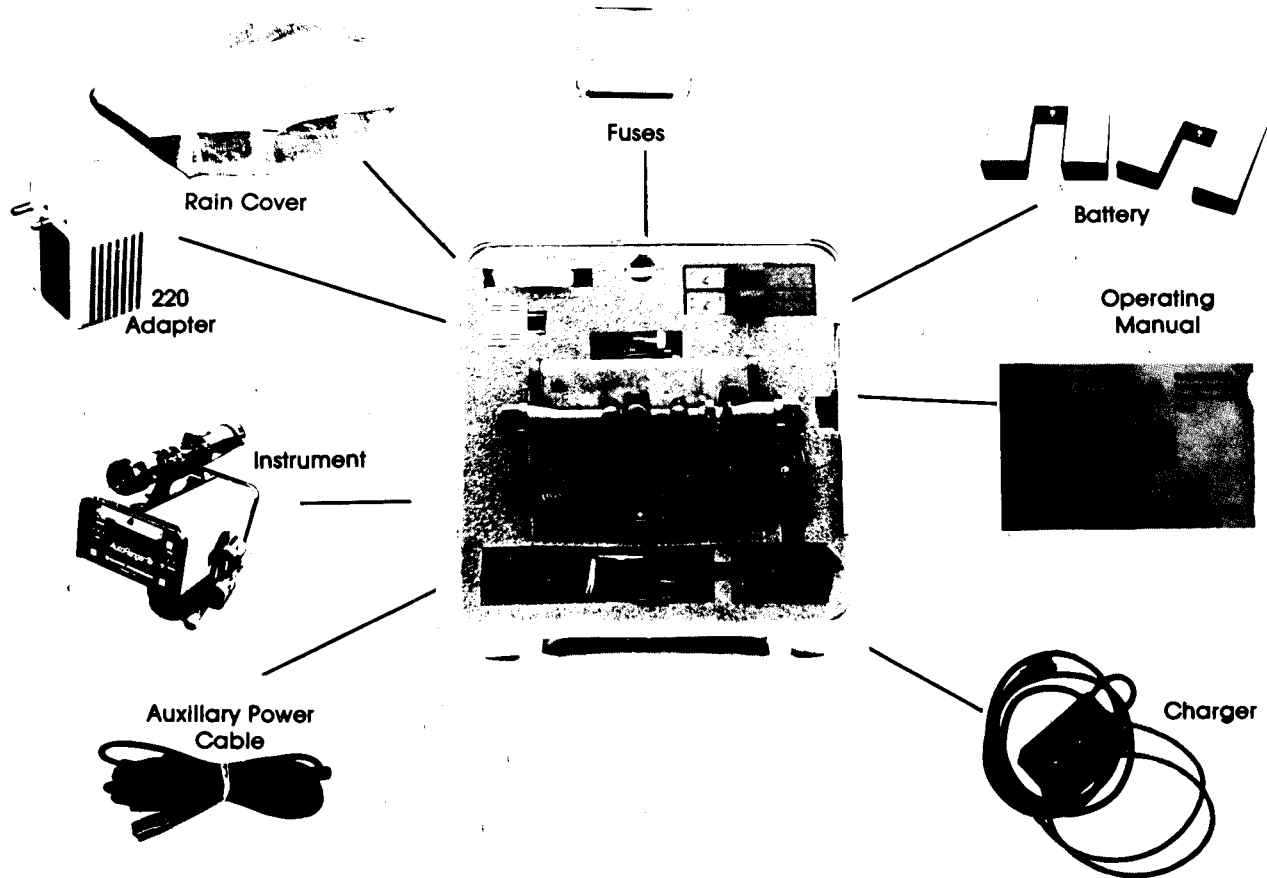
Figure 3 - Instrument Assembly
