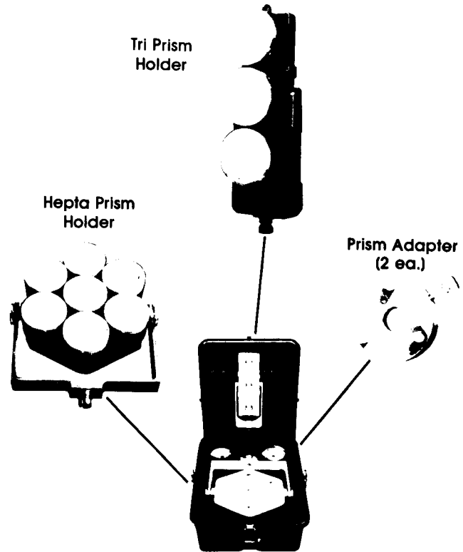
Figure 2 - Reflector Assembly
