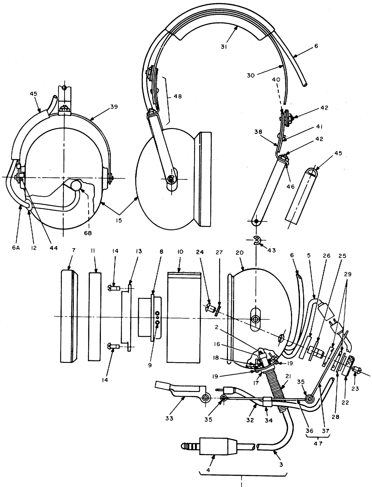
Figure D-1. Headset-Microphone 19LB-87.
