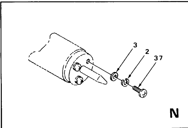
FIGURE 2. CONVERTER, ELECTRONIC FREQUENCY CV-3085/MSC-46(V) AND CV-3085/MSC-46(V) (SHEET 3 OF 3)
