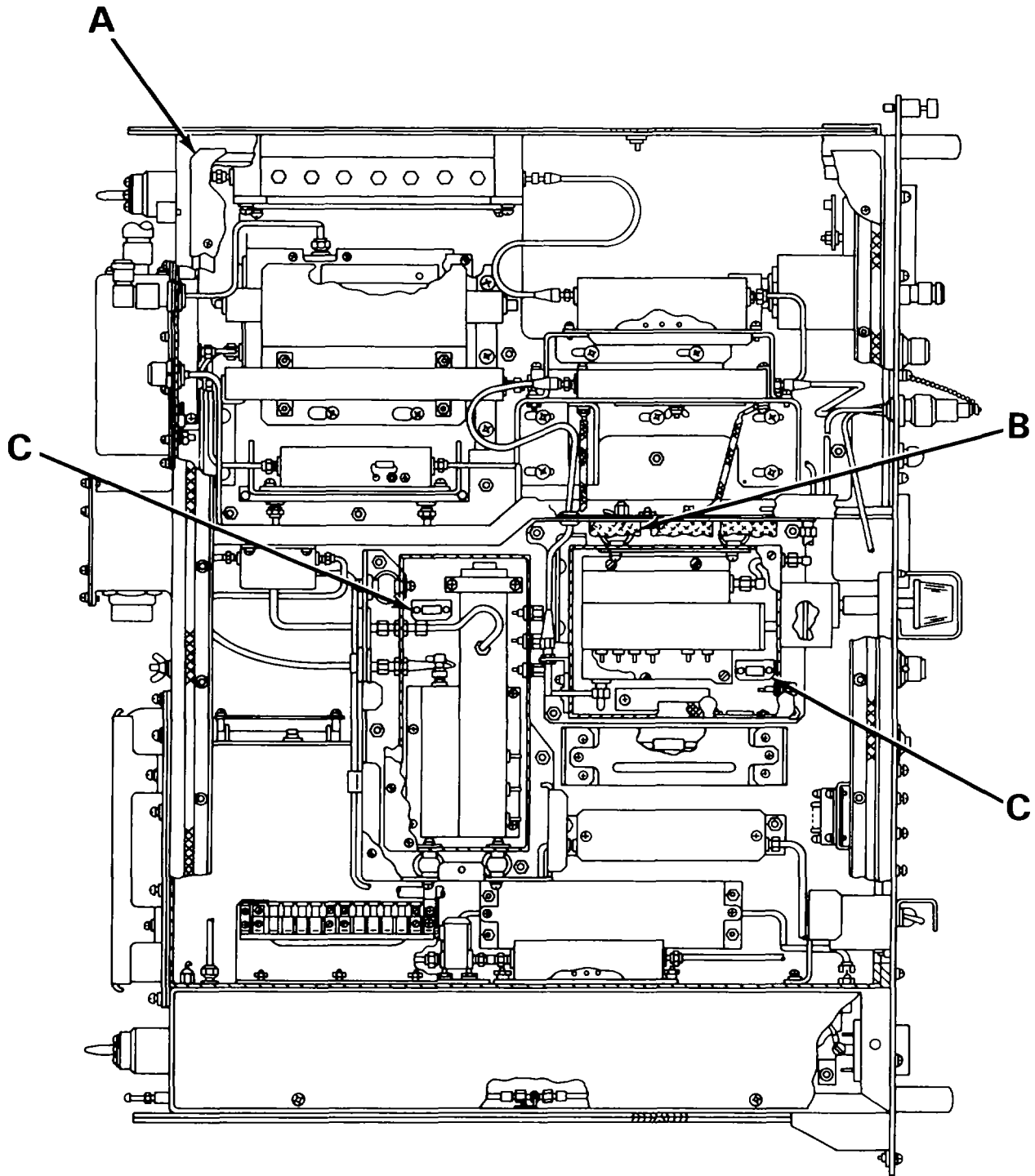
FIGURE 7. CONVERTER, ELECTRONIC FREQUENCY CV-3085/MSC-46(V) AND CV-3085A/MSC-46(V) (SHEET 1 OF 2)
