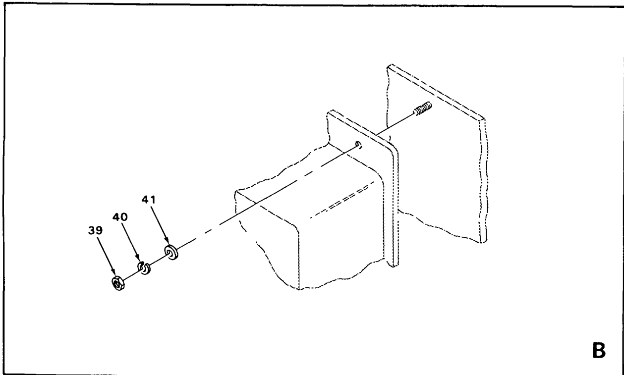
FIGURE 1 CONVERTER, ELECTRONIC FREQUENCY CV-3085/MSC-46(V) AND CV-3085A/MSC-46(V) (SHEET 2 OF 2)
