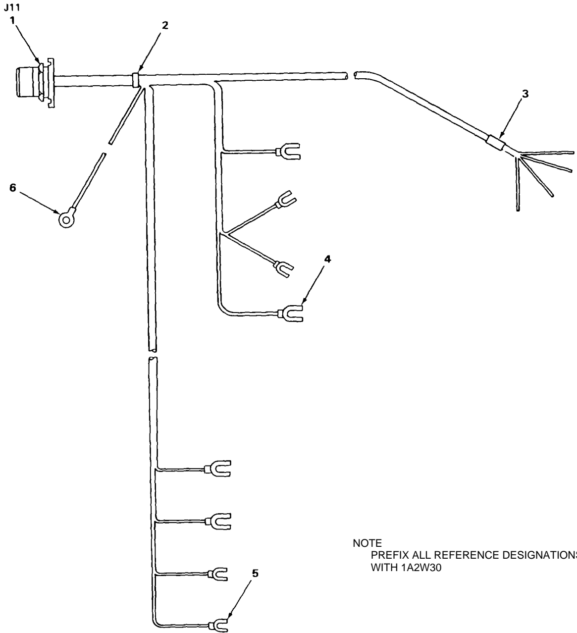
FIGURE 15. WIRING HARNESS, AC PRIME POWER (1A2W30)
