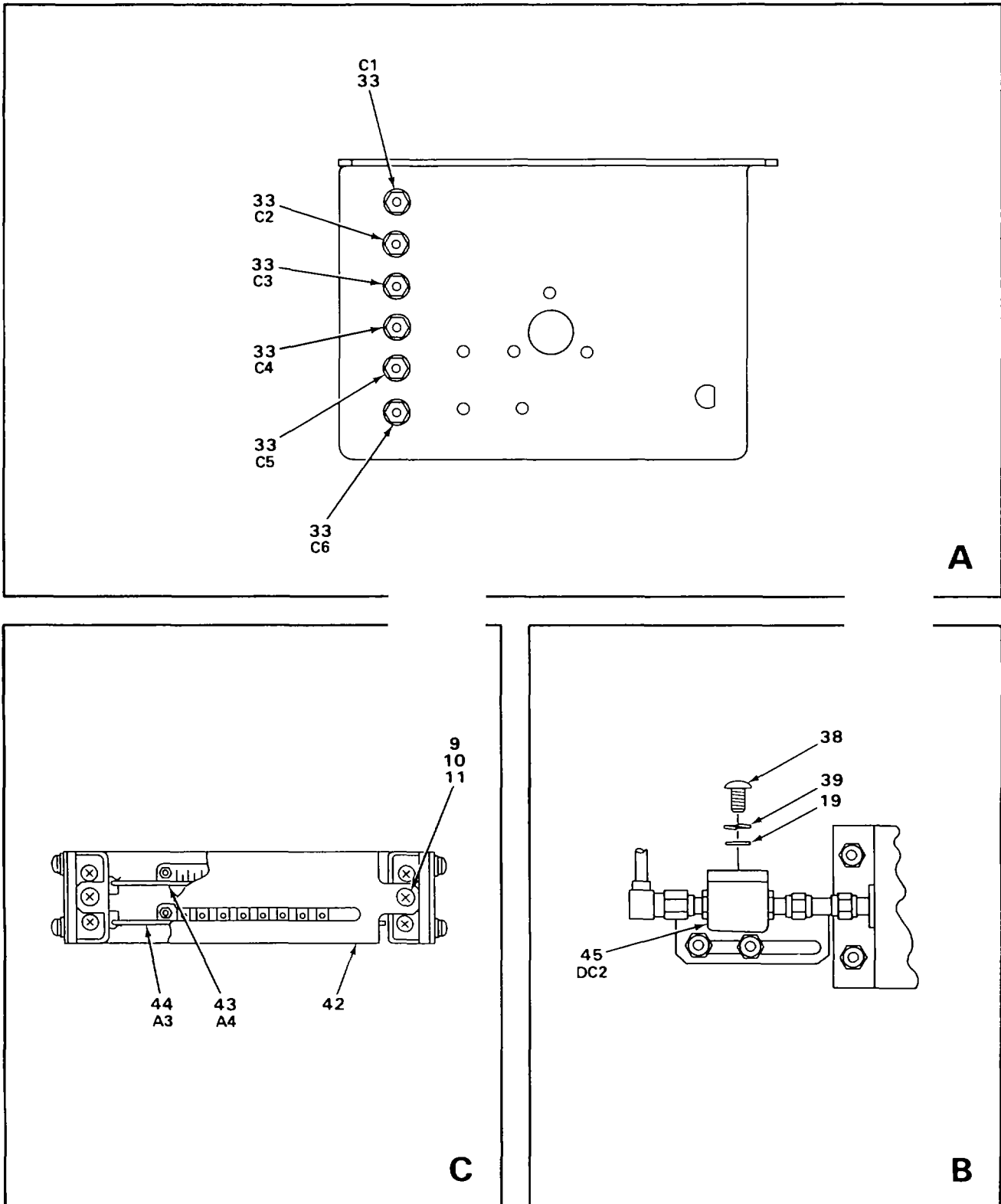
FIGURE 4. CONVERTER, ELECTRONIC FREQUENCY CV-3085/MSC-46(V) AND CV-3085A/MSC-46(V) (SHEET 2 OF 2)
