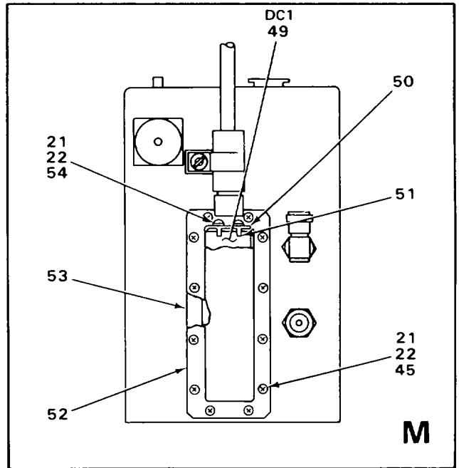
FIGURE 2. CONVERTER, ELECTRONIC FREQUENCY CV-3085/MSC-46(V) AND CV-3085/MSC-46(V) (SHEET 3 OF 3)
