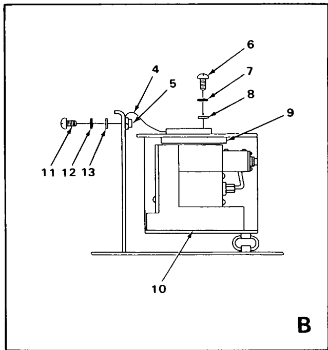
FIGURE 7. CONVERTER, ELECTRONIC FREQUENCY CV-3085/MSC-46(V) AND CV-3085A/MSC-46(V) (SHEET 2 OF 2)
