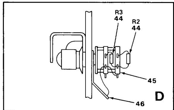
FIGURE 21. FRONT PANEL ASSEMBLY (1A2A2)
