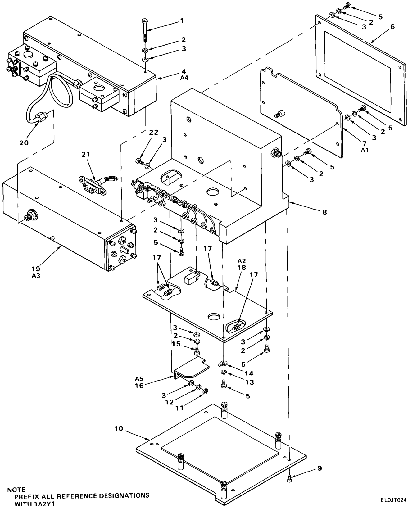
FIGURE 26. RF PHASE-LOCKED OSCILLATOR (1A2Y1)
