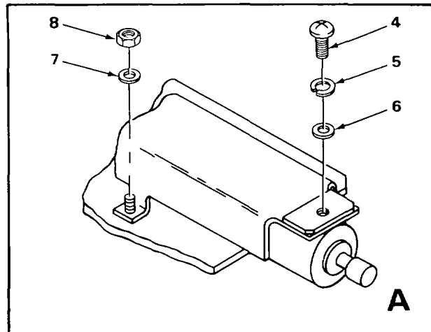
FIGURE 19. BANDPASS FILTER ASSEMBLY (1A2A7)
