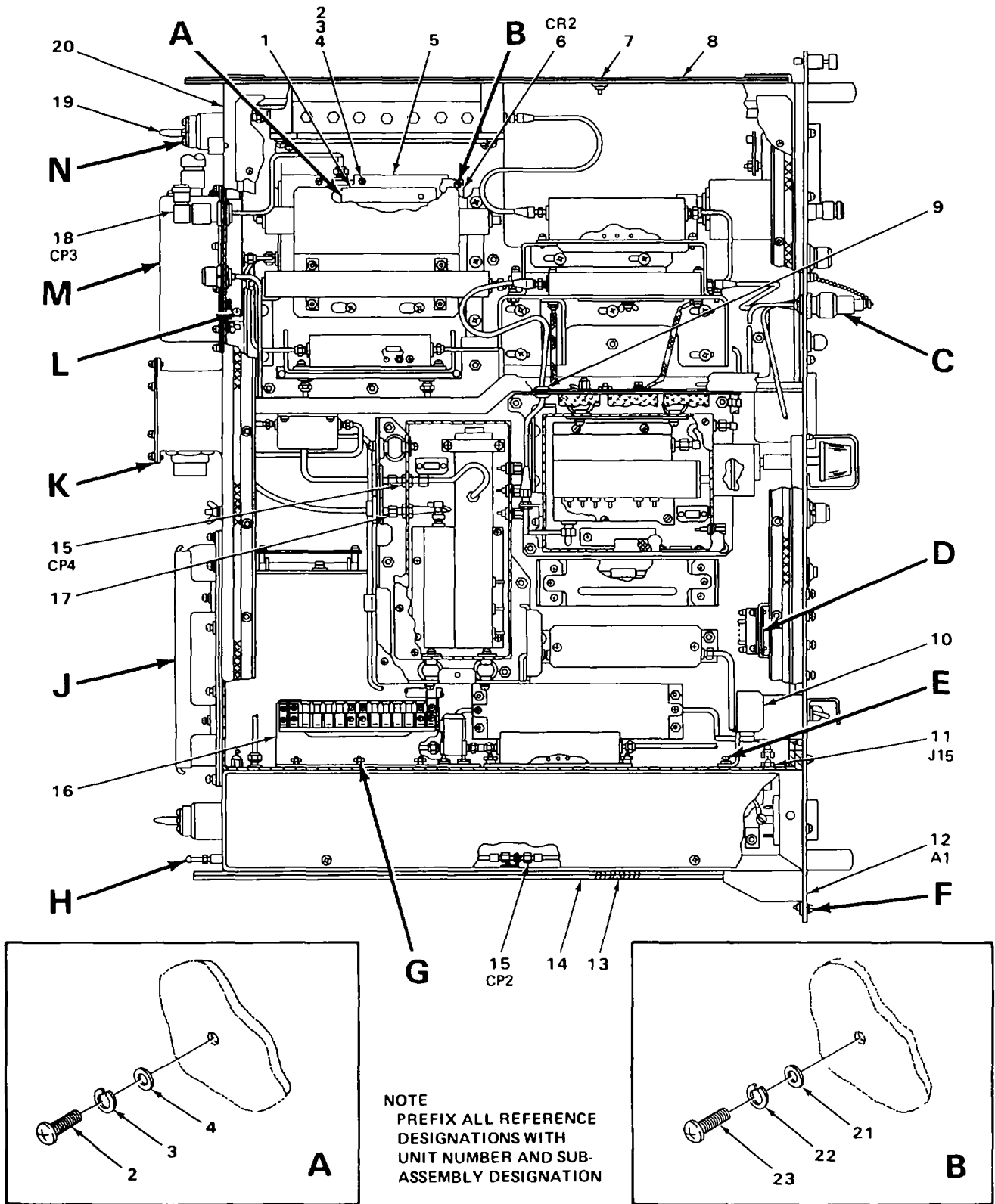
FIGURE 2. CONVERTER, ELECTRONIC FREQUENCY CV-3085/MSC-46(V) AND CV-3085A/MSC-46(V) (SHEET 1 OF 3)
