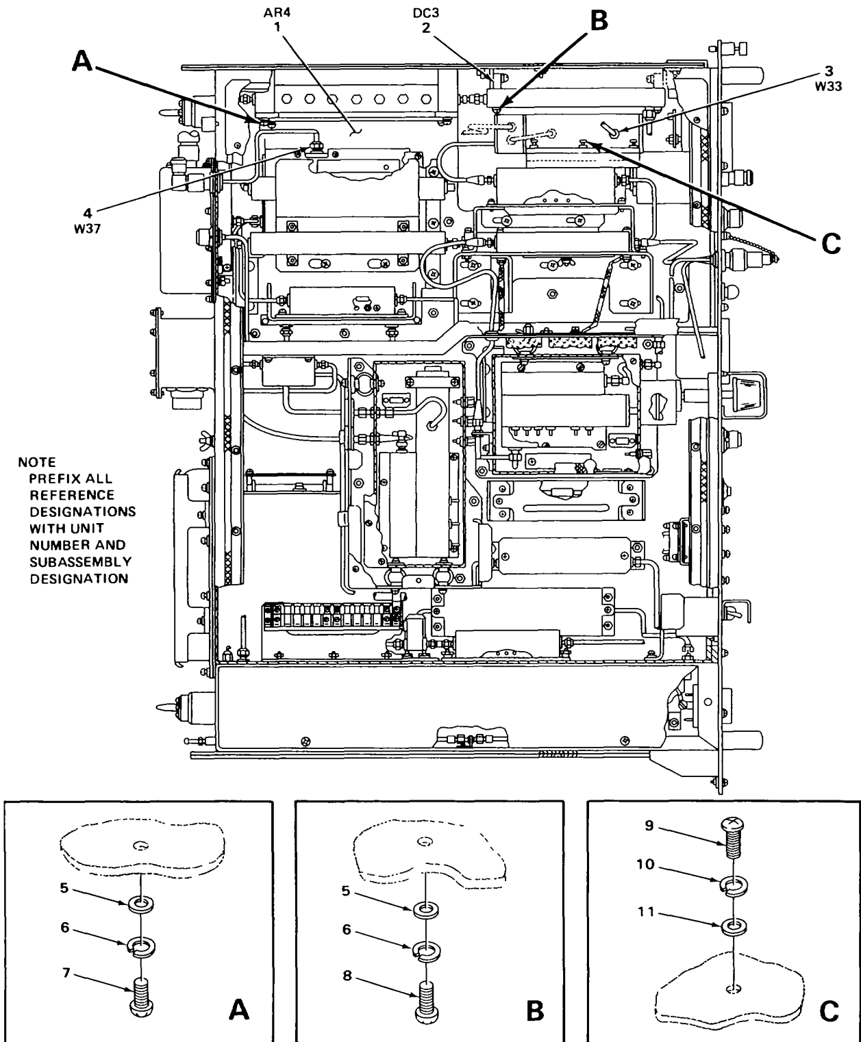
FIGURE 3. CONVERTER, ELECTRONIC FREQUENCY CV-3085/MSC-46(V) AND CV-3085/MSC-46(V)
