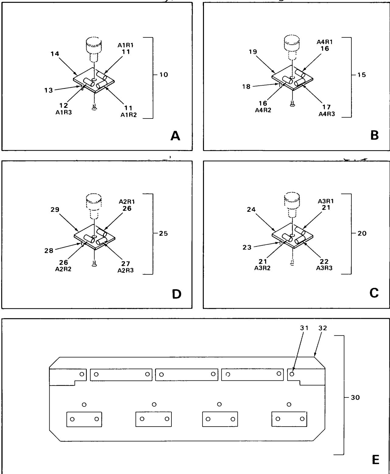
FIGURE 16. AMPLITUDE STEP ATTENUATOR (1A2AT5) (SHEET 2 OF 2)
