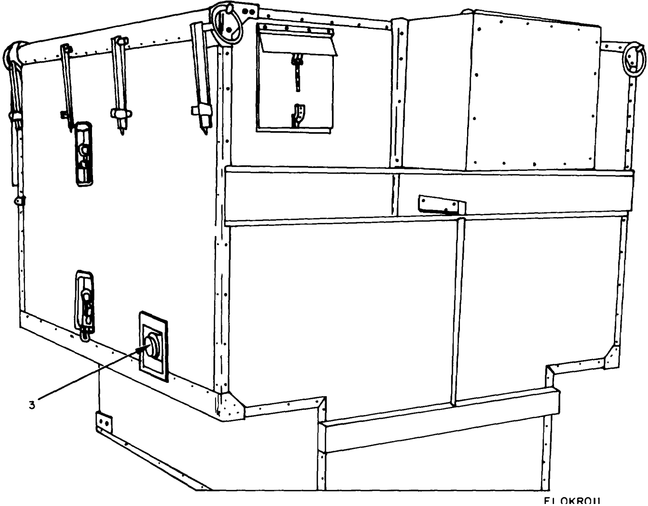
Figure 4. Shelter, Electrical Equipment, Front Door View (Sheet 2 of 2).
