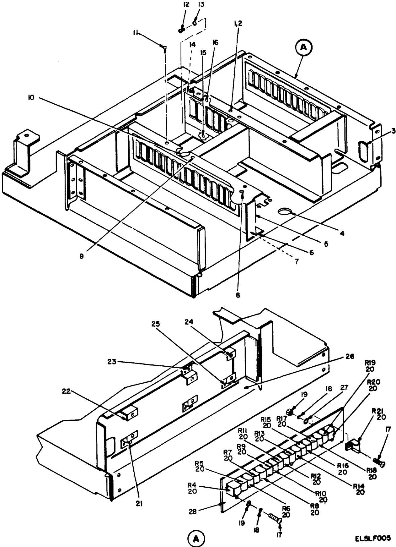
Figure 4. Signal Processor CP-925/TPX-46(V)(1A3), Chassis Top View.
