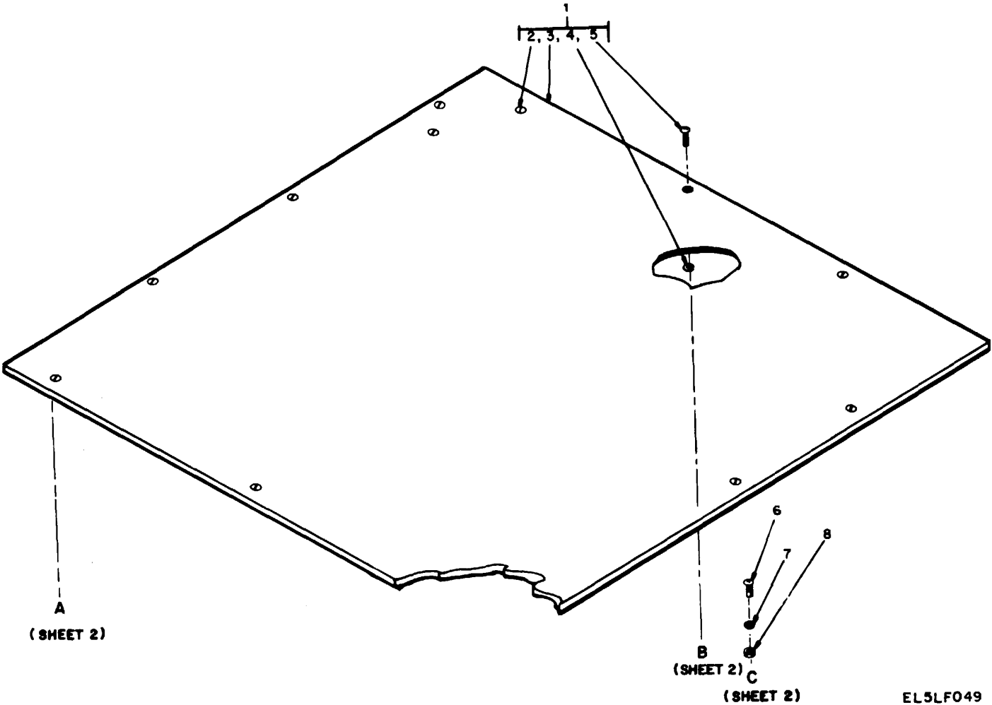
Figure 2. Signal Processor CP-925/TPX-46(V)(1A3), Bottom View. (Sheet 1 of 2).
