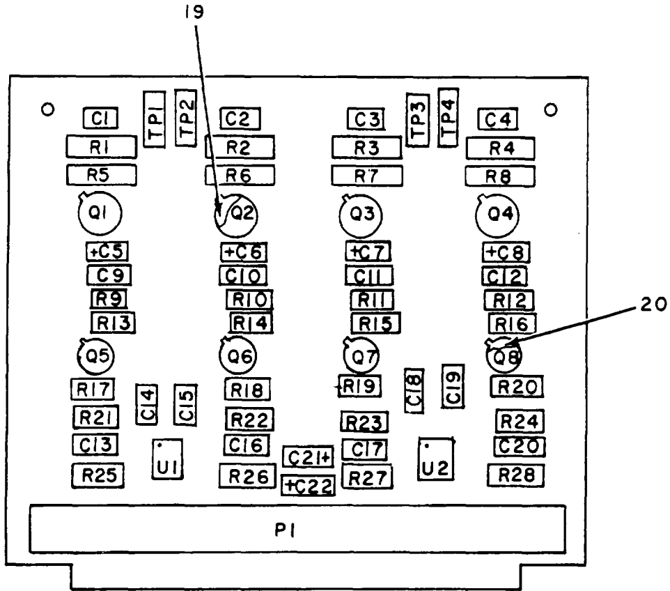
Figure 35. Read-Write Drivers (4) Circuit Card (1A3A34 thru 1A3A37) (Sheet 1 of 2).
