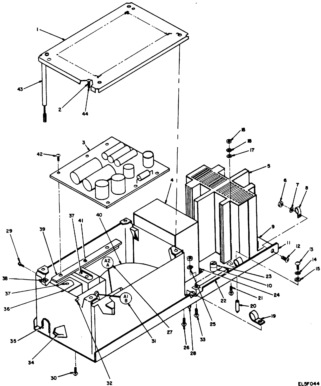
Figure 36. Power Supply (1A3A39). (Sheet 1 of 2).
