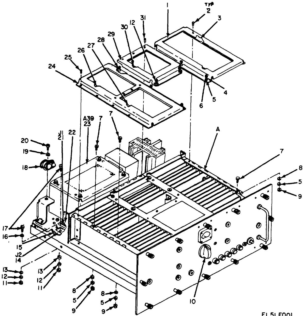
Figure 1. Signal Processor CP-925/TPX-46(V), Top View (1A3). (Sheet 1 of 2).
