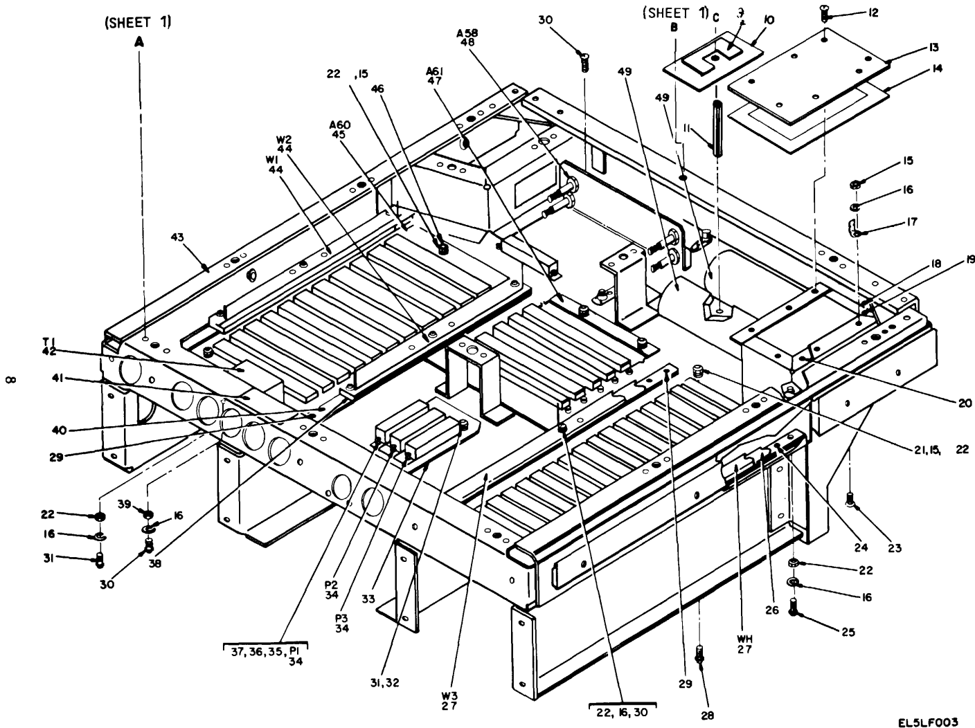
Figure 2. Signal Processor CP-925/TPX-46(V)(1A3), Bottom View (Sheet 2 of ?).
