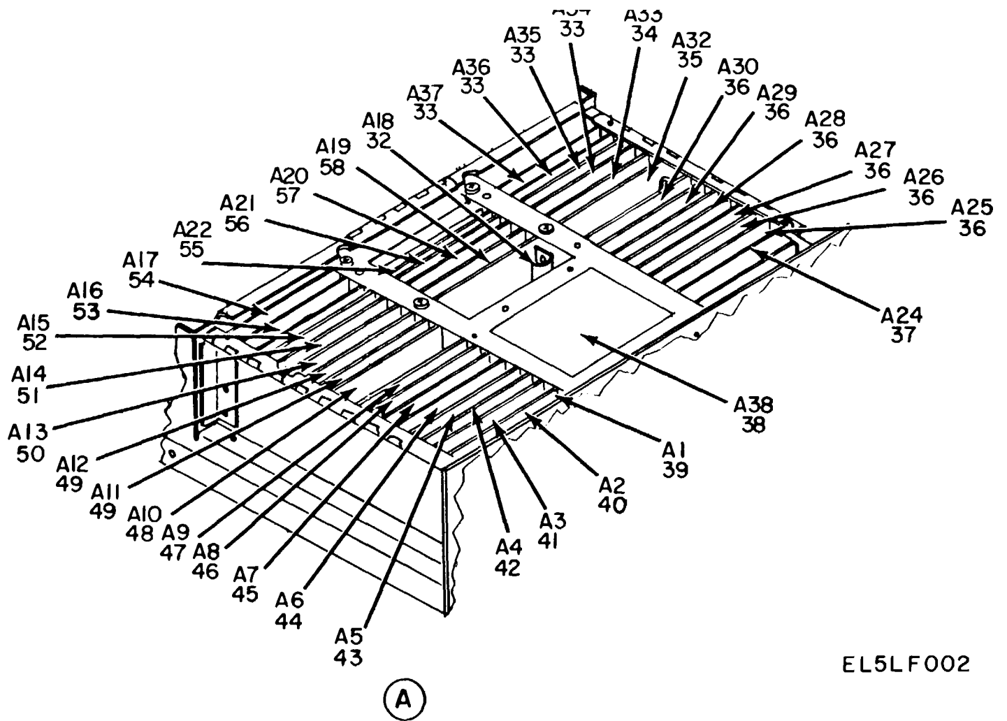
Figure 1. Signal Processor CP-925/TPX-46(V), Top View (1A3) (Sheet 2 of 2)
