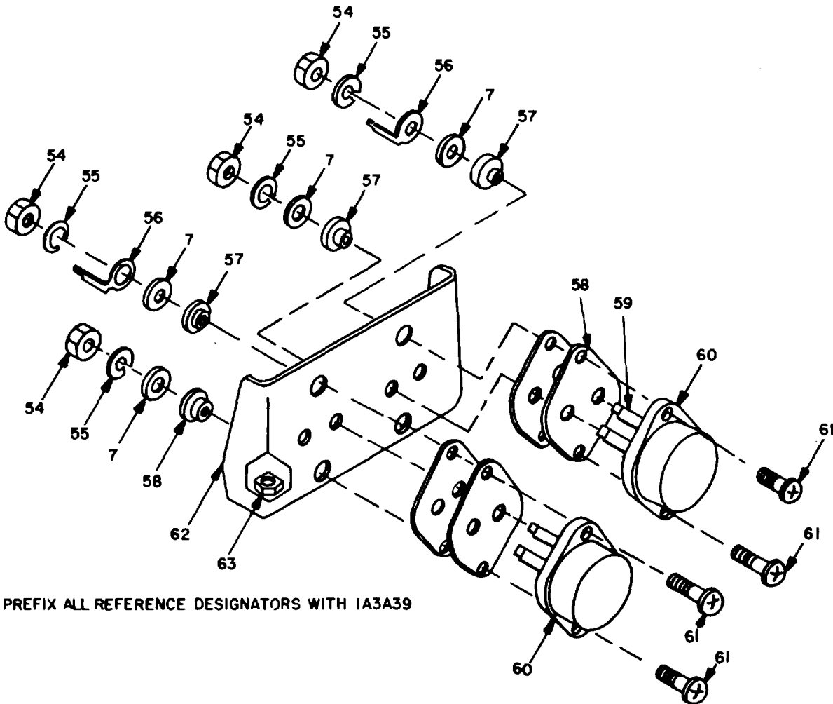
Figure 36. Power Supply (1A3A39).(Sheet 2 of 2).
