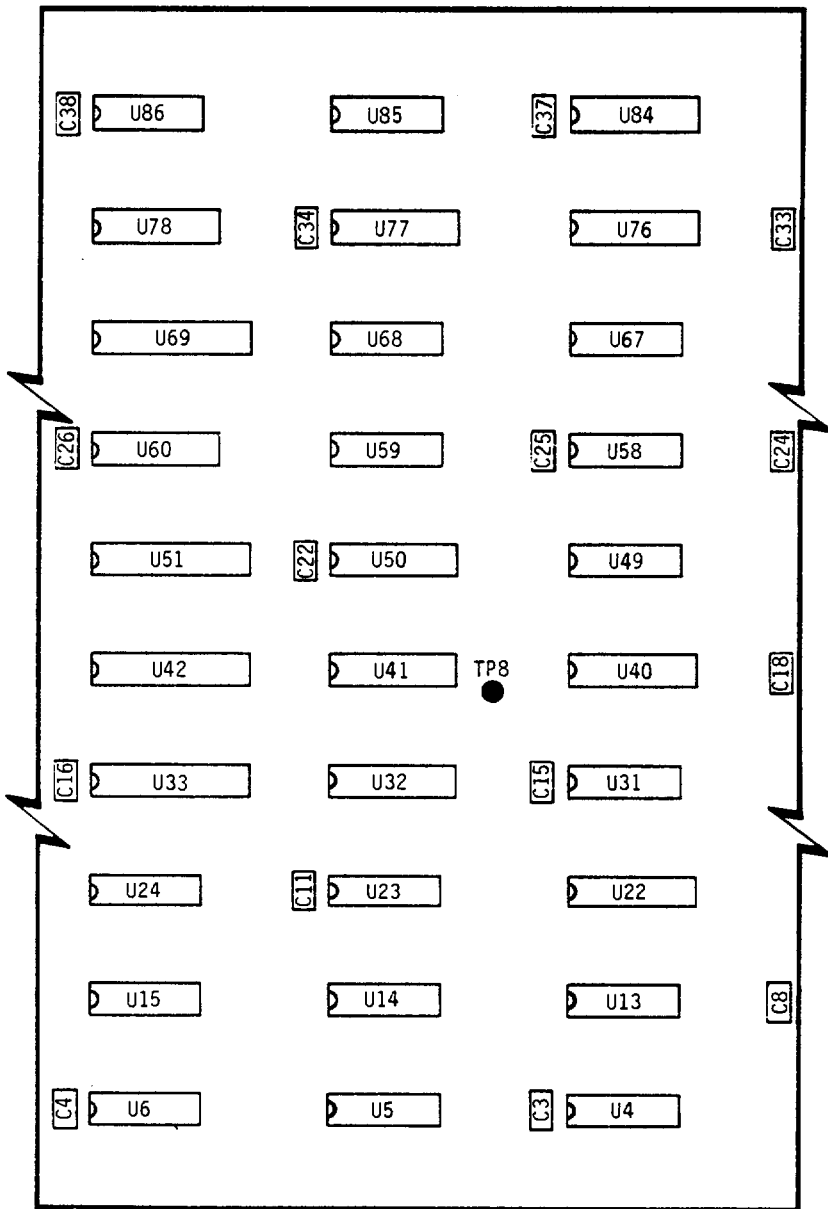
Figure 3. Circuit Card Assembly, Interleaver (A2) (Sheet 3 of 4)
