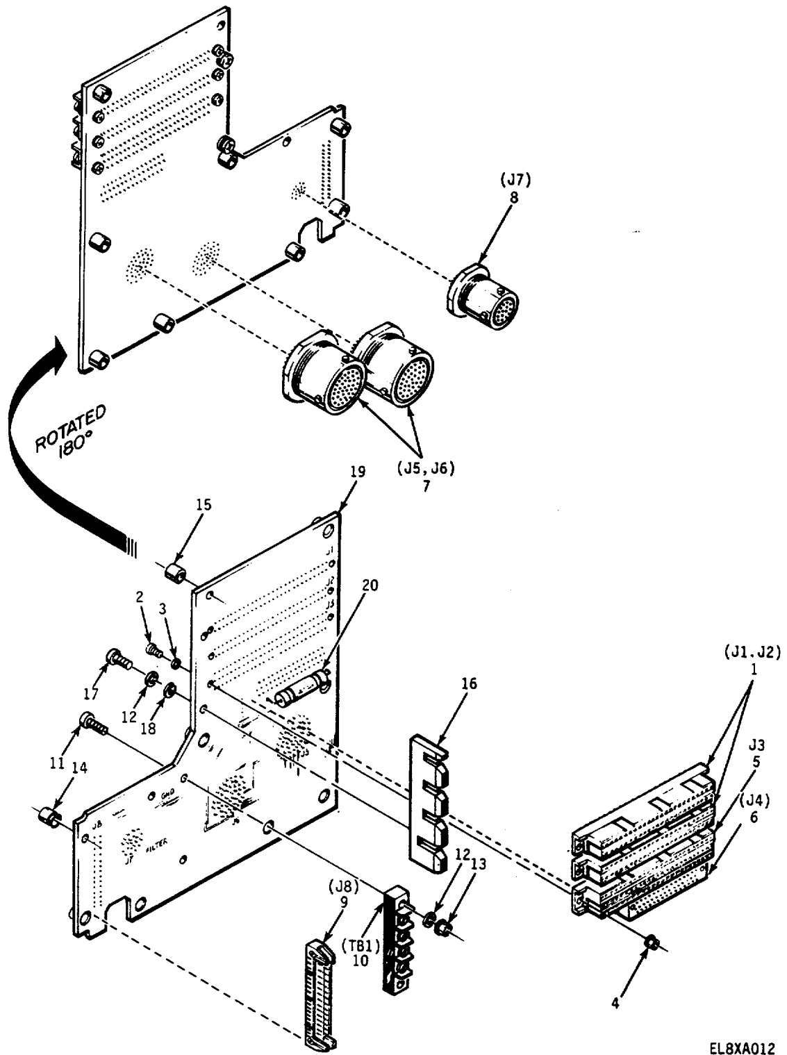
Figure 12. Circuit Card Assembly, Backplane (A5A1)
