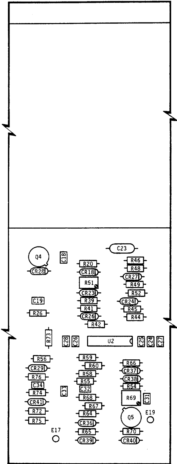
Figure 5. Circuit Card Assembly, Power Supply (A4) (Sheet 4 of 5)
