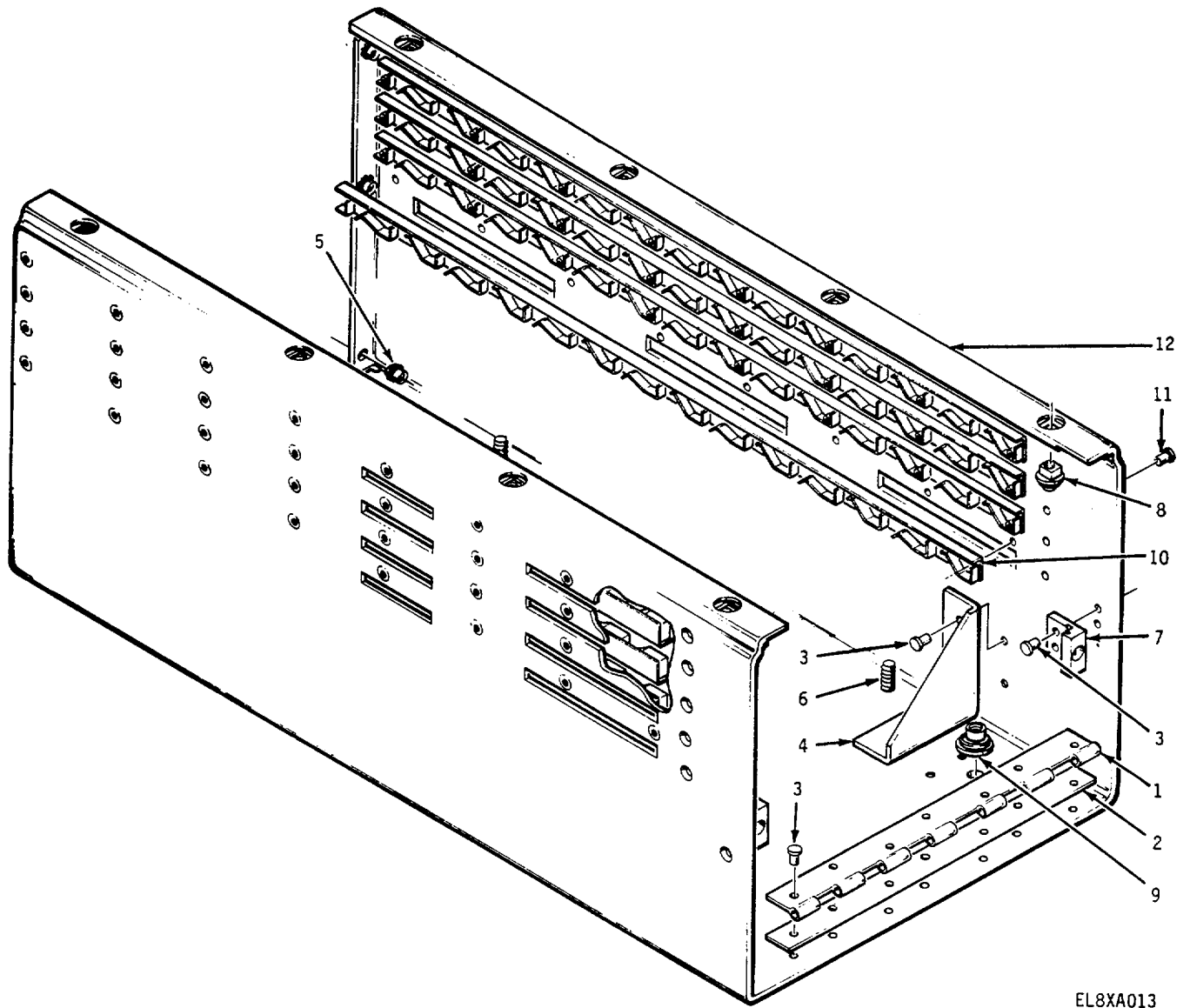
Figure 13. Chassis, Sub-Assembly (A8A1)
