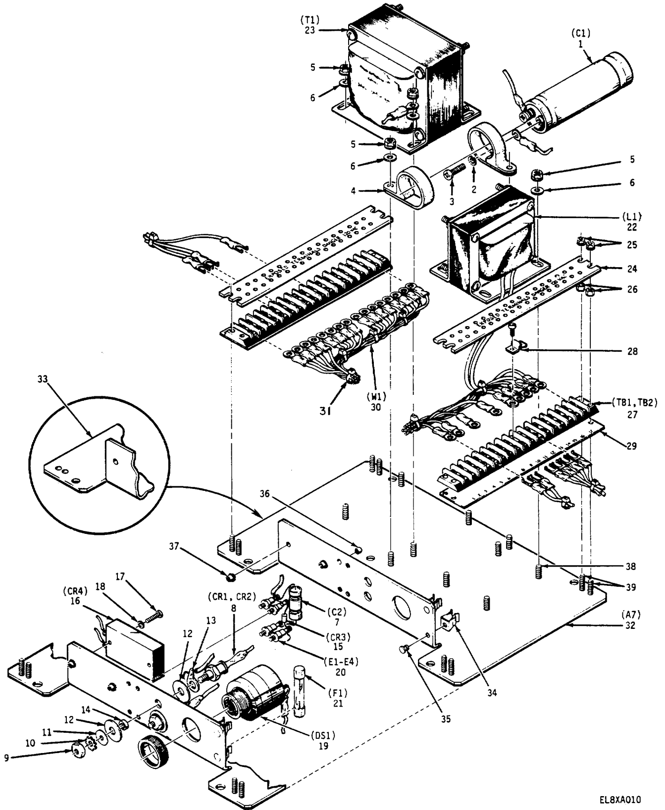
Figure 10. Bottom Panel Assembly (A7)
