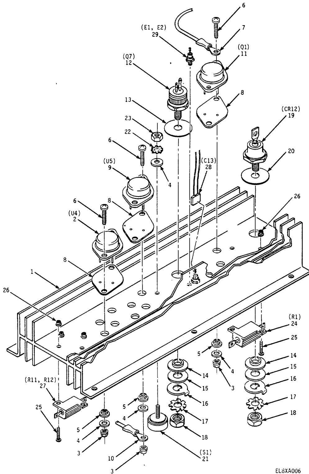
Figure 6. Heat Sink Assembly (A4A1)
