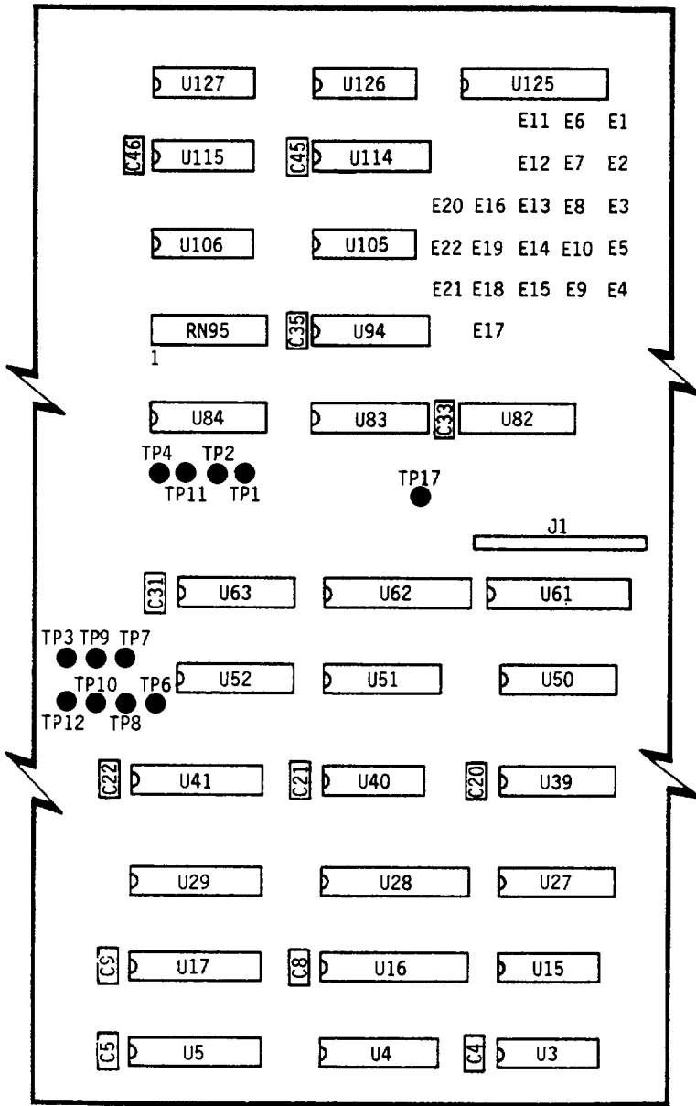
Figure 4. Circuit Card Assembly, Input/Output (A3) (Sheet 4 of 5)
