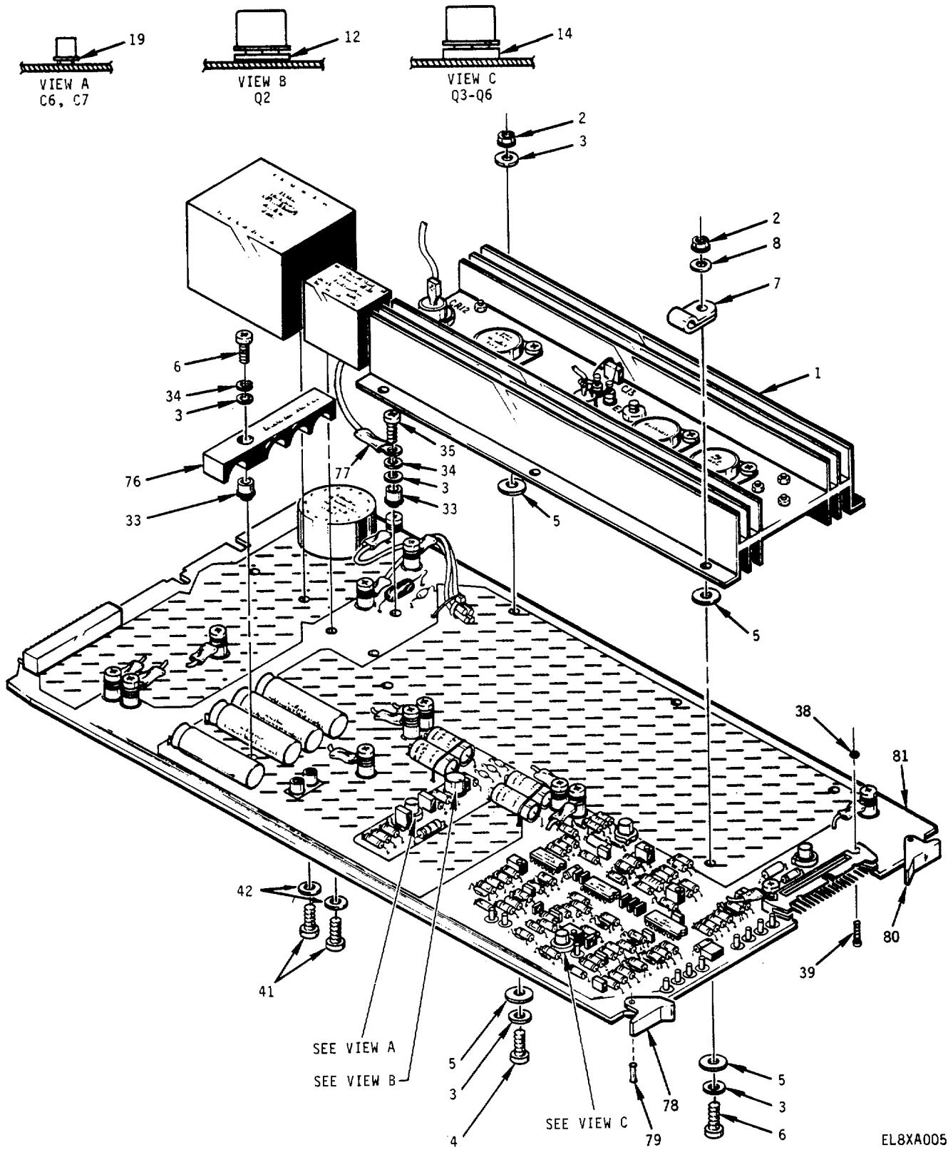
Figure 5. Circuit Card Assembly, Power Supply (A4) (Sheet 1 of 5)
