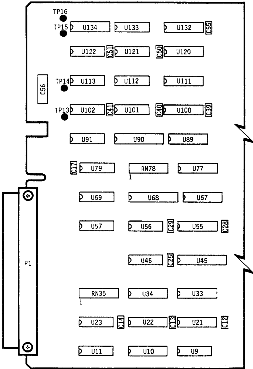
Figure 4. Circuit Card Assembly, Input/Output (A3) (Sheet 2 of 5)
