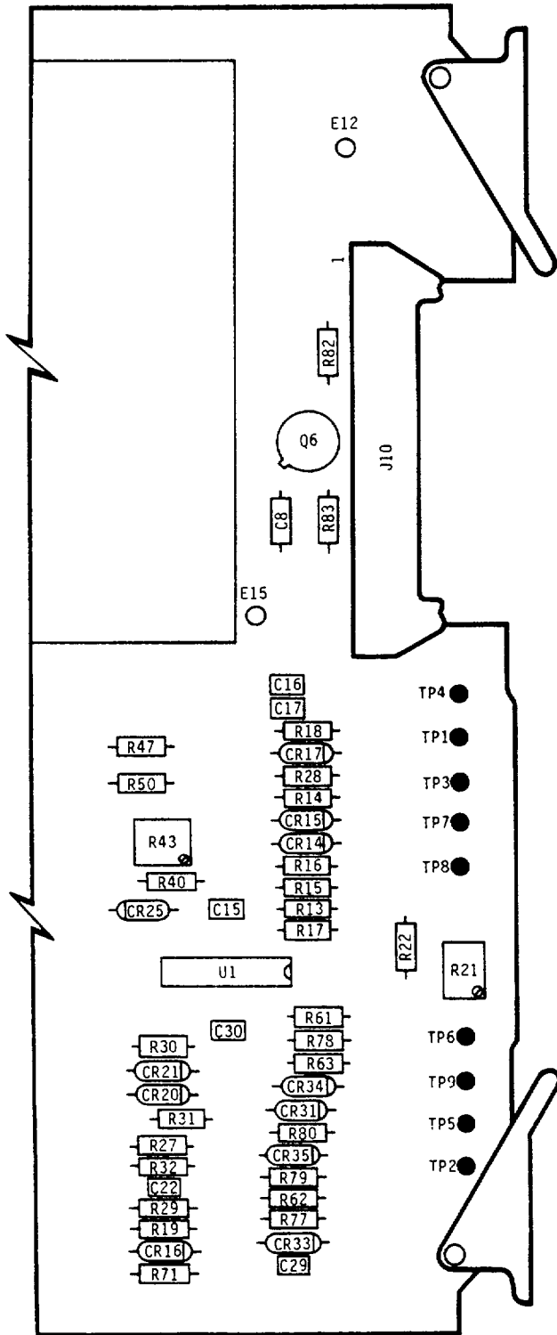
Figure 5. Circuit Card Assembly, Power Supply (A4) (Sheet 5 of 5)
