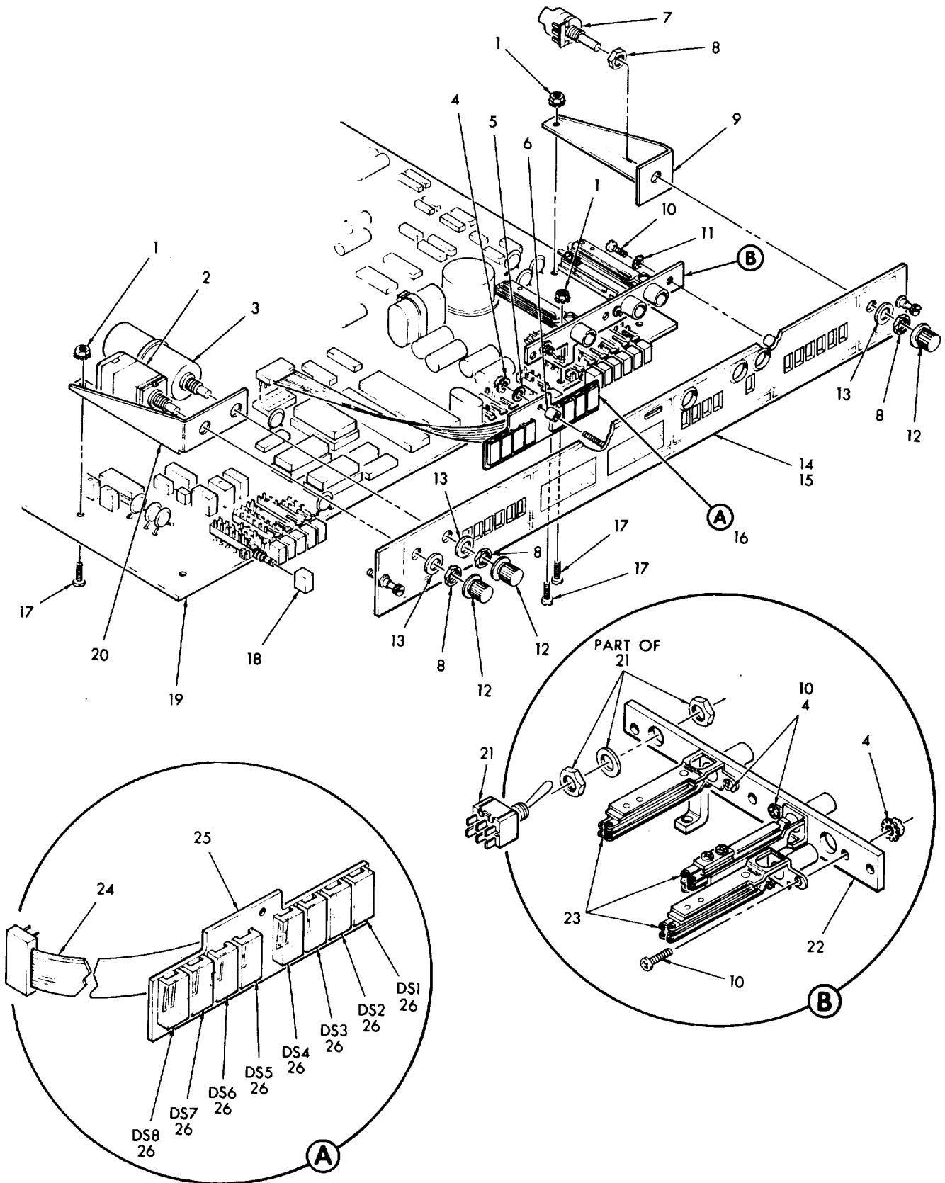
Figure 3. Panel Assembly, Front, P1122-002-02
