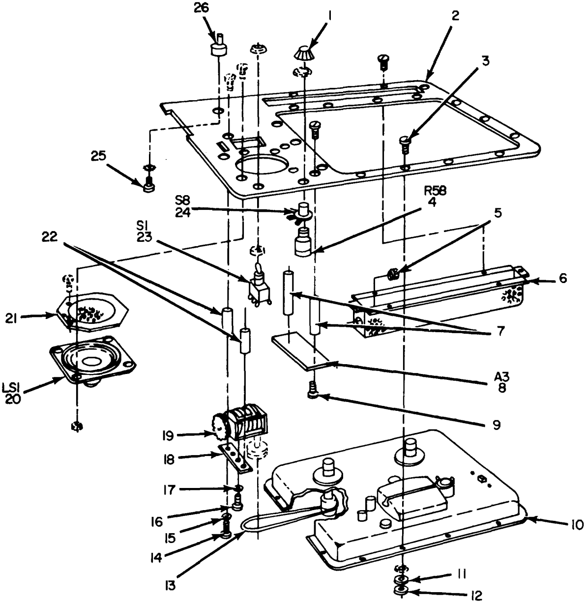
Figure 4. Recorder Reproducer Set, Sound AN/UNH-10, Panel Assembly, Main.
