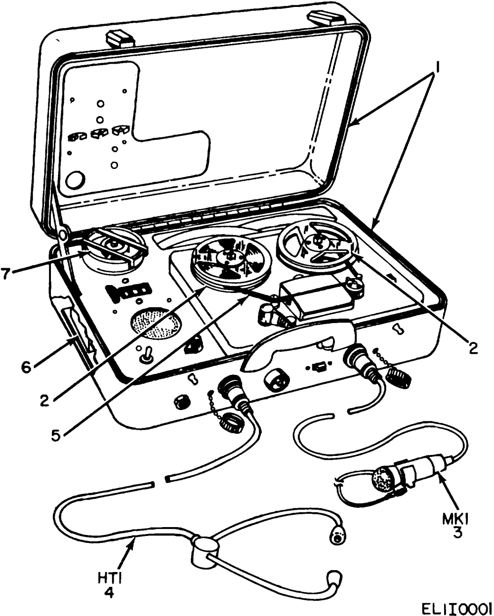
Figure 1. Recorder Reproducer Set, Sound AN/UNH-10.
