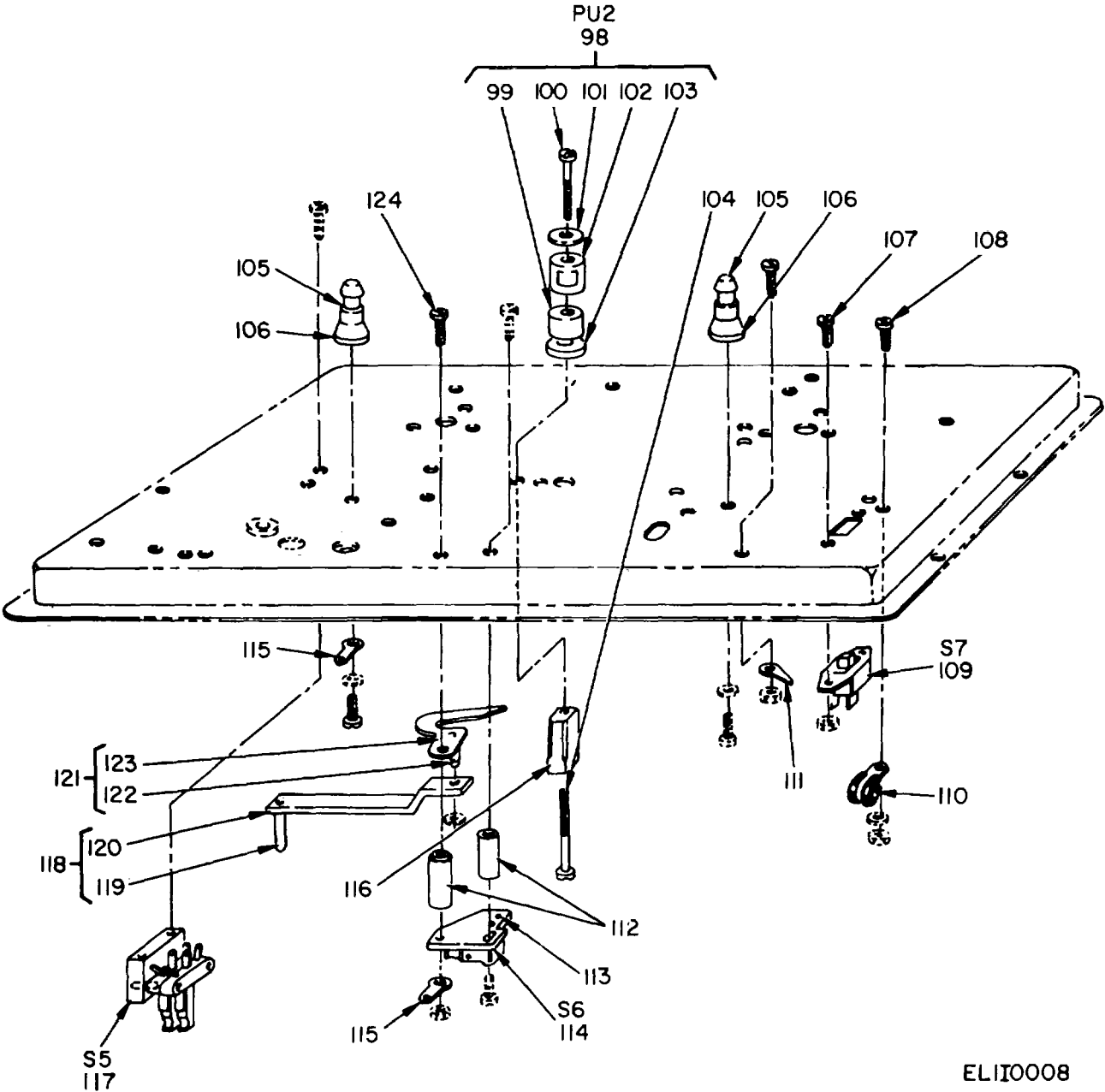
Figure 6. Recorder Reproducer Set, Sound AN//UNH-10,, Transport, Magnetic Tape (Sheet 3 of 3).
