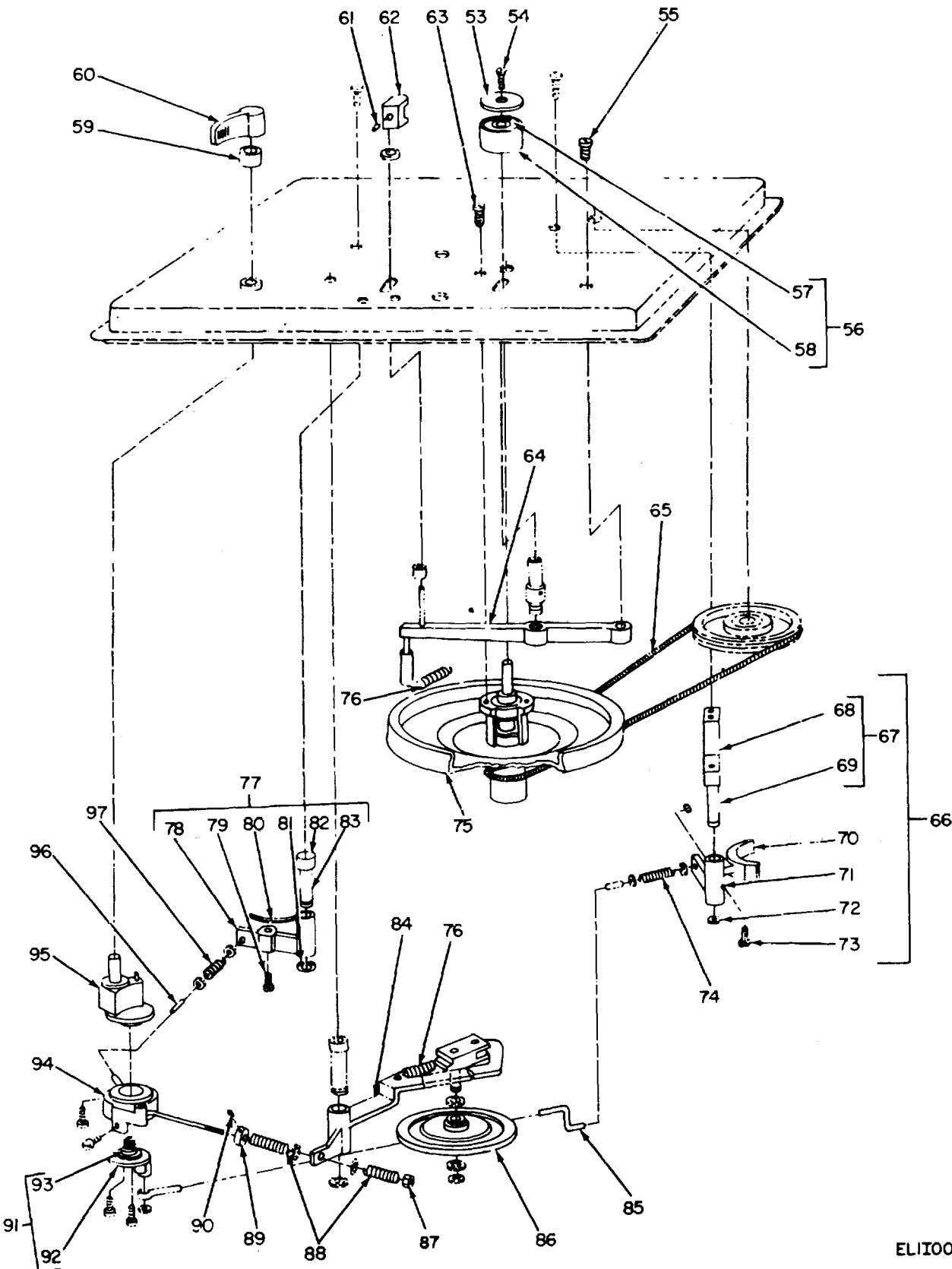
Figure 6. Recorder Reporducer Set, Sound AN/UNH-10, Transport, Magnetic Tape (Sheet 2 of 3)
