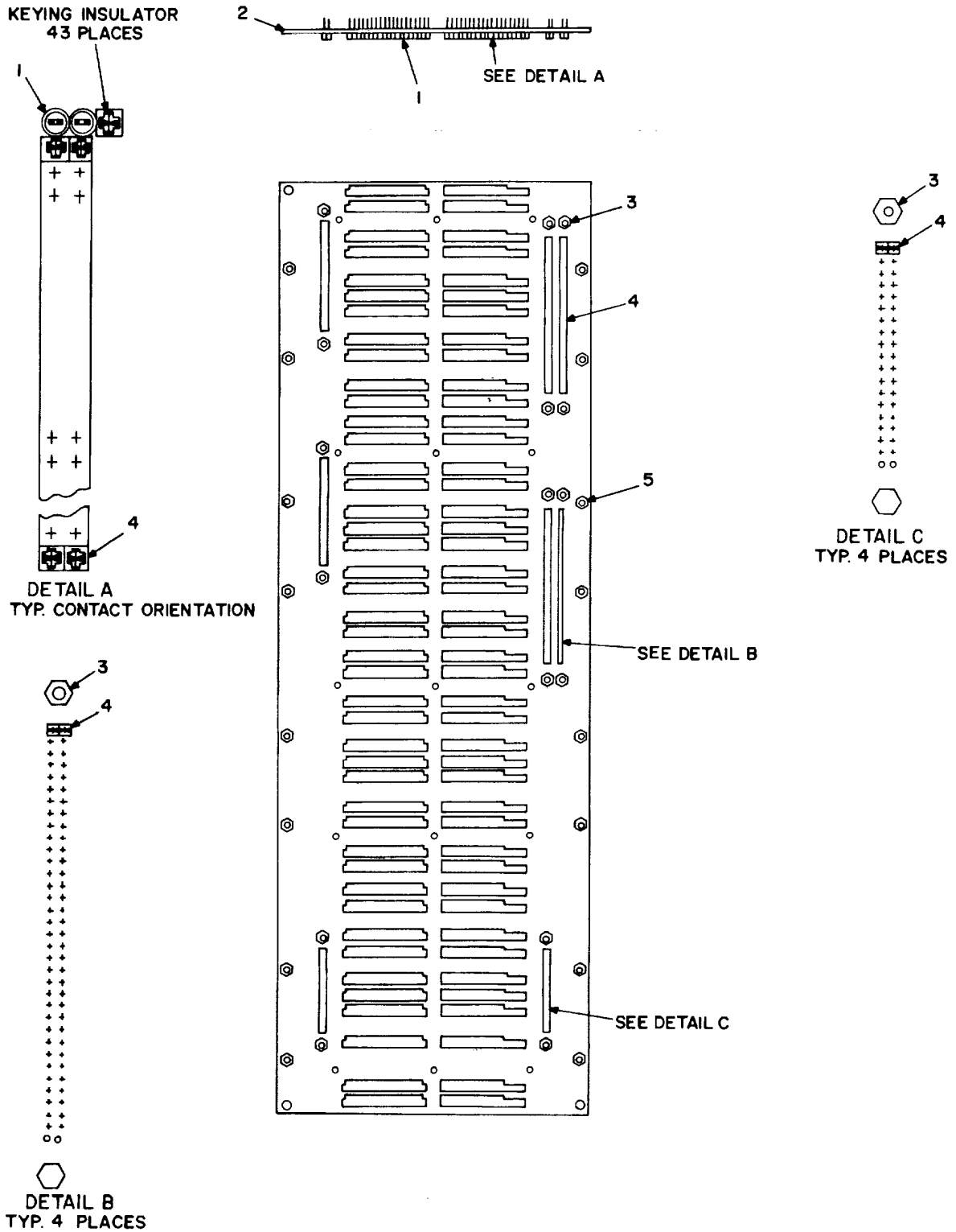
Figure 19. Connector plate assy, SM-D-814619.
