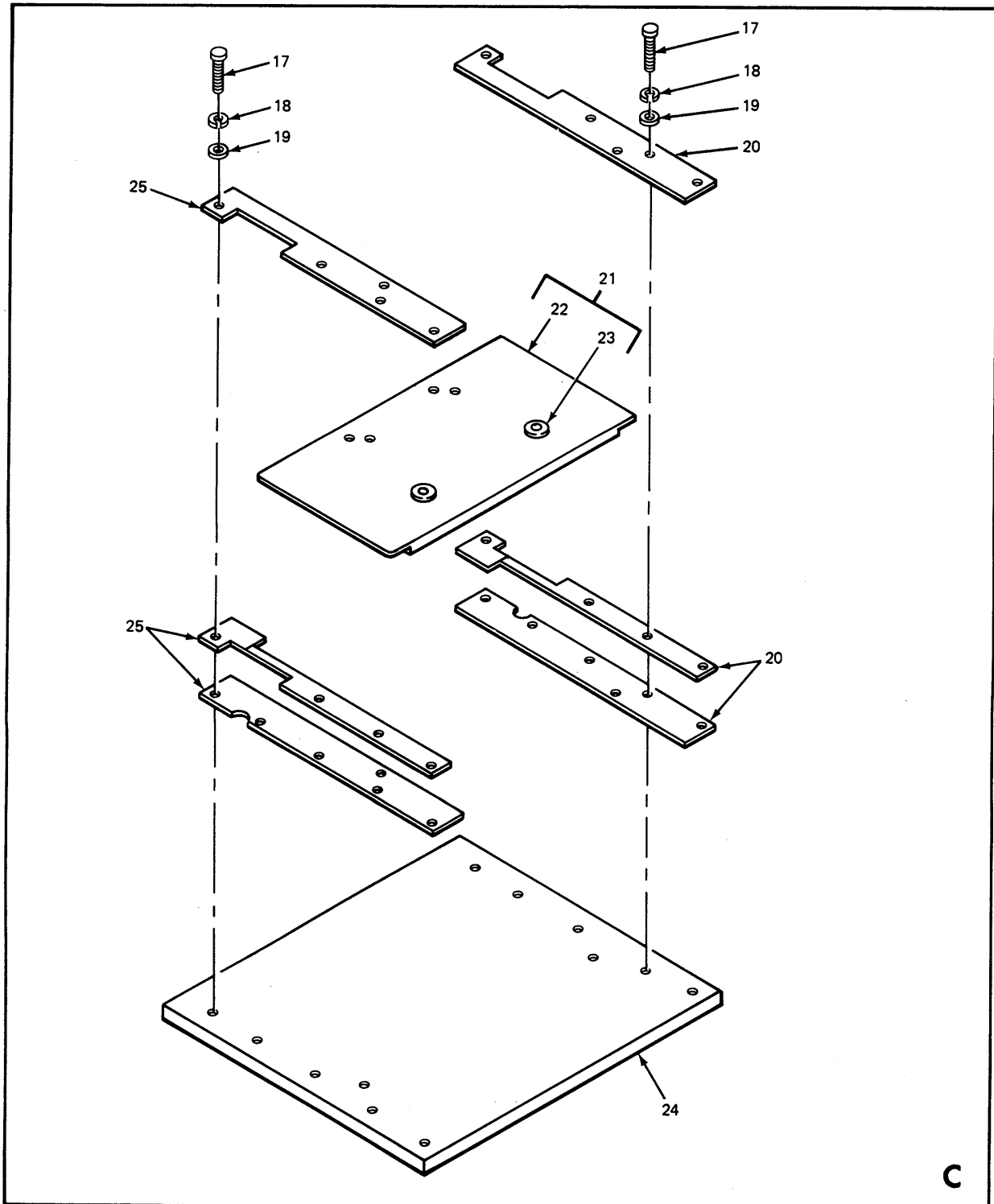
Figure 2. Shelter, Modified S-348A/TSC-58A, Curbside (Sheet 2 of 2).
