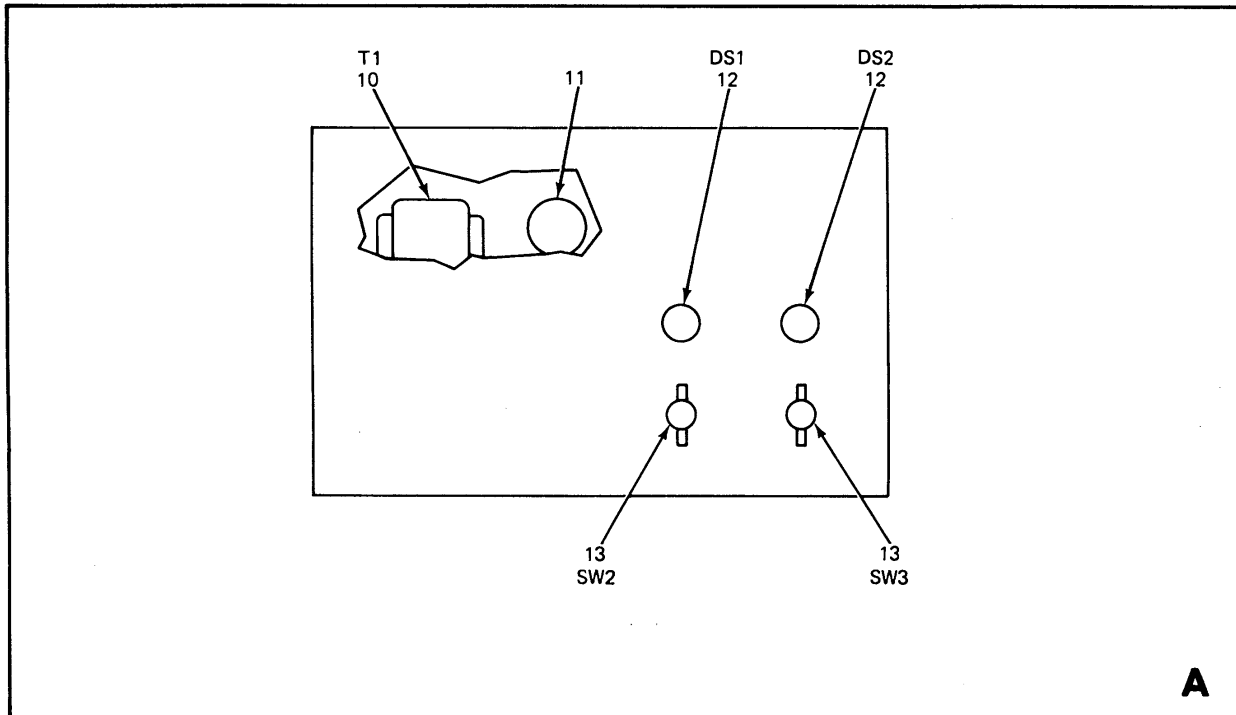
Figure 5. Shelter, Electrical Equipment S-348/TSC-58 and S-348A/TSC-58A, Curbside Wall.
