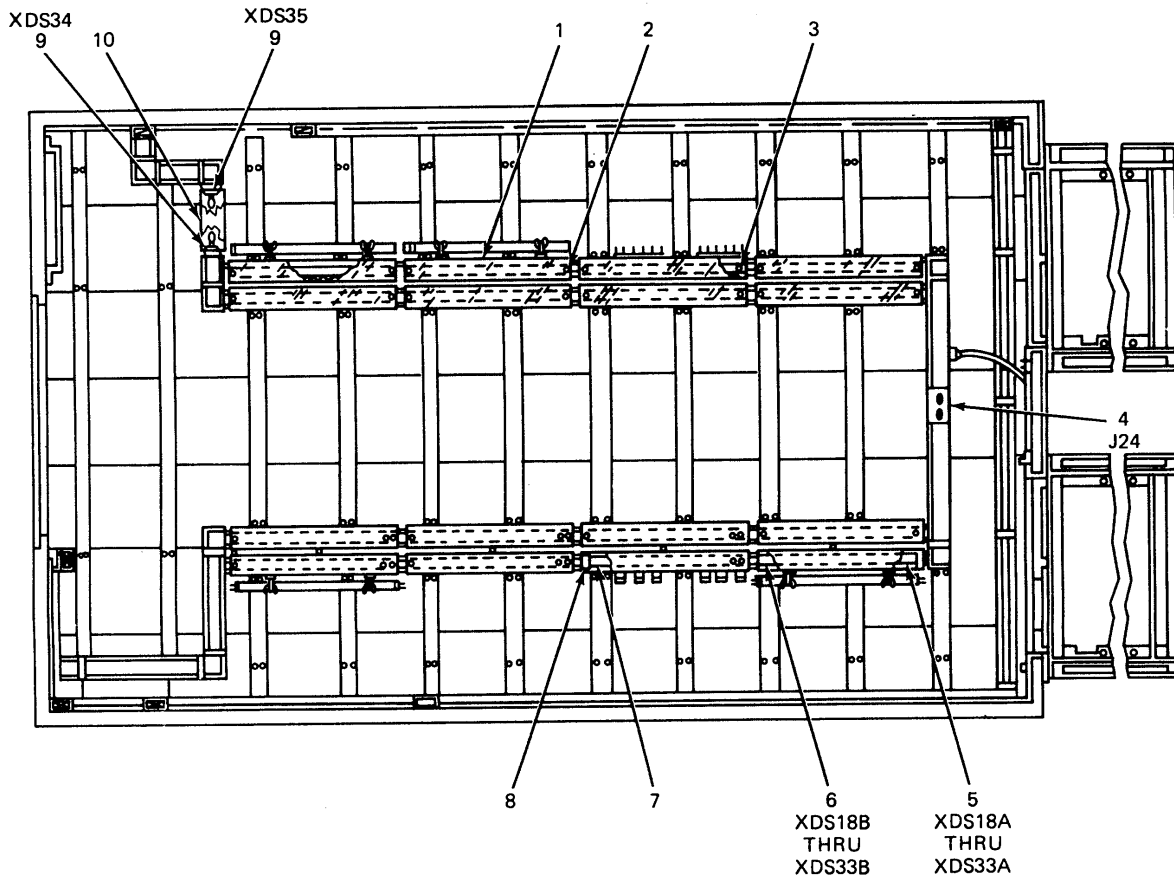
Figure 9. Shelter, Electrical Equipment S-348/TSC-58 and S-348A/TSC-58A, Ceiling Plan.
