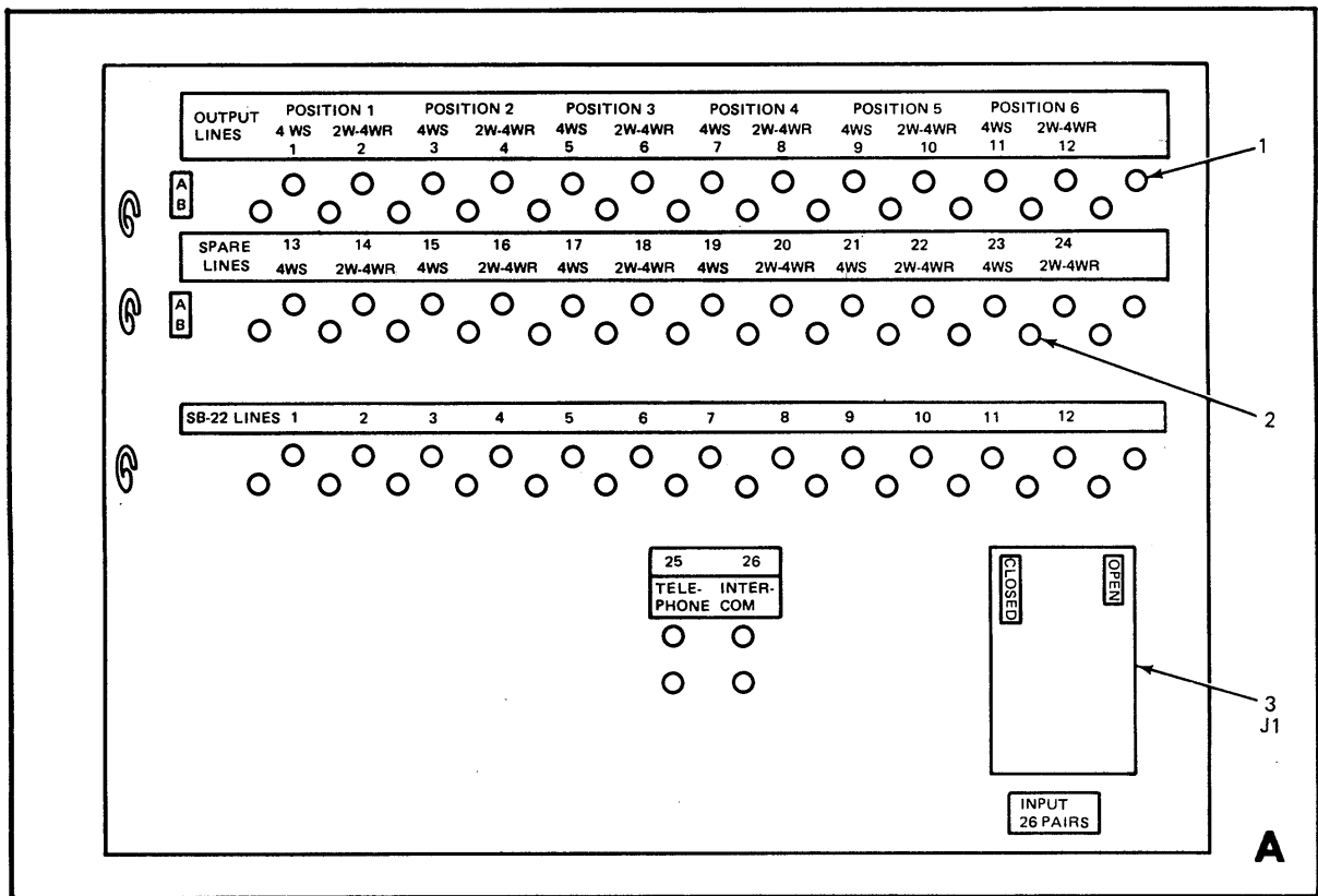
Figure 13. Shelter, Electrical Equipment S-348/TSC-58 and S-348A/TSC-58A, Signal Entrance Box.
