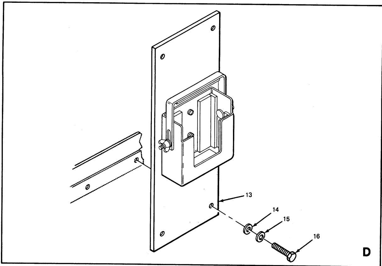
Figure 3. Shelter, Modified S-348A/TSC-58A, Roadside (Sheet 2 of 2).
