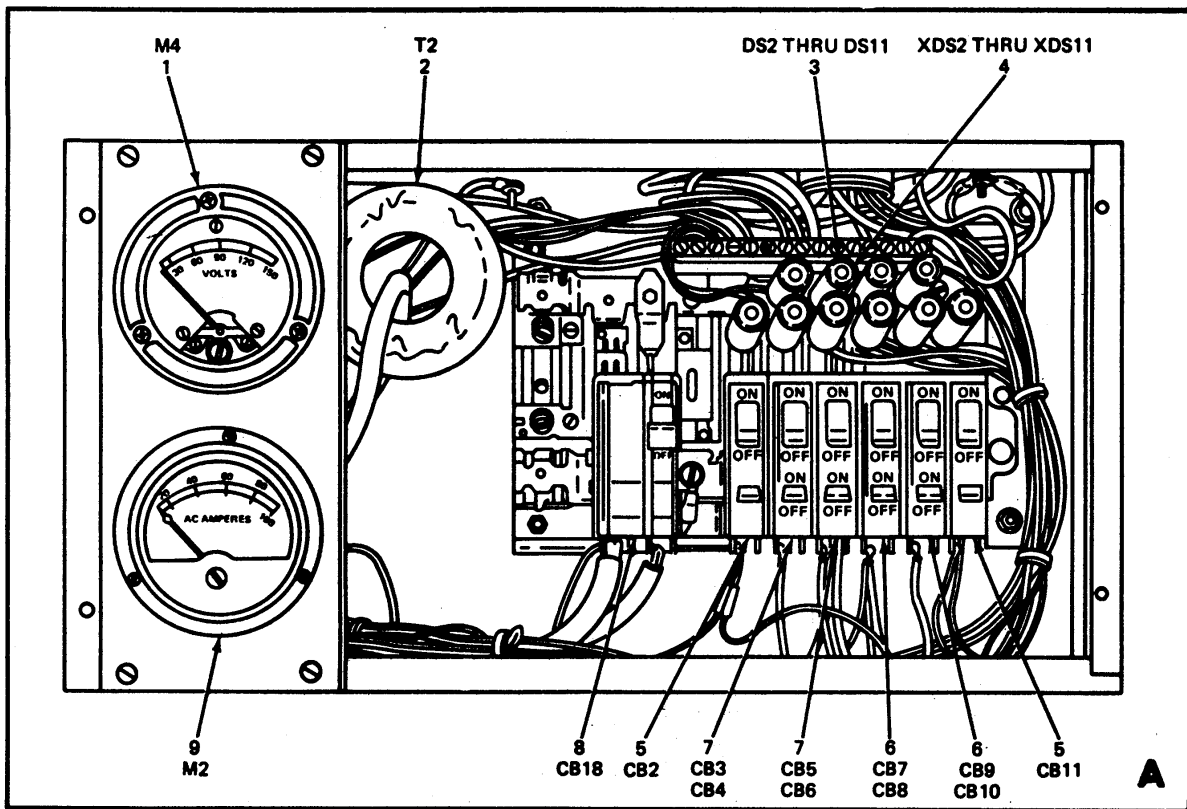
Figure 14. Shelter, Electrical Equipment S-348/TSC-58 and S-348A/TSC-58A, Block Power Distribution Panel.
