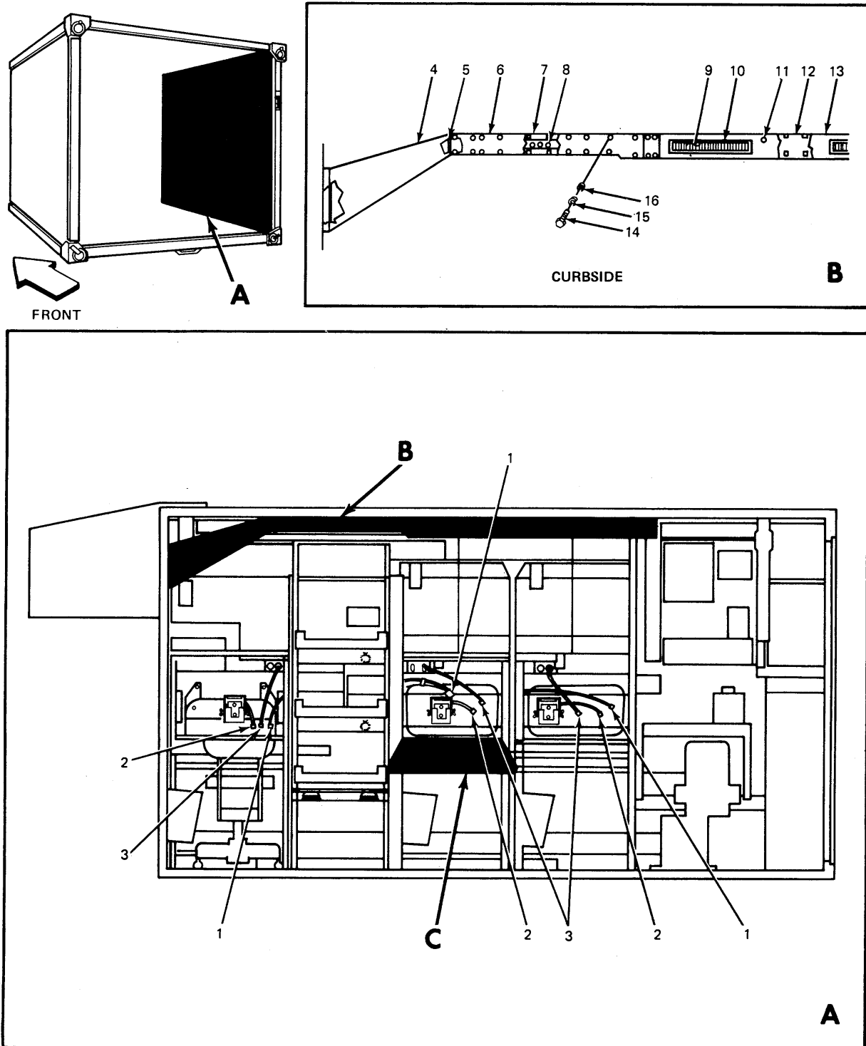
Figure 2. Shelter, Modified S-348A/TSC-58A, Curbside (Sheet 1 of 2).
