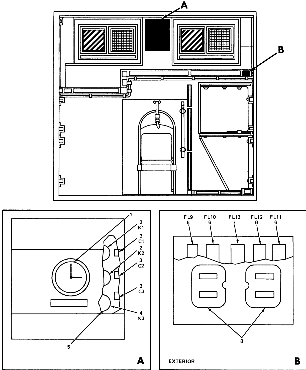
Figure 10. Shelter, Electrical Equipment S-348/TSC-58 and S-348A/TSC-58A, Front Wall
