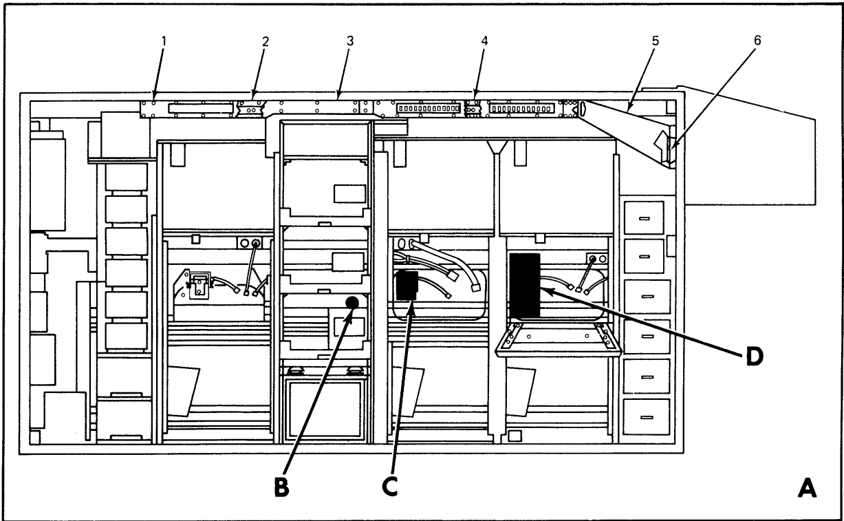
Figure 3. Shelter, Modified S-348A/TSC-58A, Roadside (Sheet 1 of 2).
