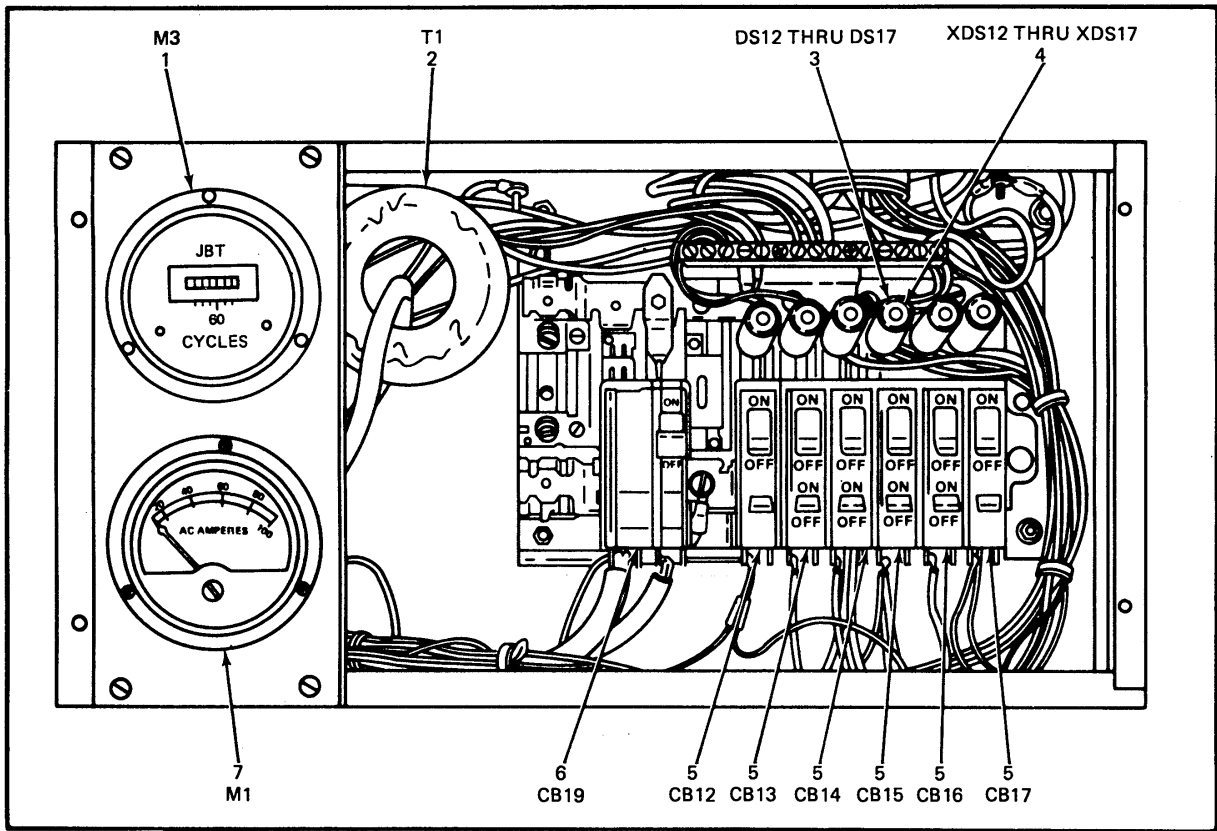
Figure 15. Shelter, Electrical Equipment S-348/TSC-58 and S-348A/TSC-58A, Red Power Distribution Panel.
