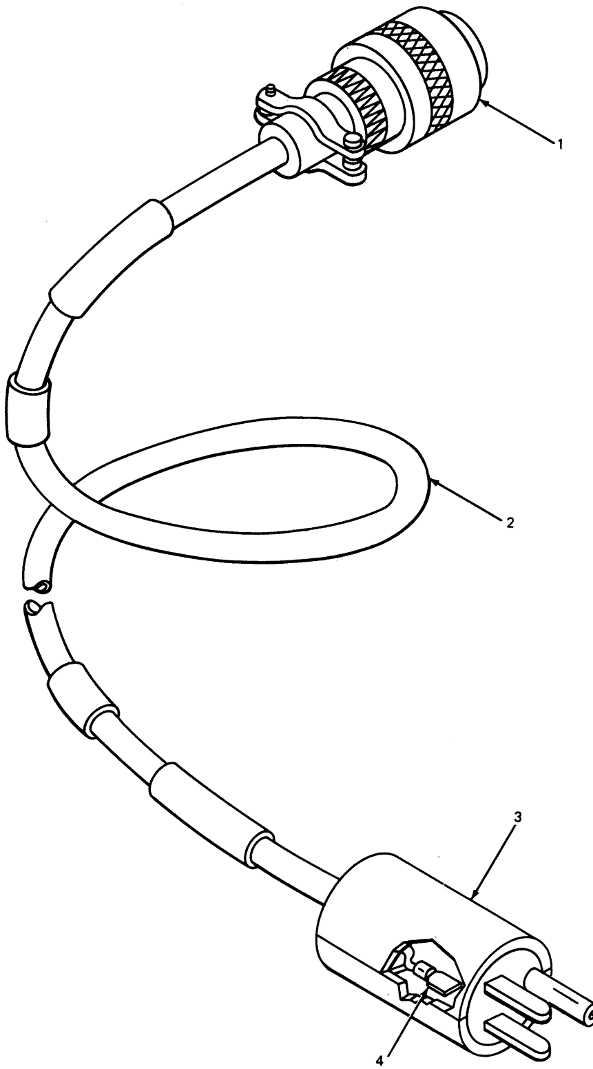
Figure 23. AC Power Cable SC-D-960025-000.
