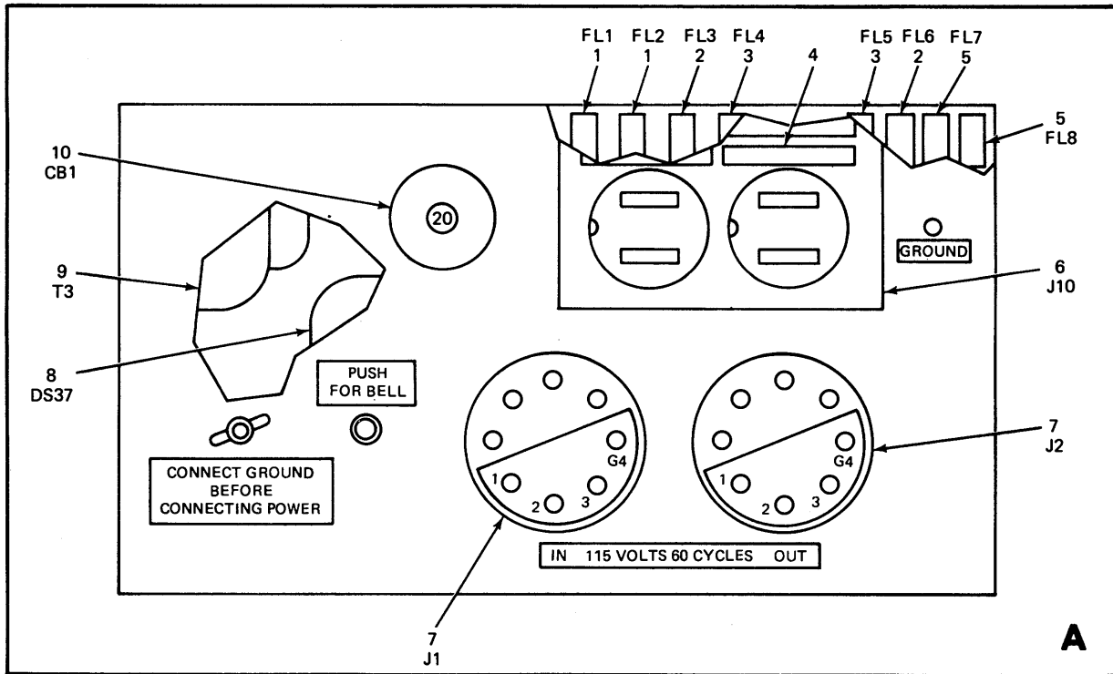
Figure 12. Shelter, Electrical Equipment S-348/TSC-58 and S-348A/TSC-58A, Power Box.
