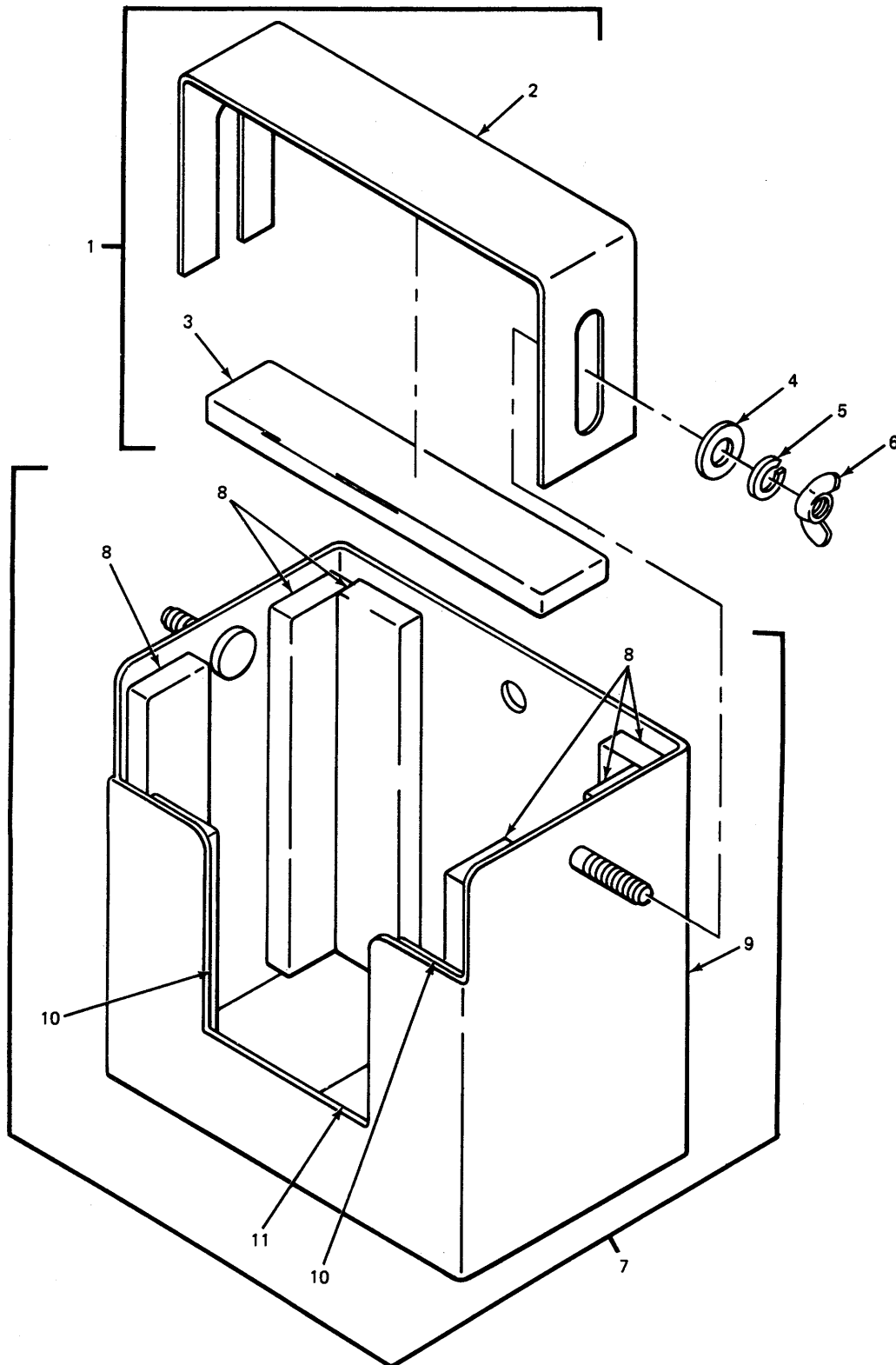
Figure 4. Holder, Battery Assembly.
