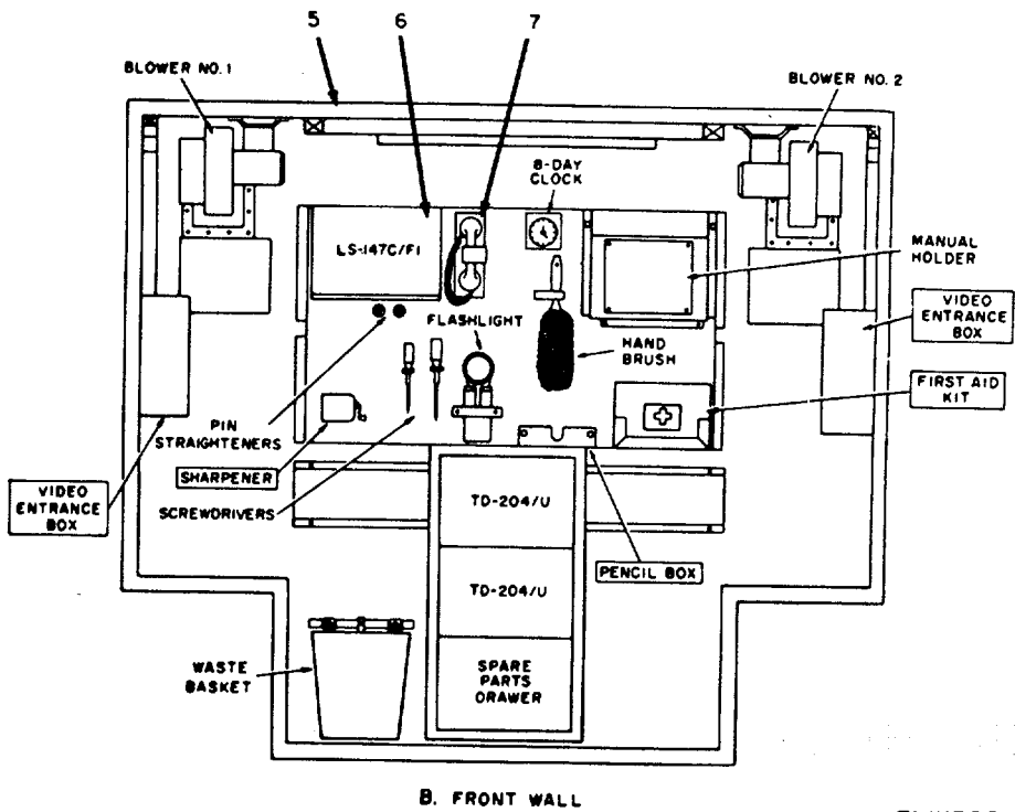
Figure 1. Telephone Terminal AN/TCC-65.
