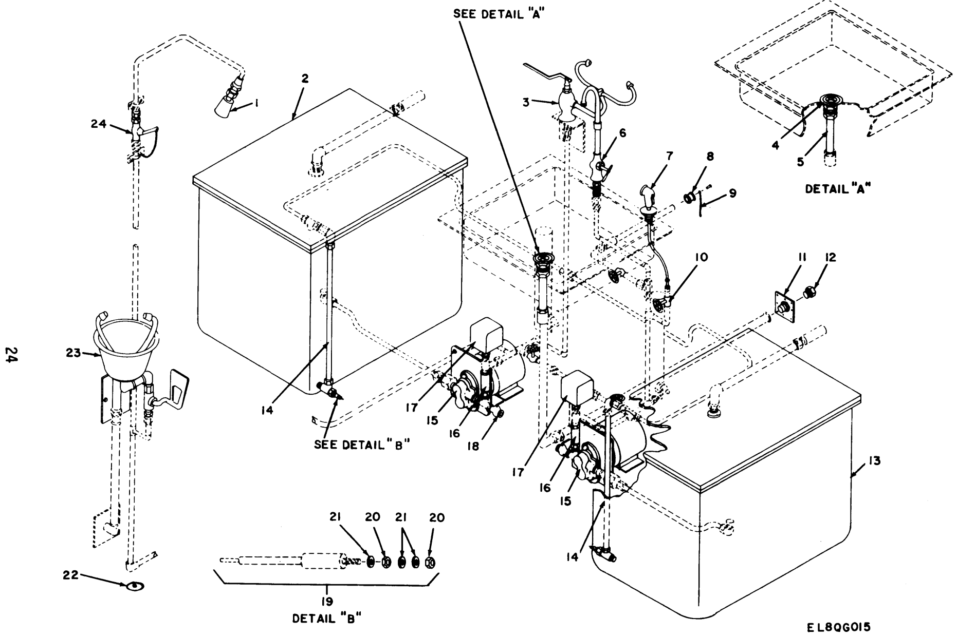
Figure 9. Plumbing installation.
