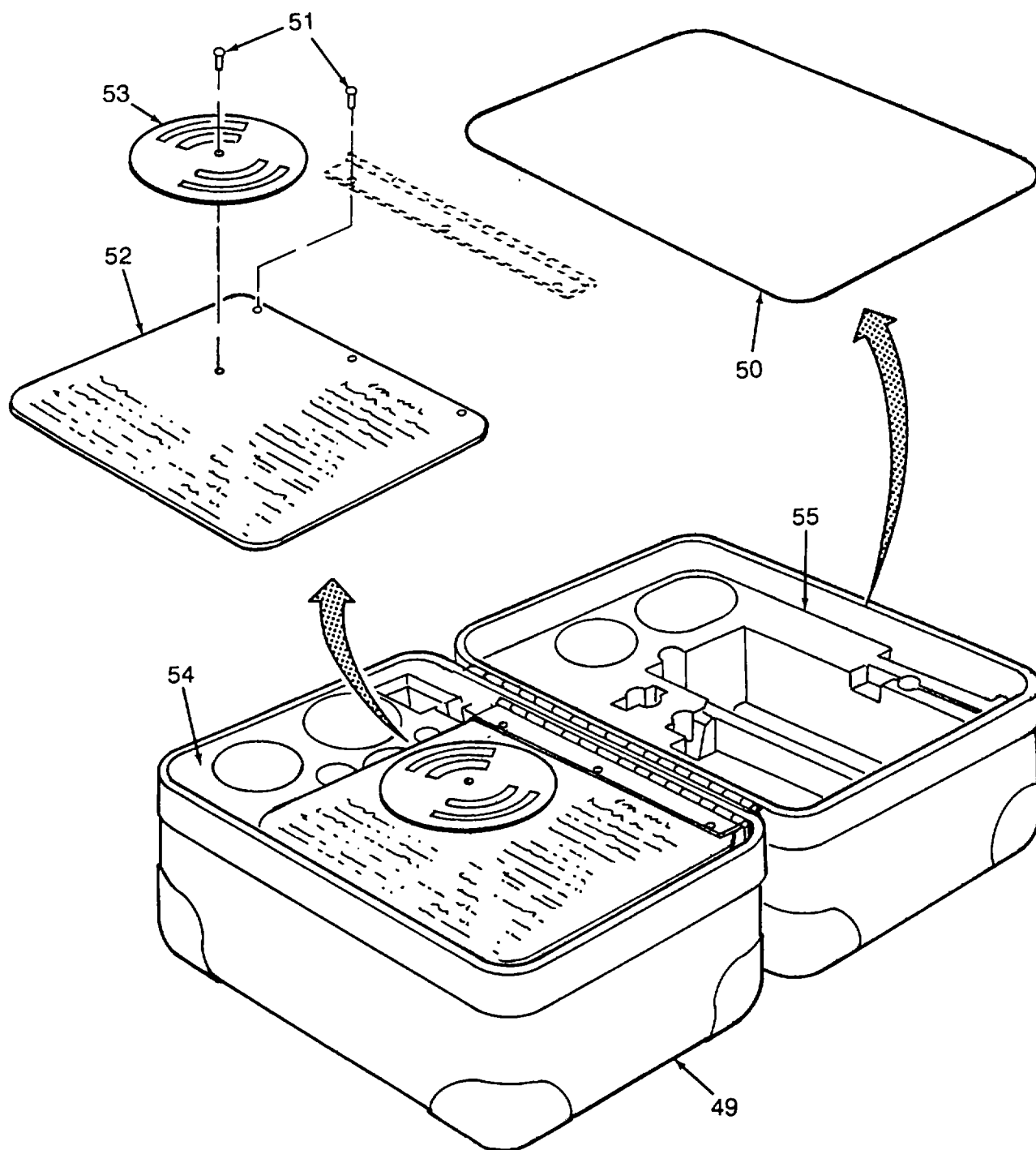
Figure 1. Petroleum Test Kit (Sheet 5 of 5)
