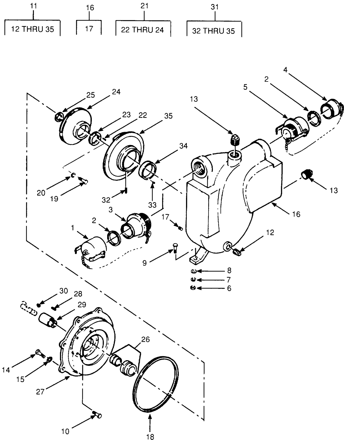
Figure 1. Pump Assembly.
