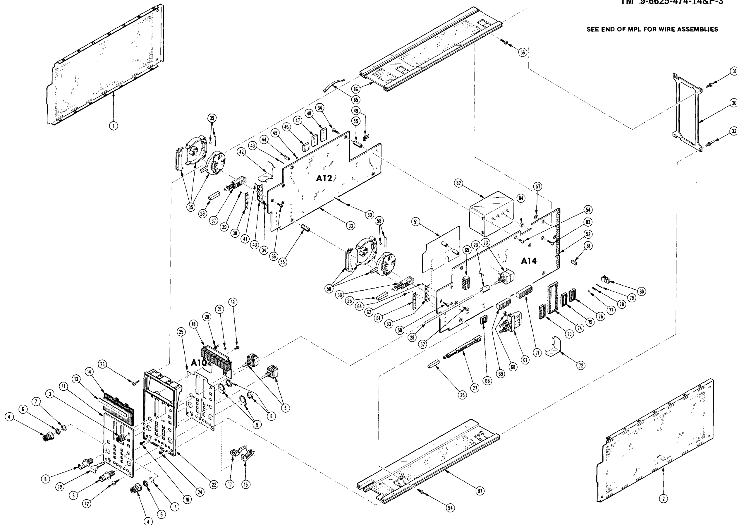
DC 503A UNIVERSAL TIMER/COUNTER EXPLODED VIEW
