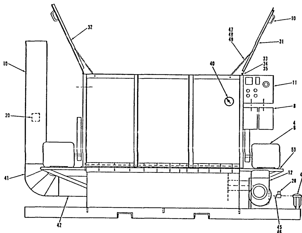
Figure 1 - AUC-81, Front Elevation
