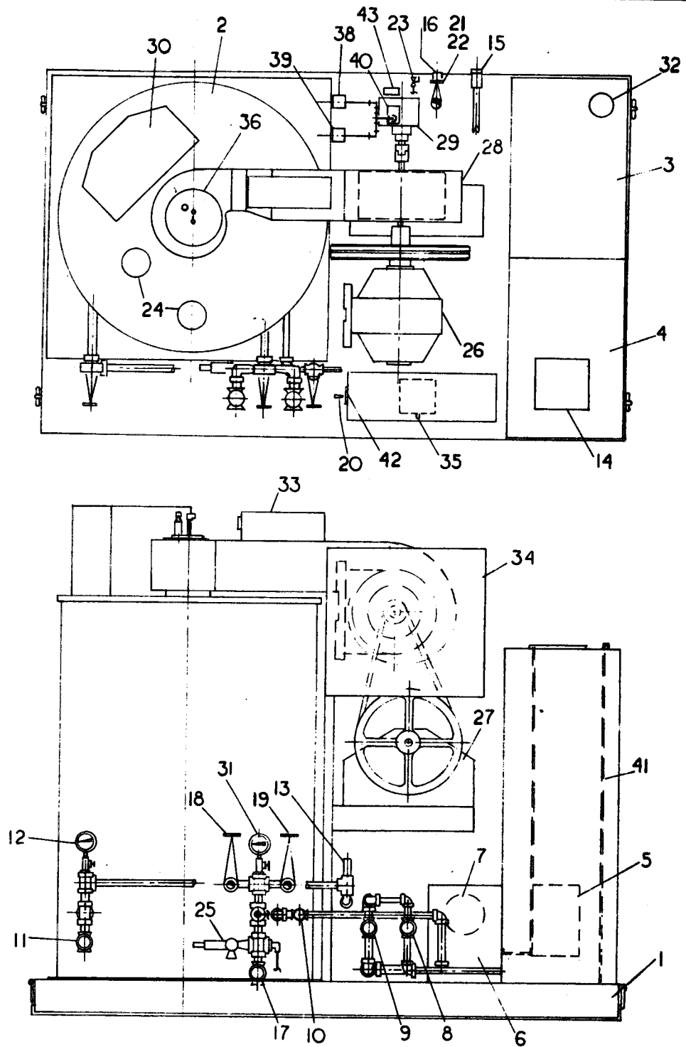
FIG.5 STEAM CLEANER
