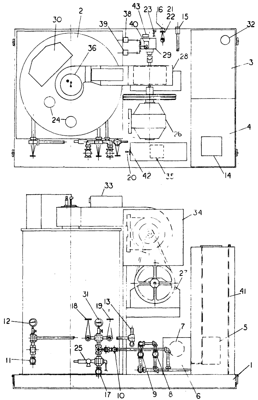
FIG. 1 STEAM CLEANER
