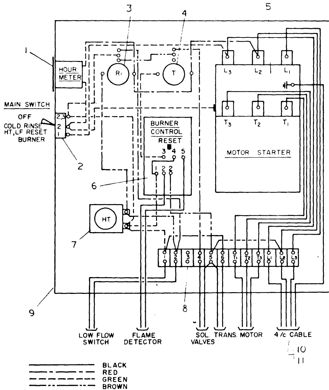
FIG. 9 WIRING DIAGRAM - CONTROL PANEL
