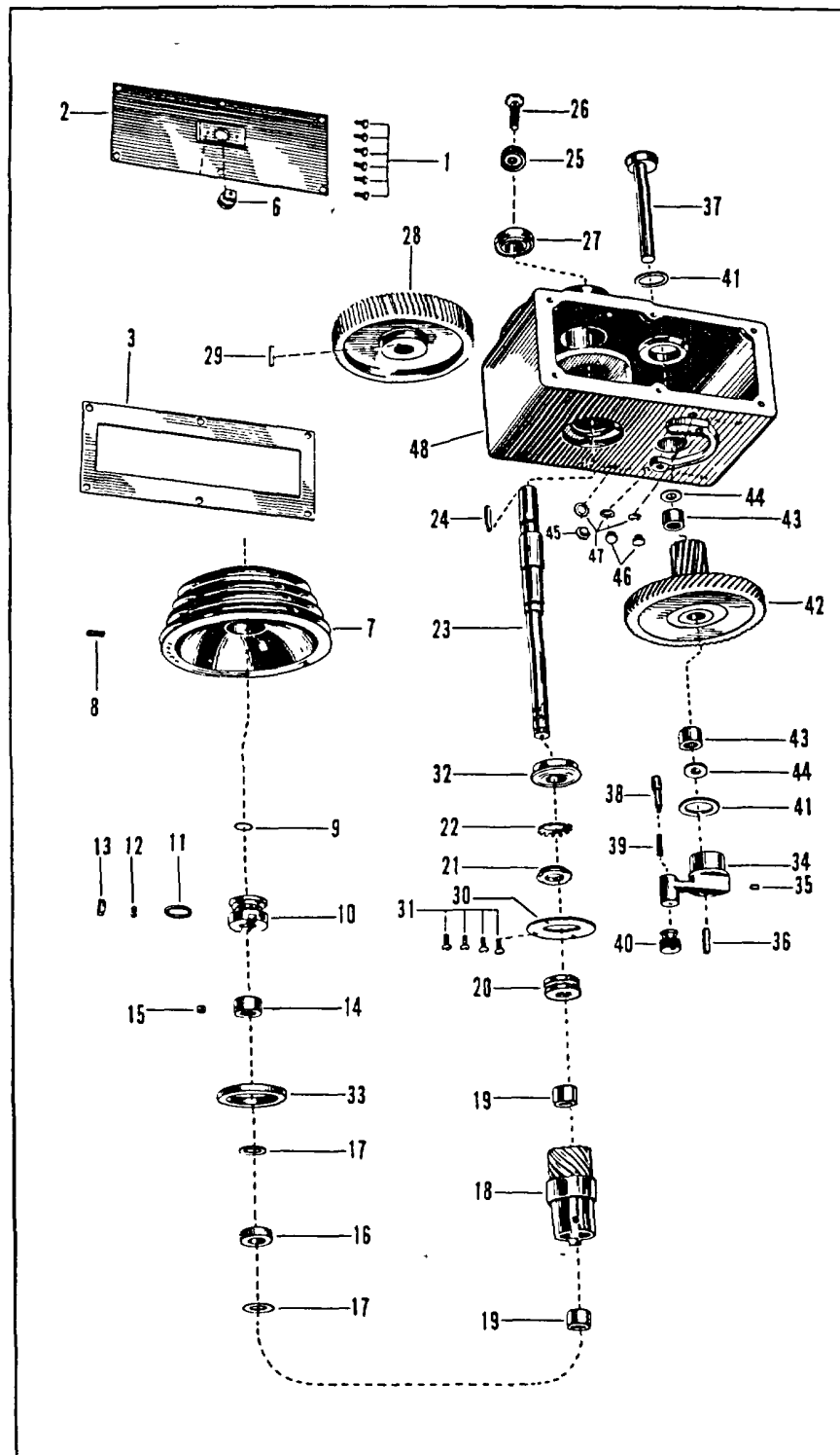
Figure 9. Transmission Assembly - Band Saw, Eight-Speed
