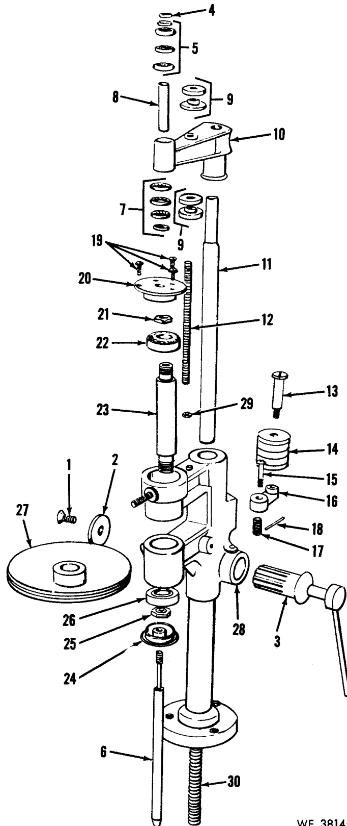
Figure 1. Drilling machine.
