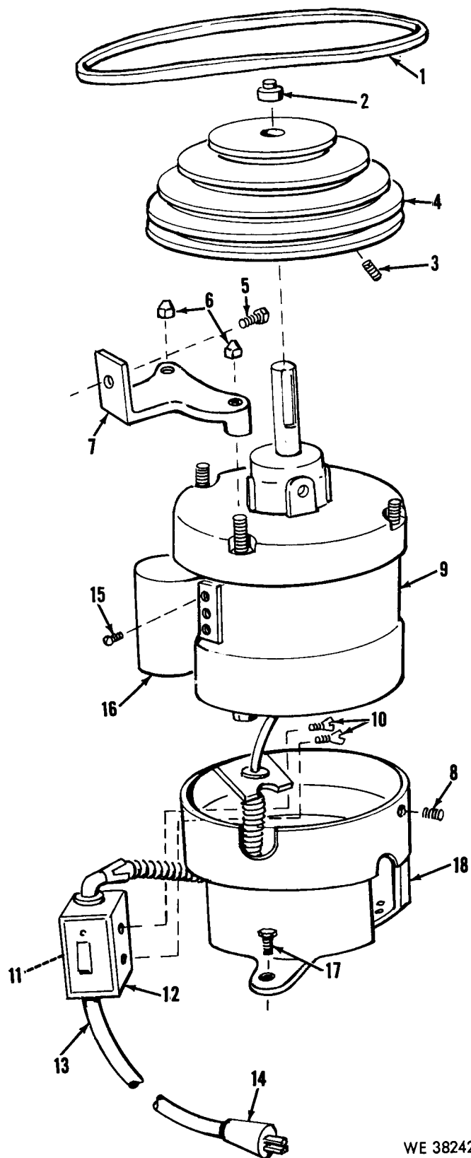
Figure 2. Drilling machine (motor group).
