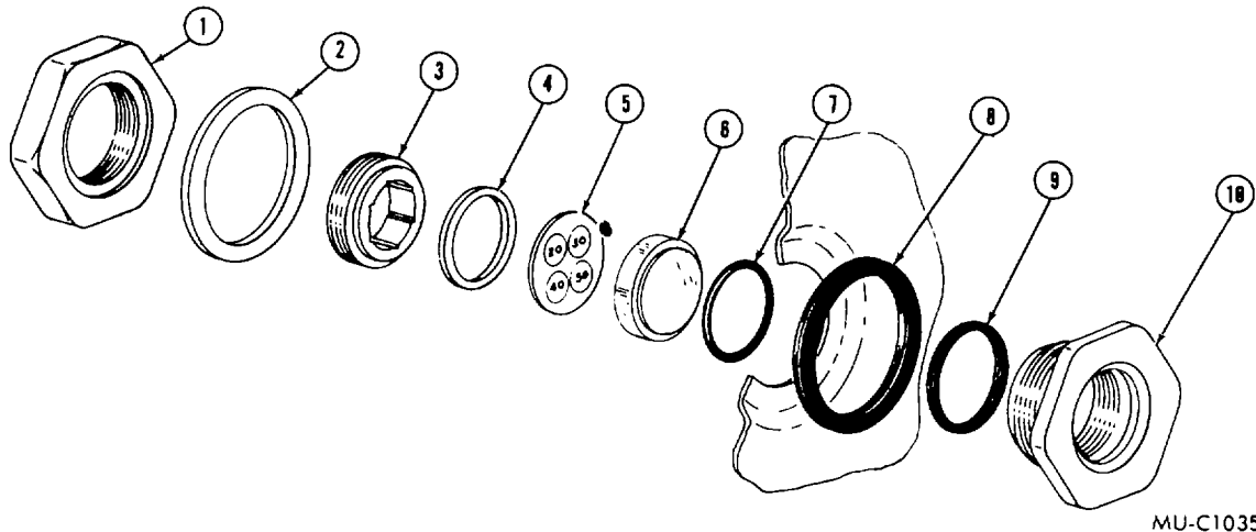
Figure C2. Indicator, Humidity, Plug.
