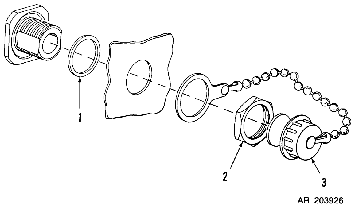
Figure C3. Vent Assembly
