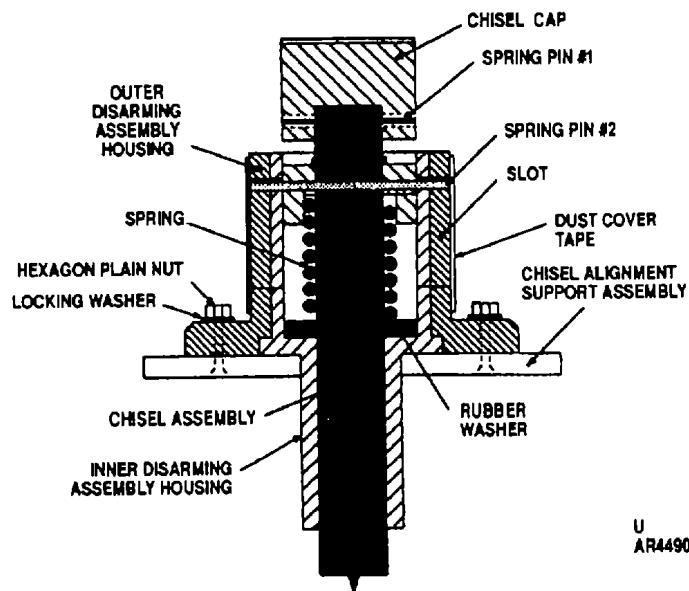
Disarming Assembly.
