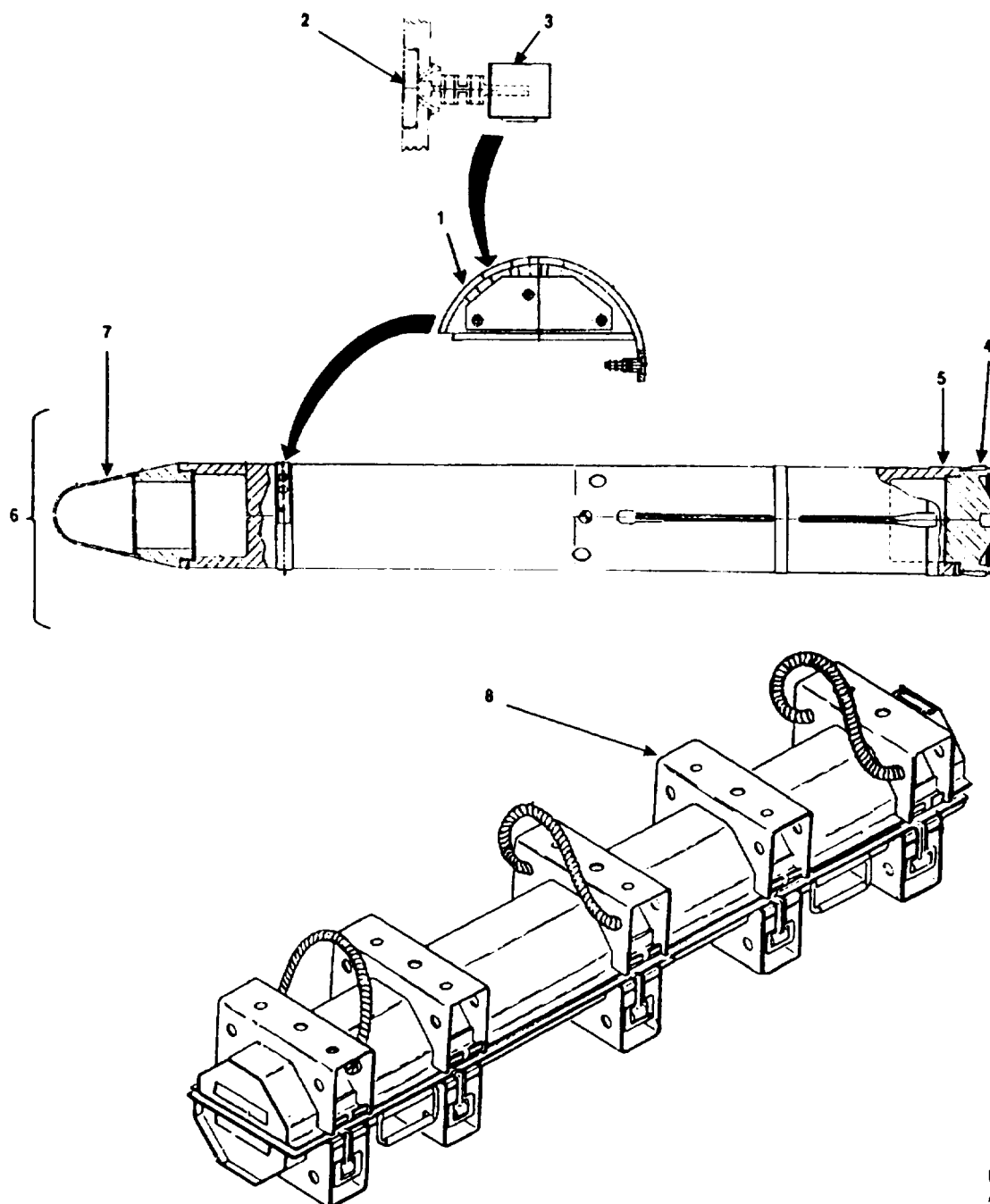
FIGURE C1. PROJECTILE, 155MM:
