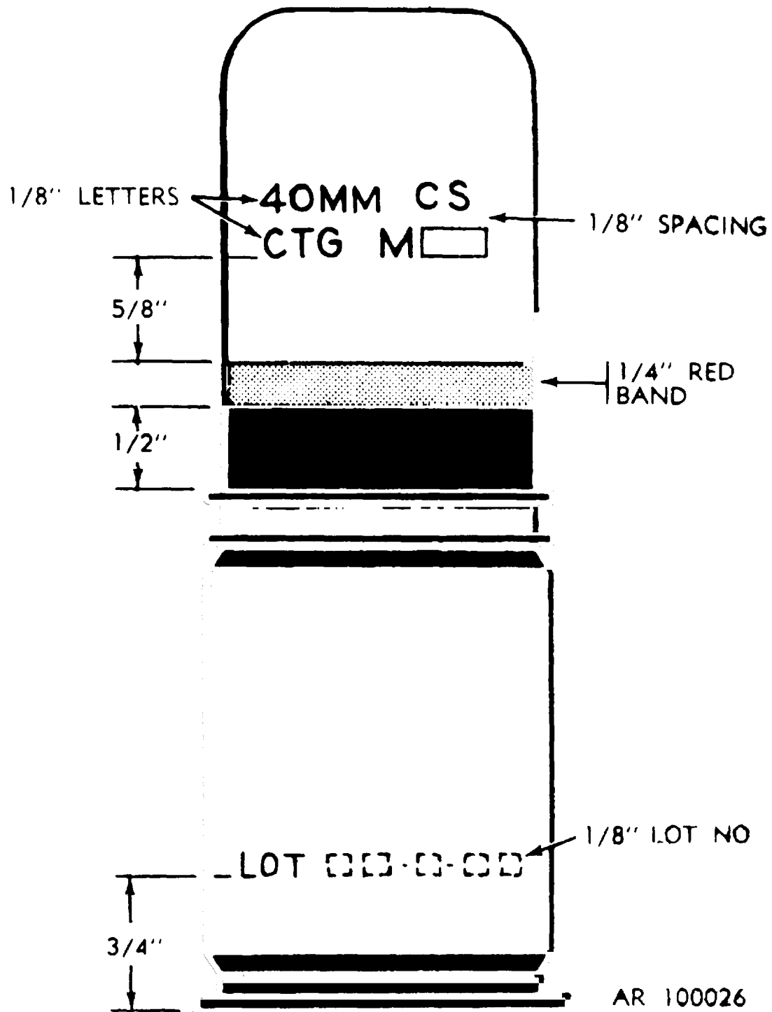
Figure E-4. Typical marking for 40mm grenade cartridge M651.
