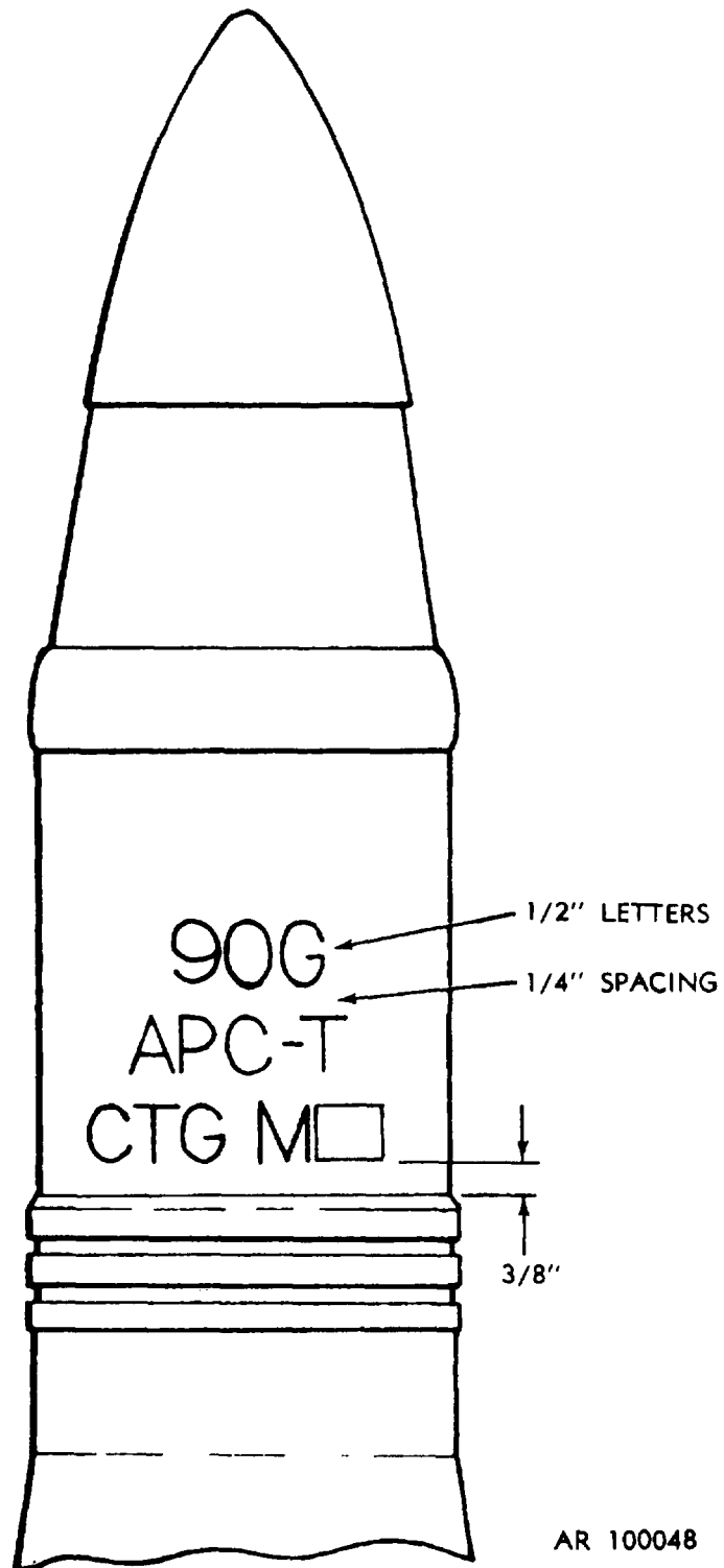
Figure E-36. Typical marking for 90mm gun cartridge M82.
