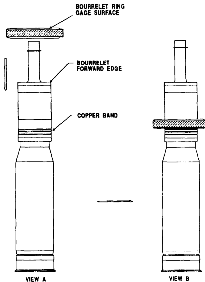
Figure 4-9. Bourrelet ring gage.
