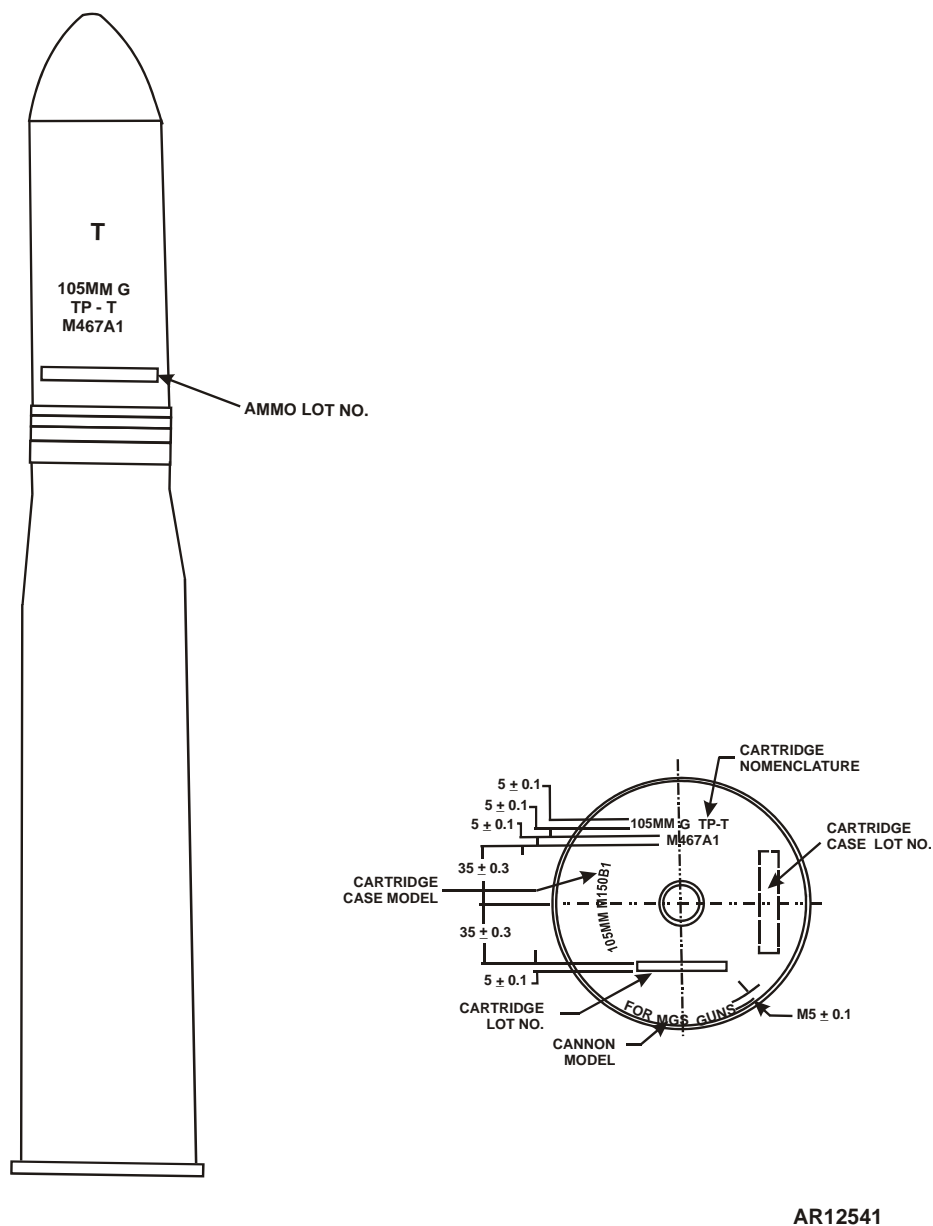
Figure E-55.3. Typical Marking for 105mm Gun Cartridge M467A1.
