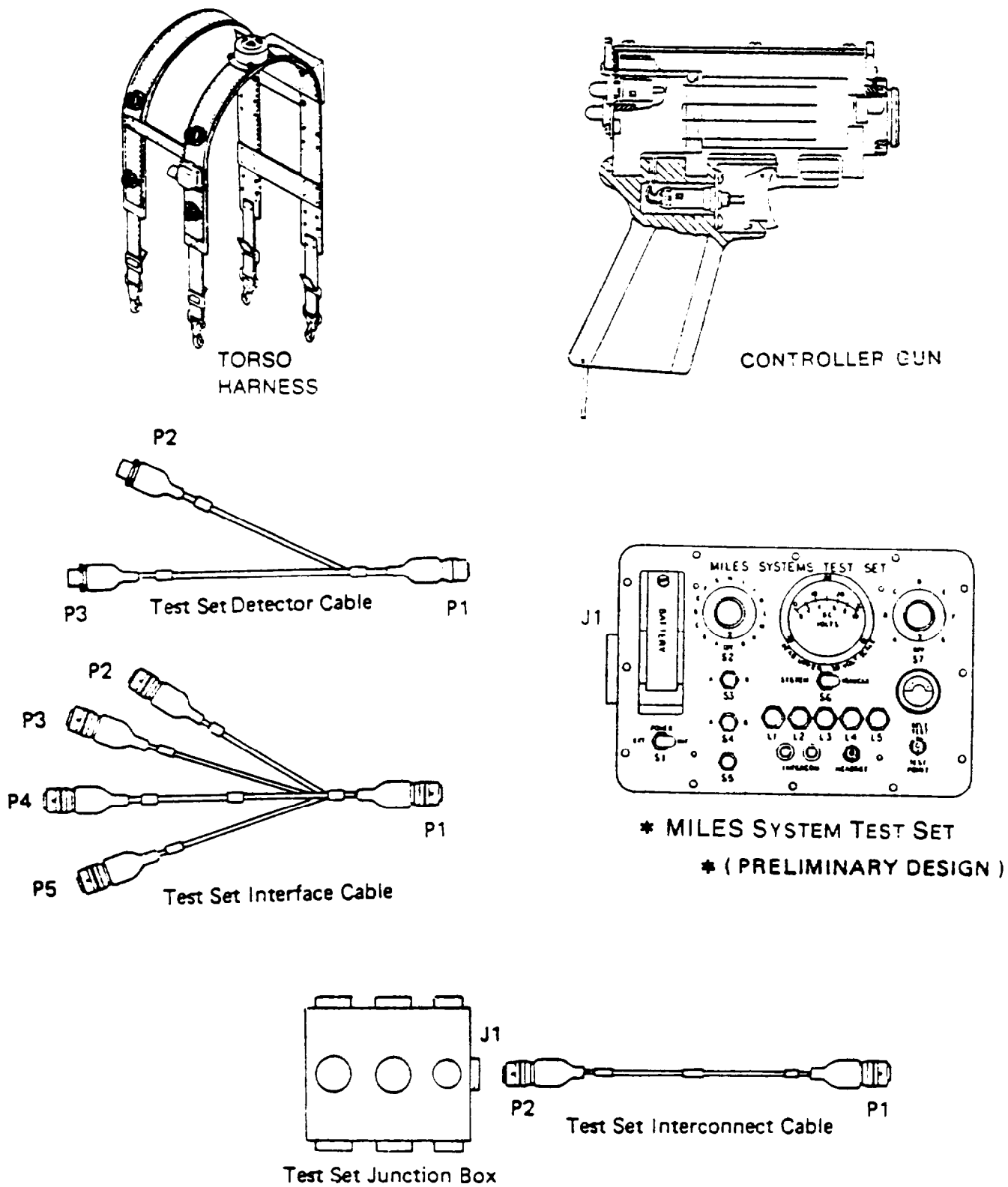
Figure 3-1. MILES UH-1H Helicopter Troubleshooting Equipment
