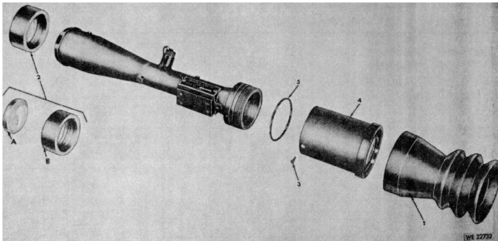
Figure 1. Telescope M120 or telescope XM134 - partial exploded view.
