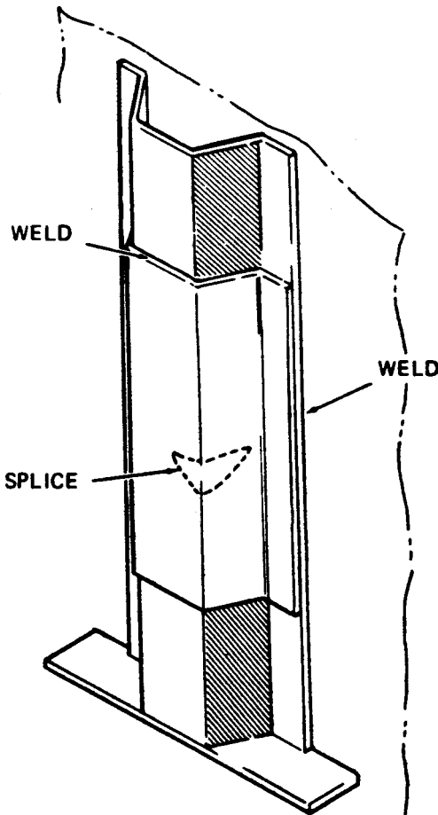
Figure 4-3 Corrugated Panel Repair.
