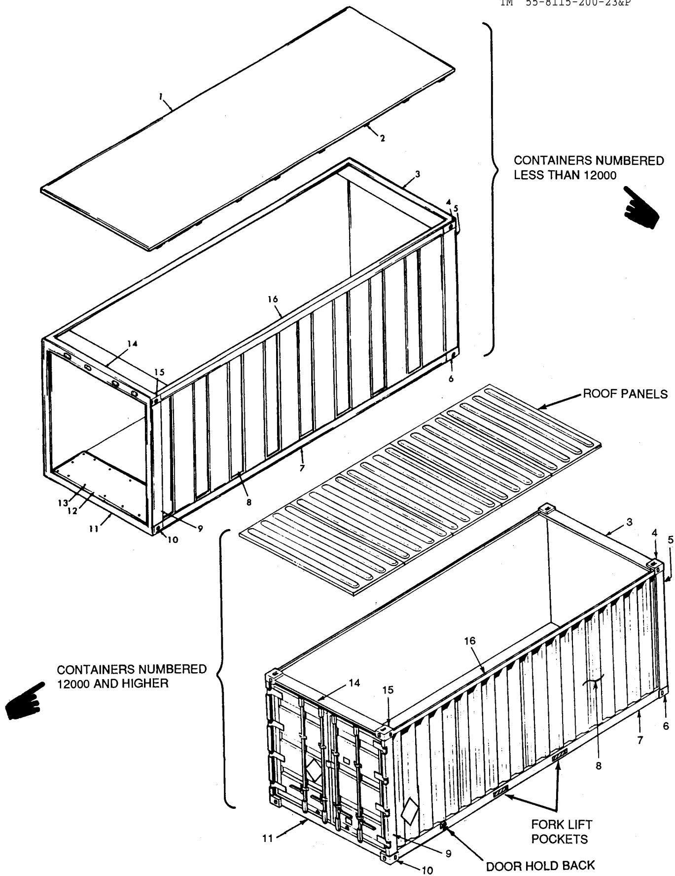
Figure 1-1. Container Assembly.
