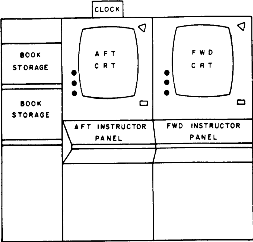
Figure 2-2. Instructor Station Layout
