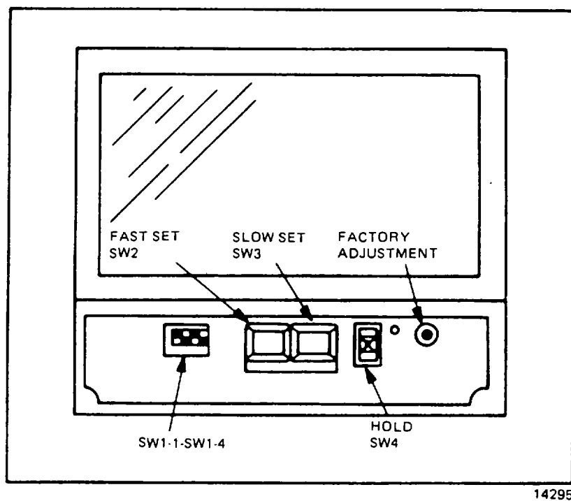
Figure 8-4. Digital Clock (Front View, Access Cover Removed)
