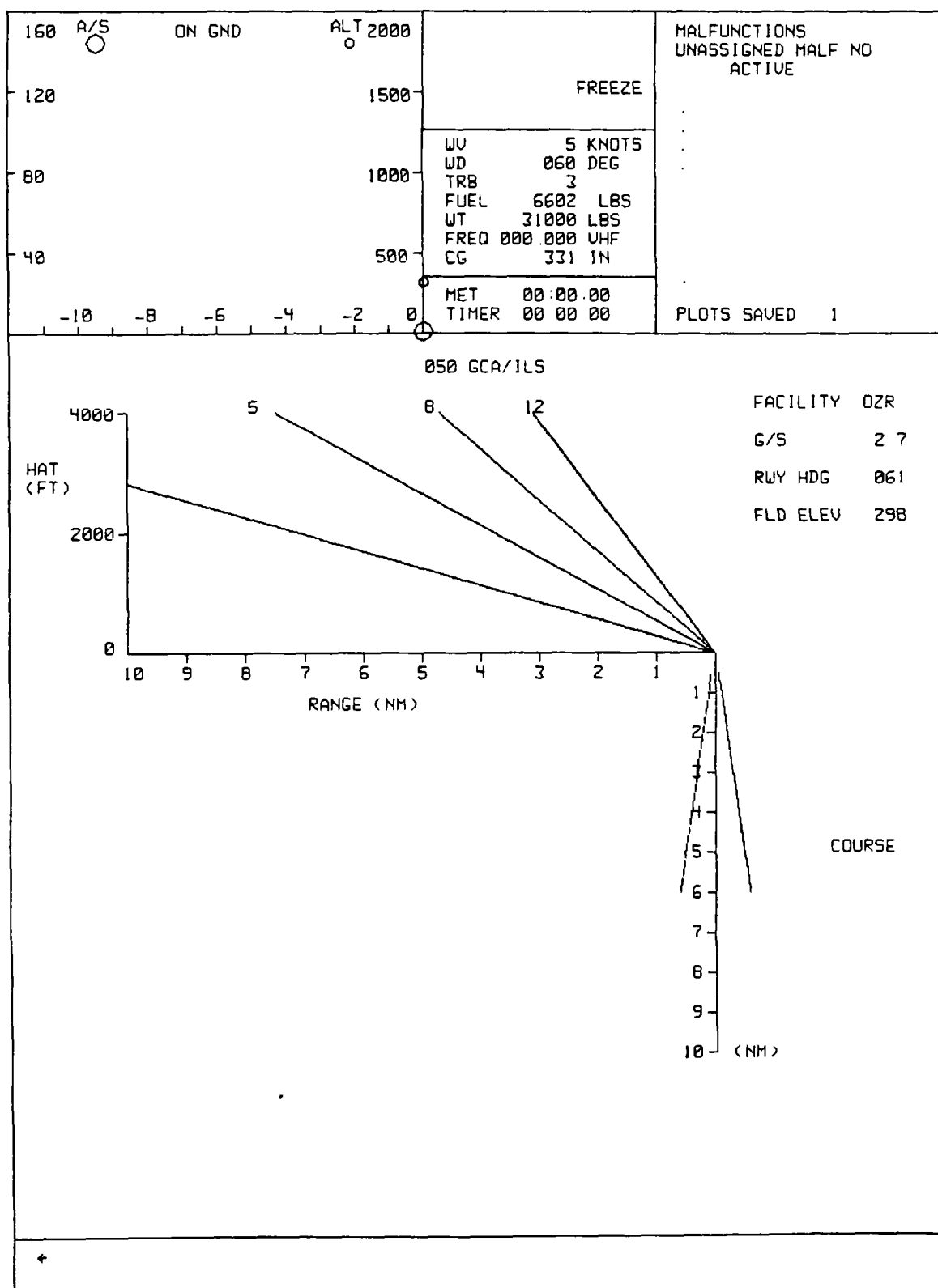
Figure 2-5. Typical Lower GCA/ILS Display
