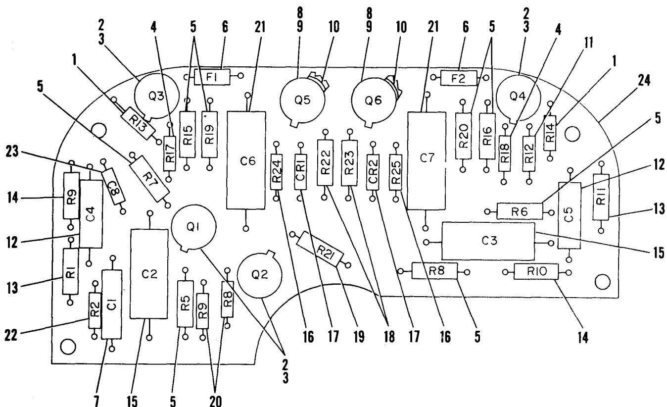
Figure 2-4. Electronic Control Amplifier.
