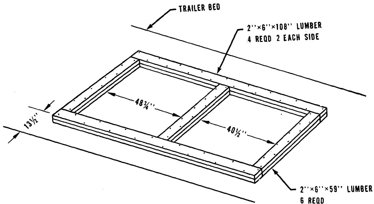
Figure 5-5. Shoring for M1015 carrier on M127-series semitrailer.
