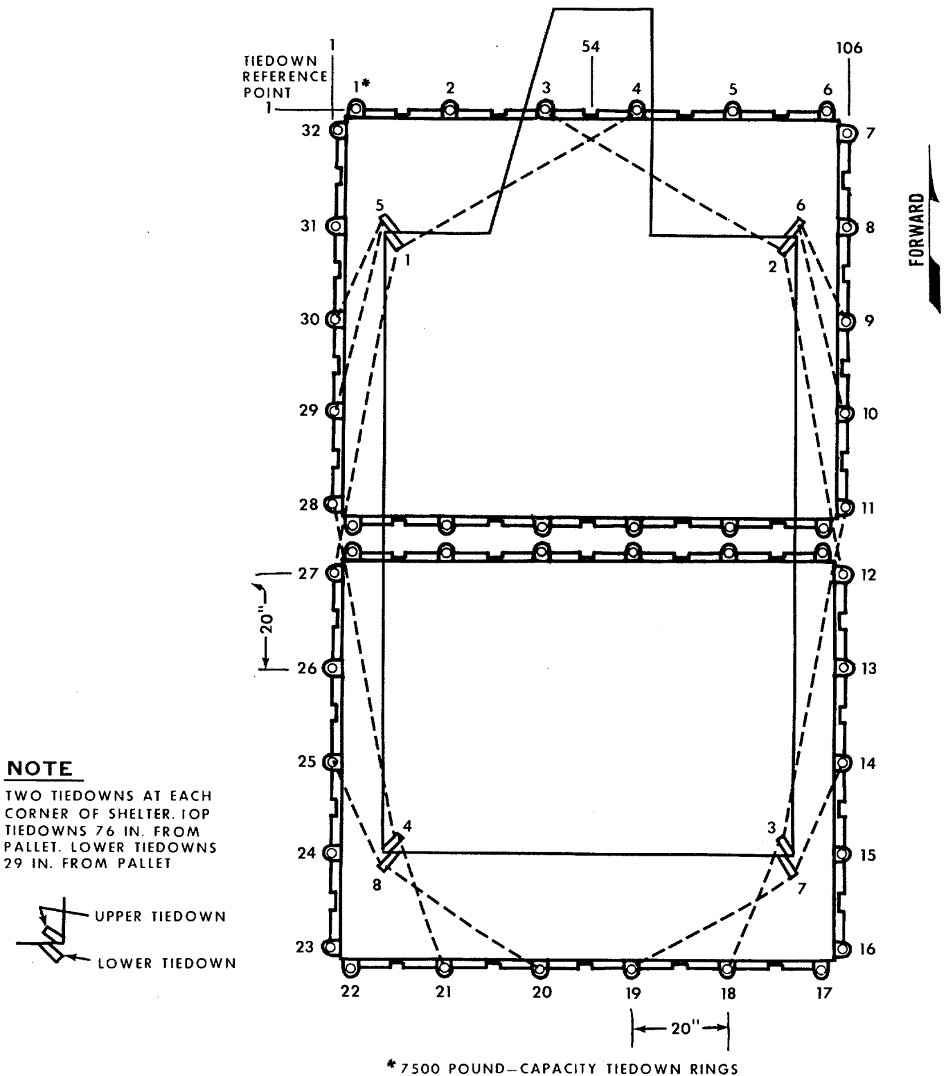
Figure 4-5. Tiedown diagram for shelters on two interlocked 463L pallets.
