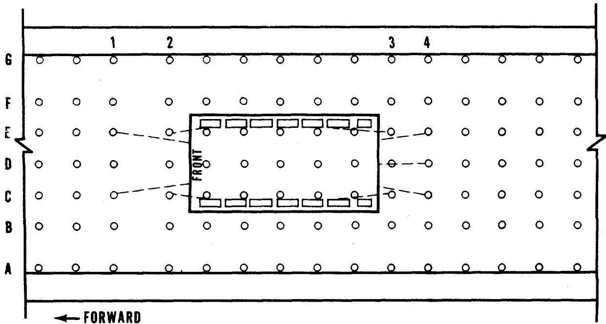
Figure 4-1. Tiedown diagram for M1015 carrier in C-5 aircraft.
