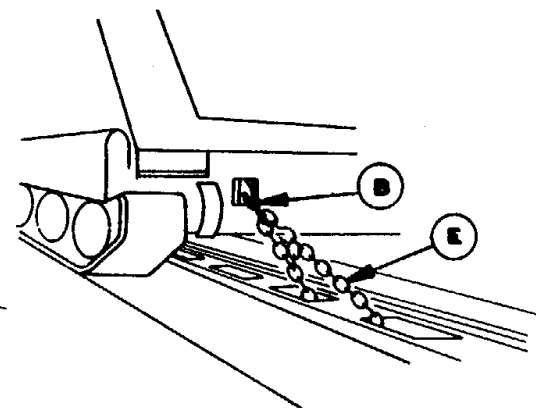
SKETCH - 3 DETAIL OF CHAIN THRU CUSHIONED RUB RAIL SLOTS
