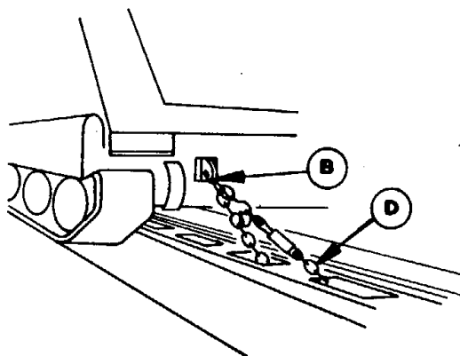
SKETCH - 2 DETAIL OF CHAIN WITH TURN BUCKLE THRU CUSHIONED RUB RAIL SLOTS
