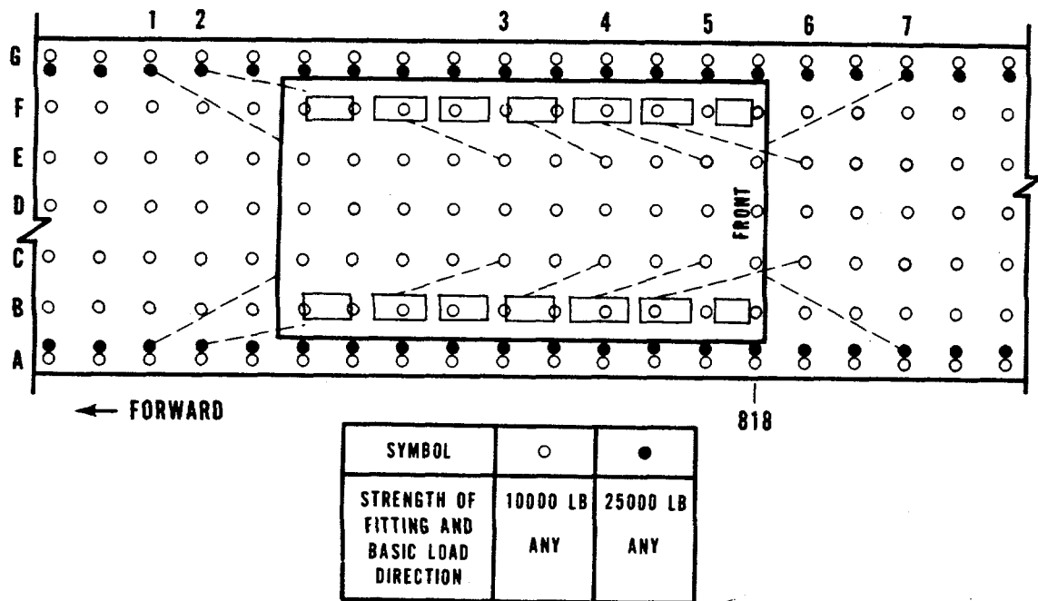
Figure 4-2. Tiedown diagram for M1015 carrier in C-141 aircraft.
