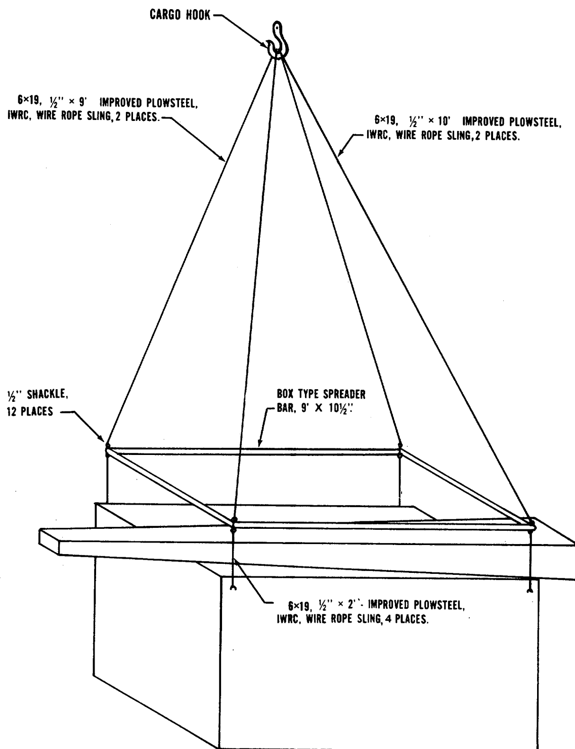
Figure 6-5. Lifting diagram for shelters.
