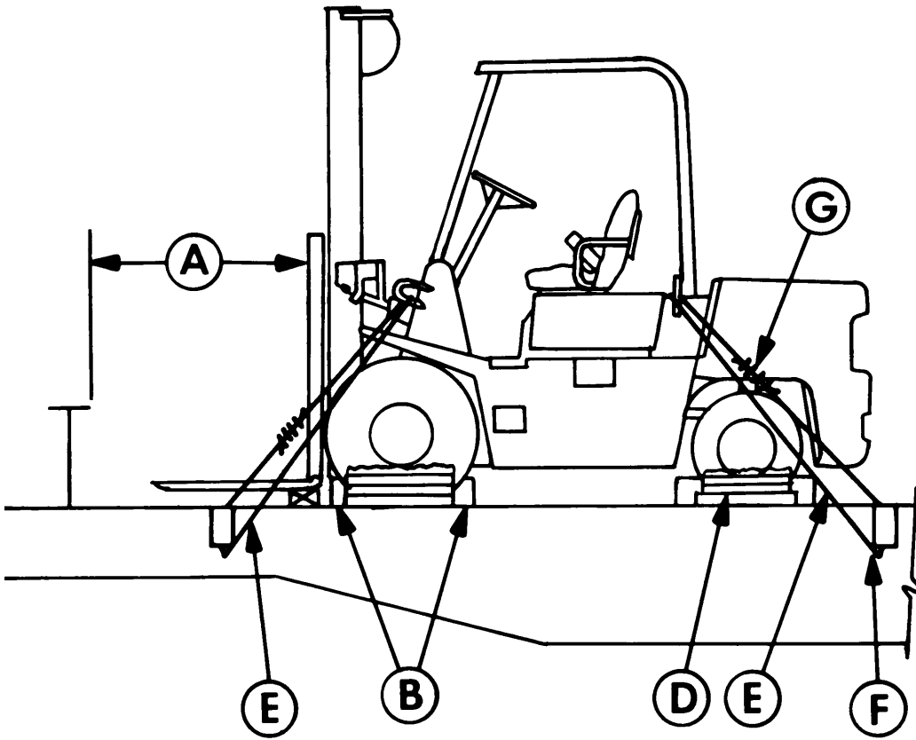
Figure 7-1. Blocking and tiedown of typical forklift on CONUS general-purpose flatcar.
