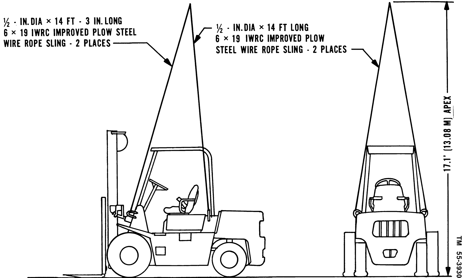
Figure 6-2. Lifting the clean burning diesel forklift, 6k-pound capacity, Hyster Co, model H60XL.
