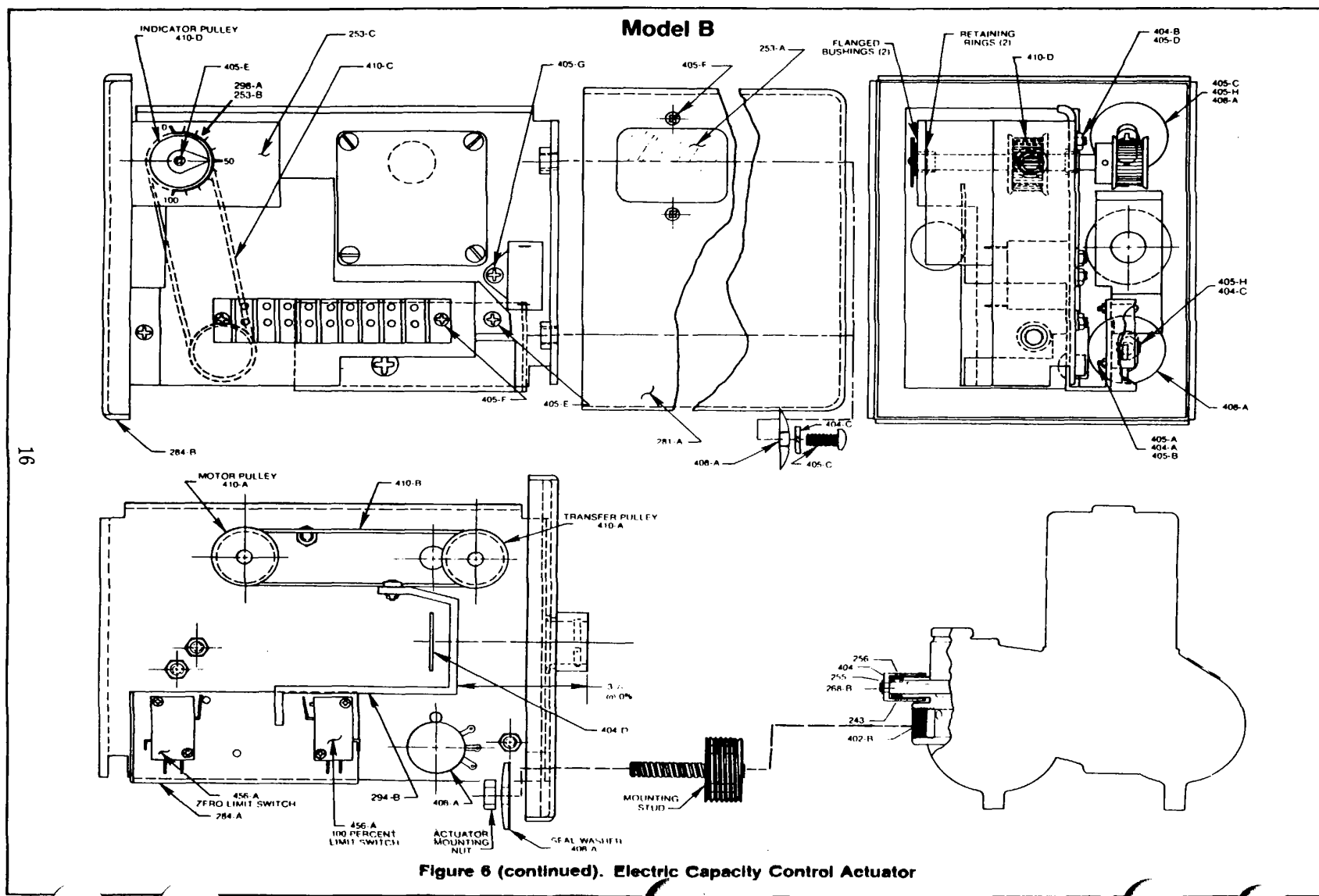
Figure. 6 (continued). Electric Capacity Control Actuator
