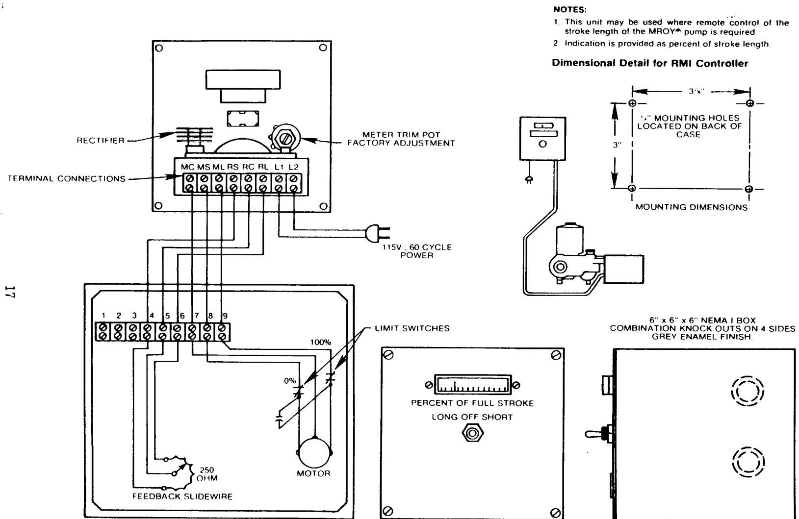
Figure 7. Model RMI Controller-to-Actuator Wiring Diagram
