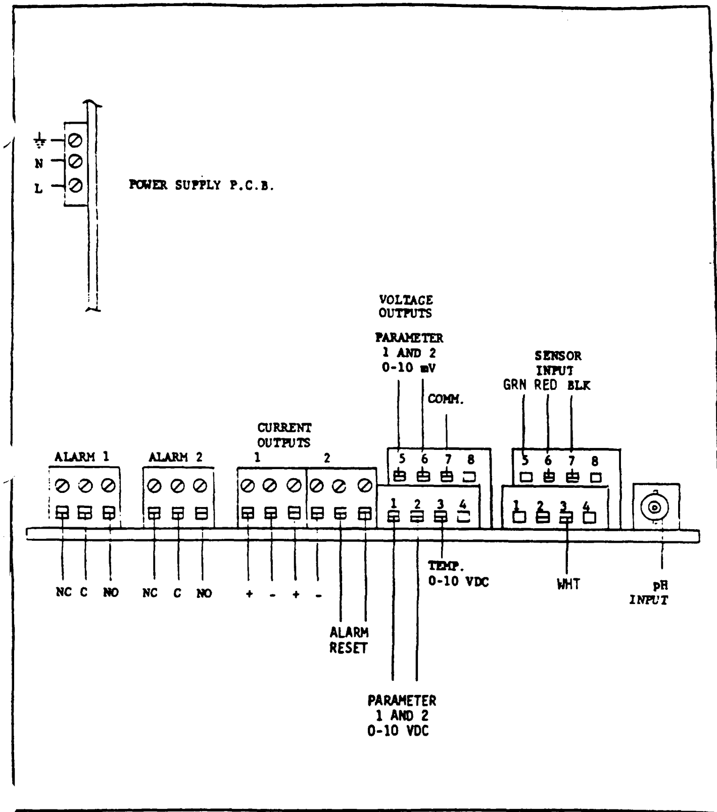
Fig. 3 - 924 External Connections
