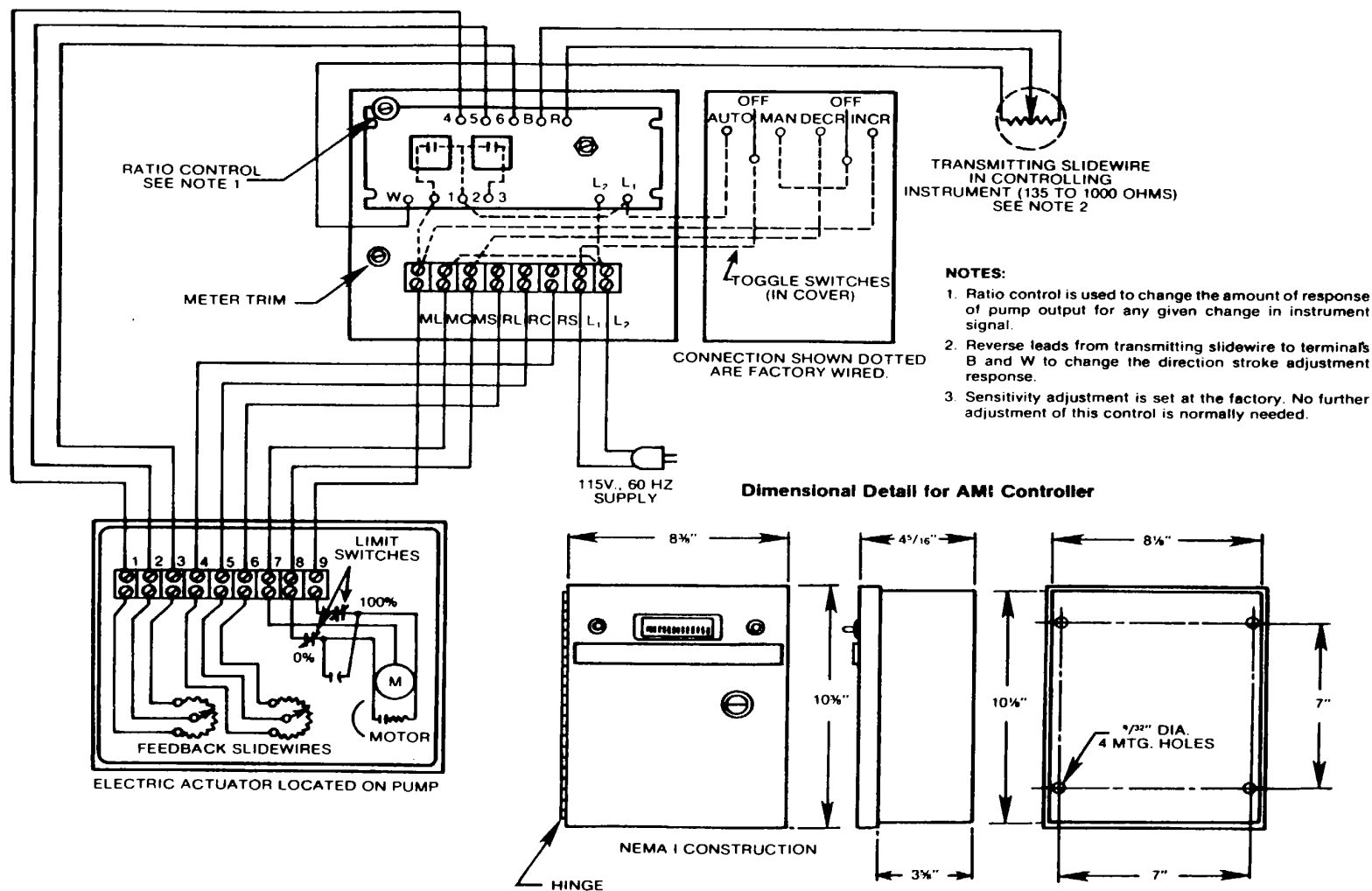
Figure 10. Model AMI Controller-to-Actuator Wiring Diagram
