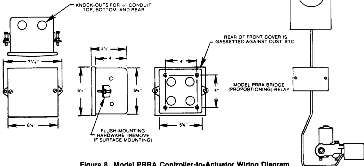
Figure 8. Model PRRA Controller-to-Actuator Wiring Diagram
