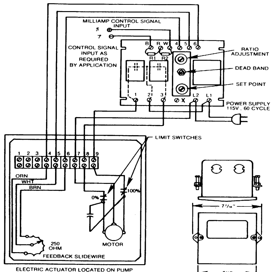
Figure 9. Model PRRA-MA Controller-to-Actuator Wiring Diagram
