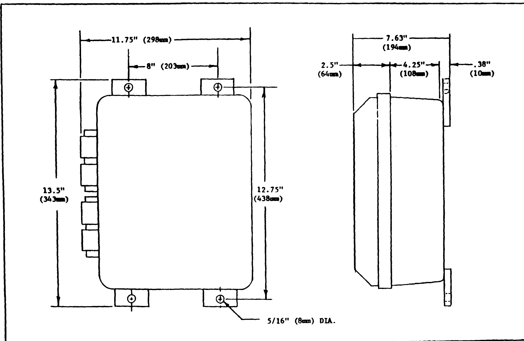
Fig. 8 Analyzer Dimensions
