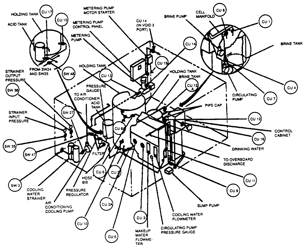
Figure 1-2. Chlorination System Installation (Barge 1)
