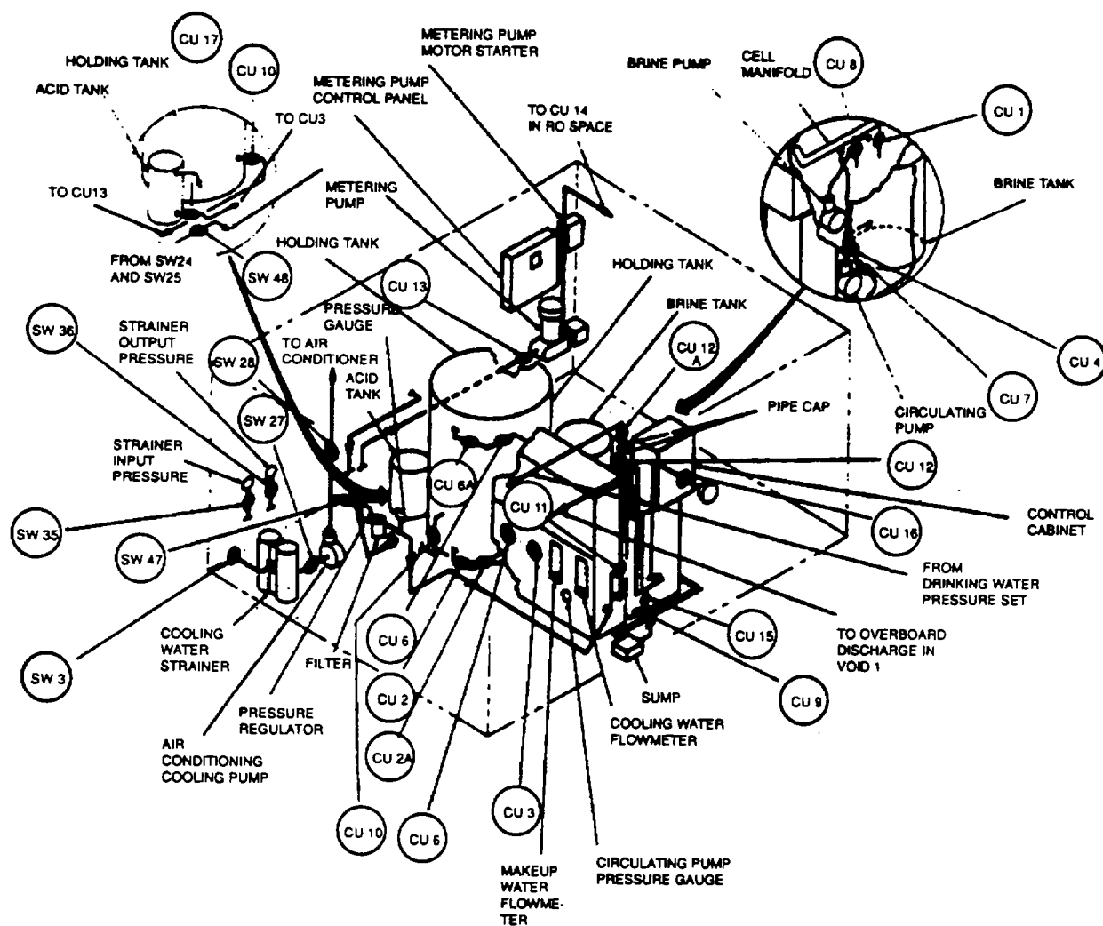
Figure 1-3. Chlorination System Installation (Barges 2 and 3)
