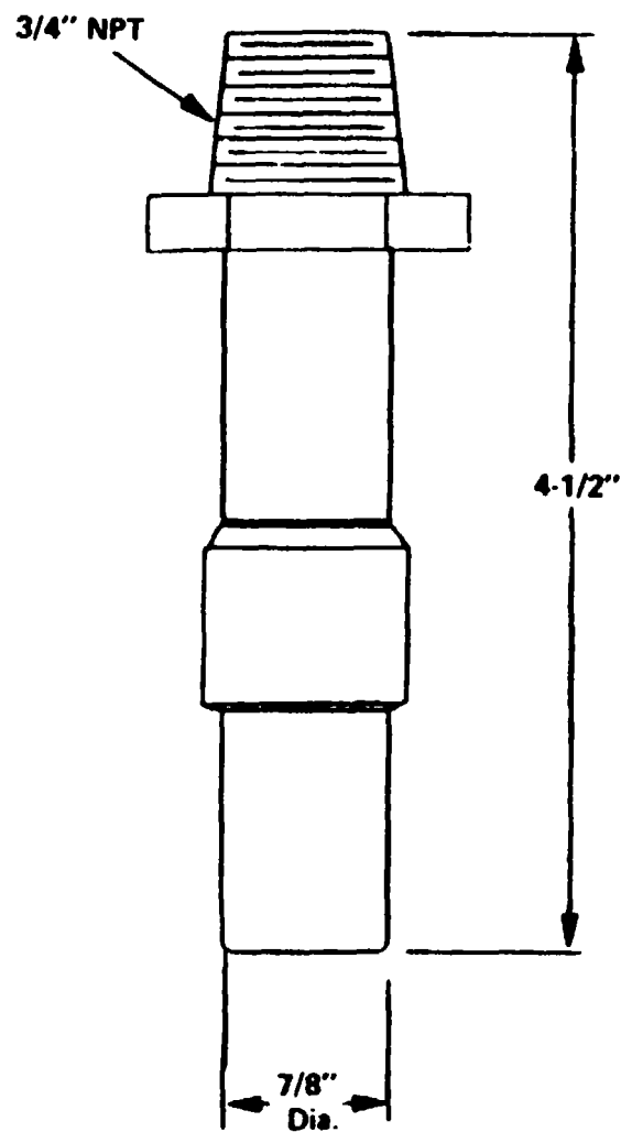
FIG. 6 - Optional pH Sensor Dimensional Dwg.
