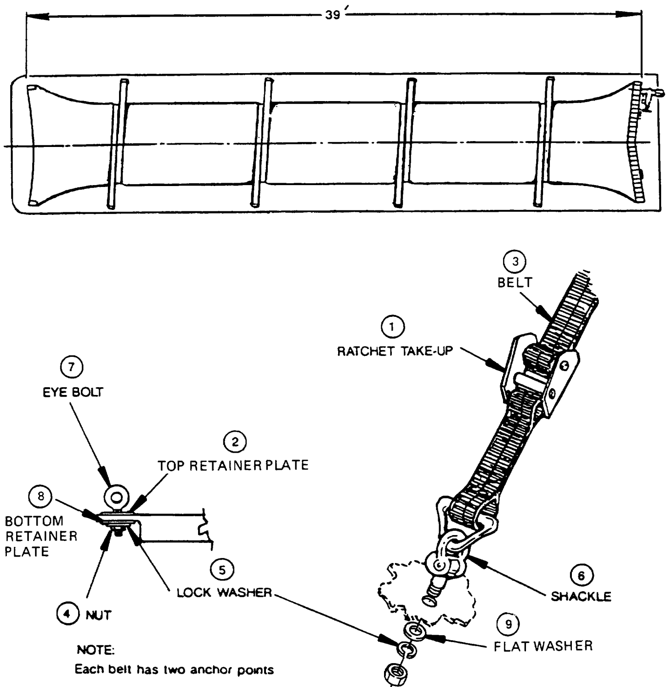
Figure 2-3A. Tie-Down Assembly (Model 91094)
