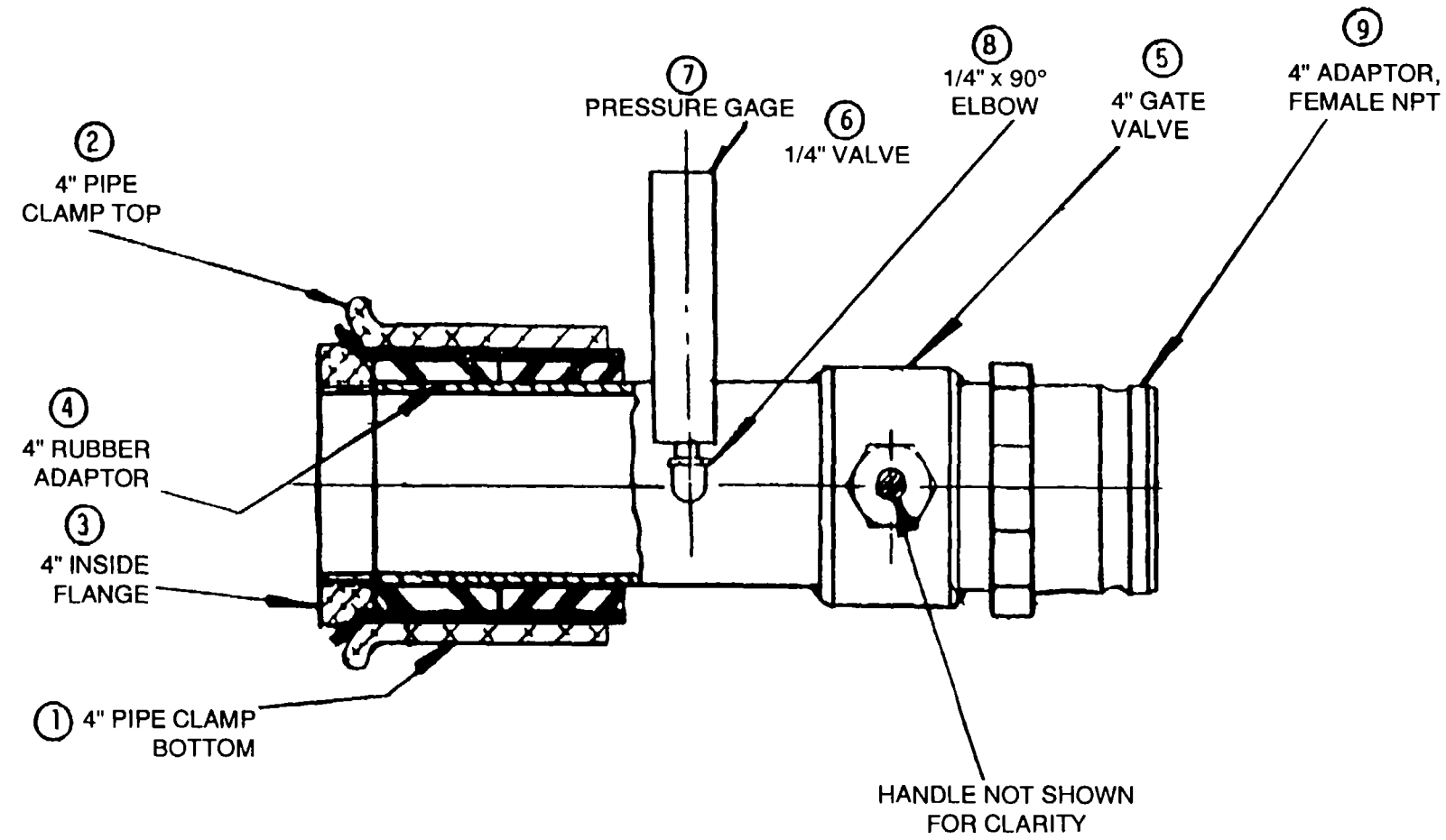
Figure C-2. FILLER/DISCHARGE ASSEMBLY (MODEL 5,000 gallon)
