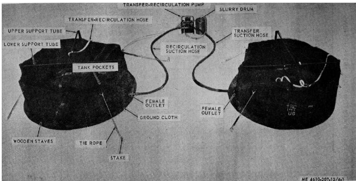
Figure 4-1. Tank detail.
