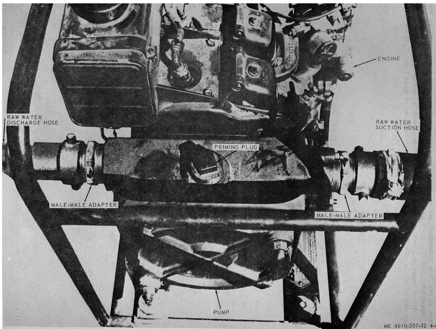
Figure 4-6. Raw water pump details.
