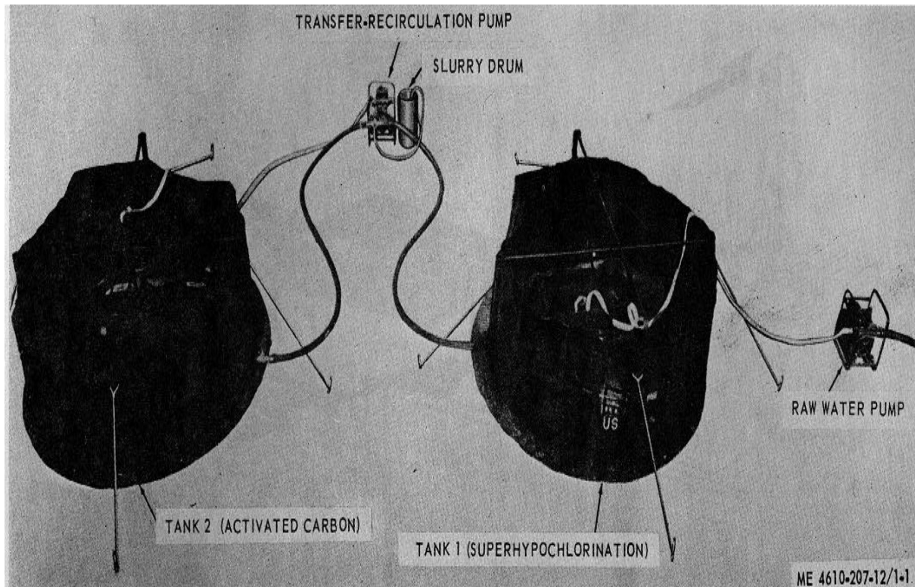
Figure 1-1. Tanks, hoses, and pumps, physical arrangement
