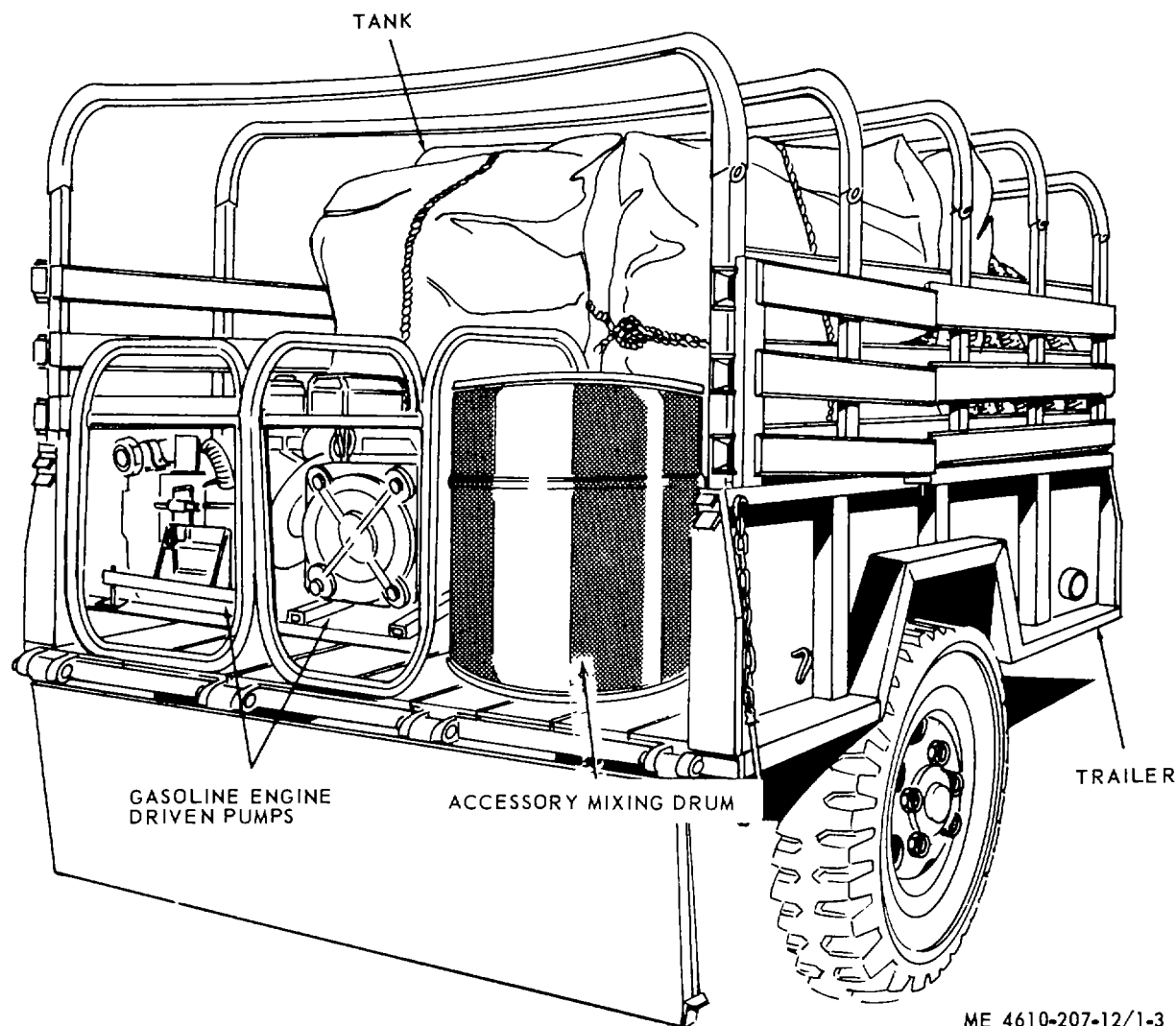
Figure 1-3. Trailer, rear, loaded (without cover).
