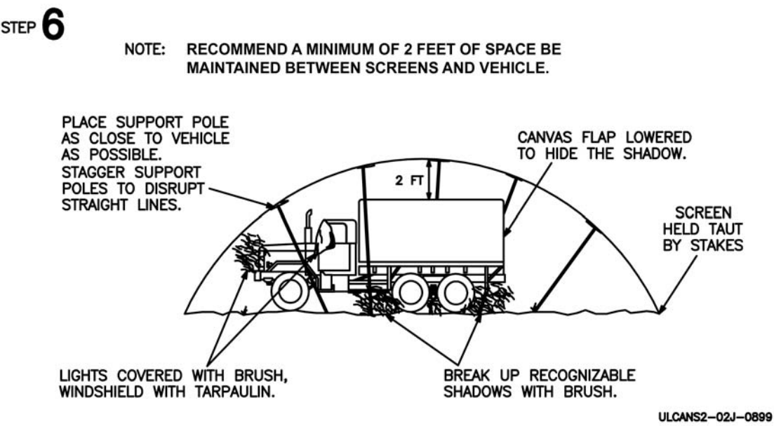
Figure 2-2. Deployment/Retrieval/Storage Instructions, ULCANS (Sheet 8 of 9)
