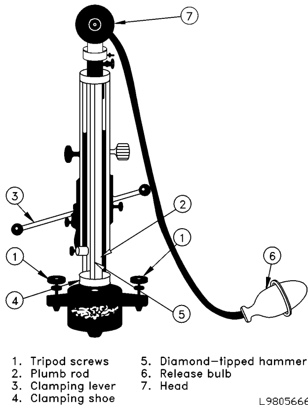
Figure 8-6. Shore Scleroscope
