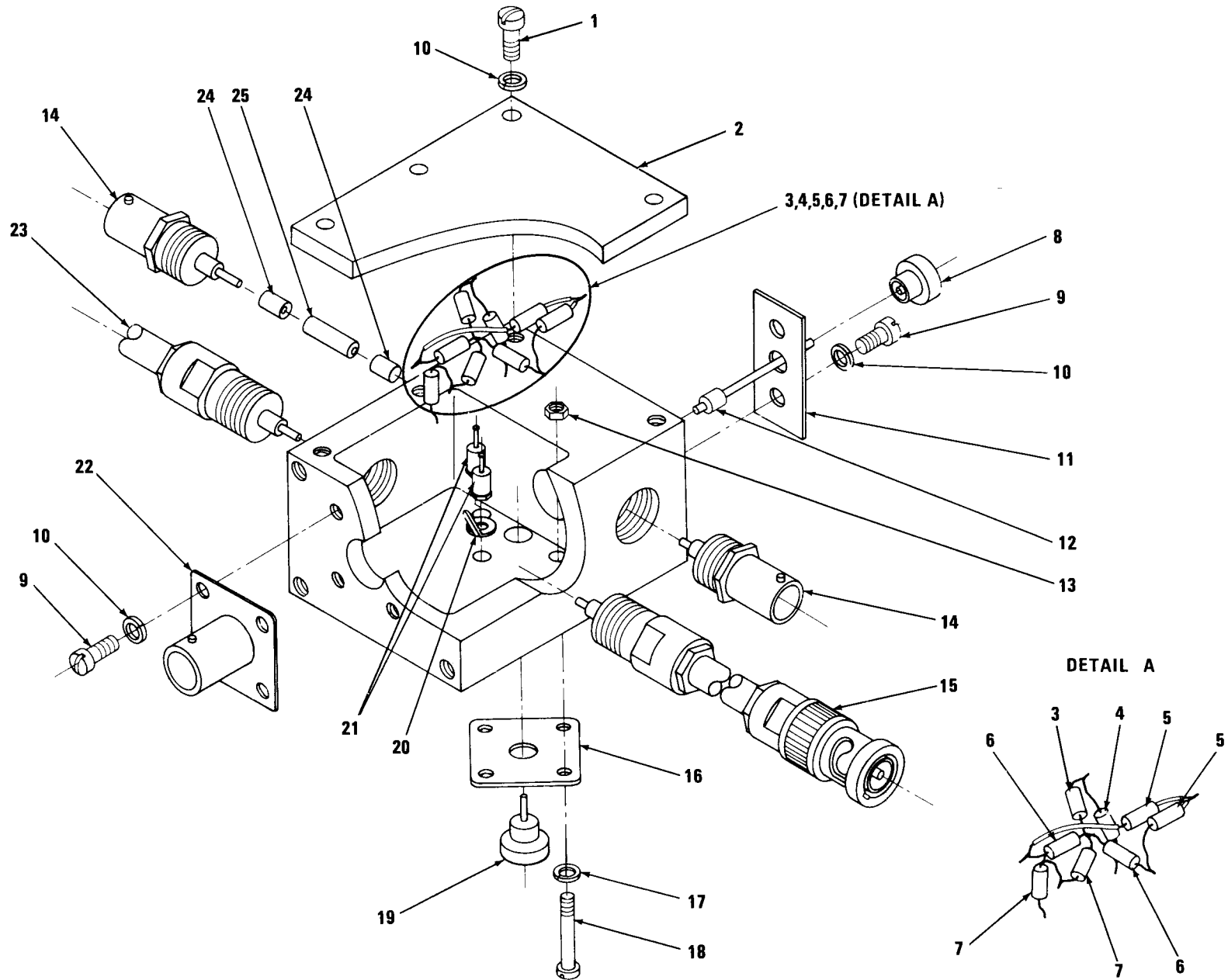
Figure C-24. Monitor/Mixer Subassembly
