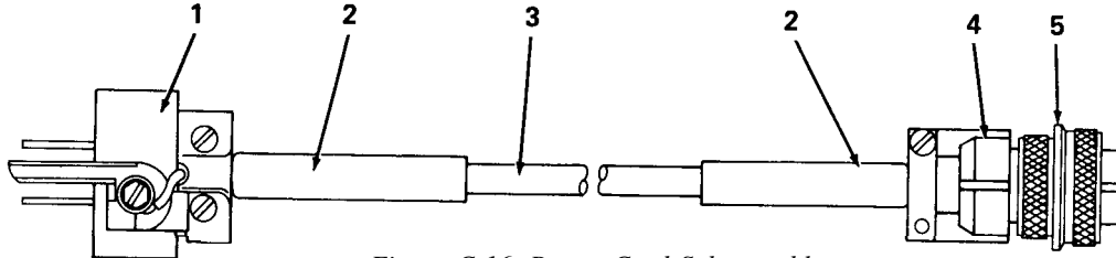
Figure C-16. Power Cord Subassembly
