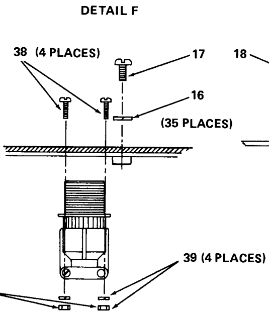
Figure C-1. Sweep Signal Generator SG-677/U (Sheet 4 of 4)
