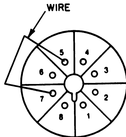
TD1 AND TD2 SOCKET VIEWED FROM TOP
