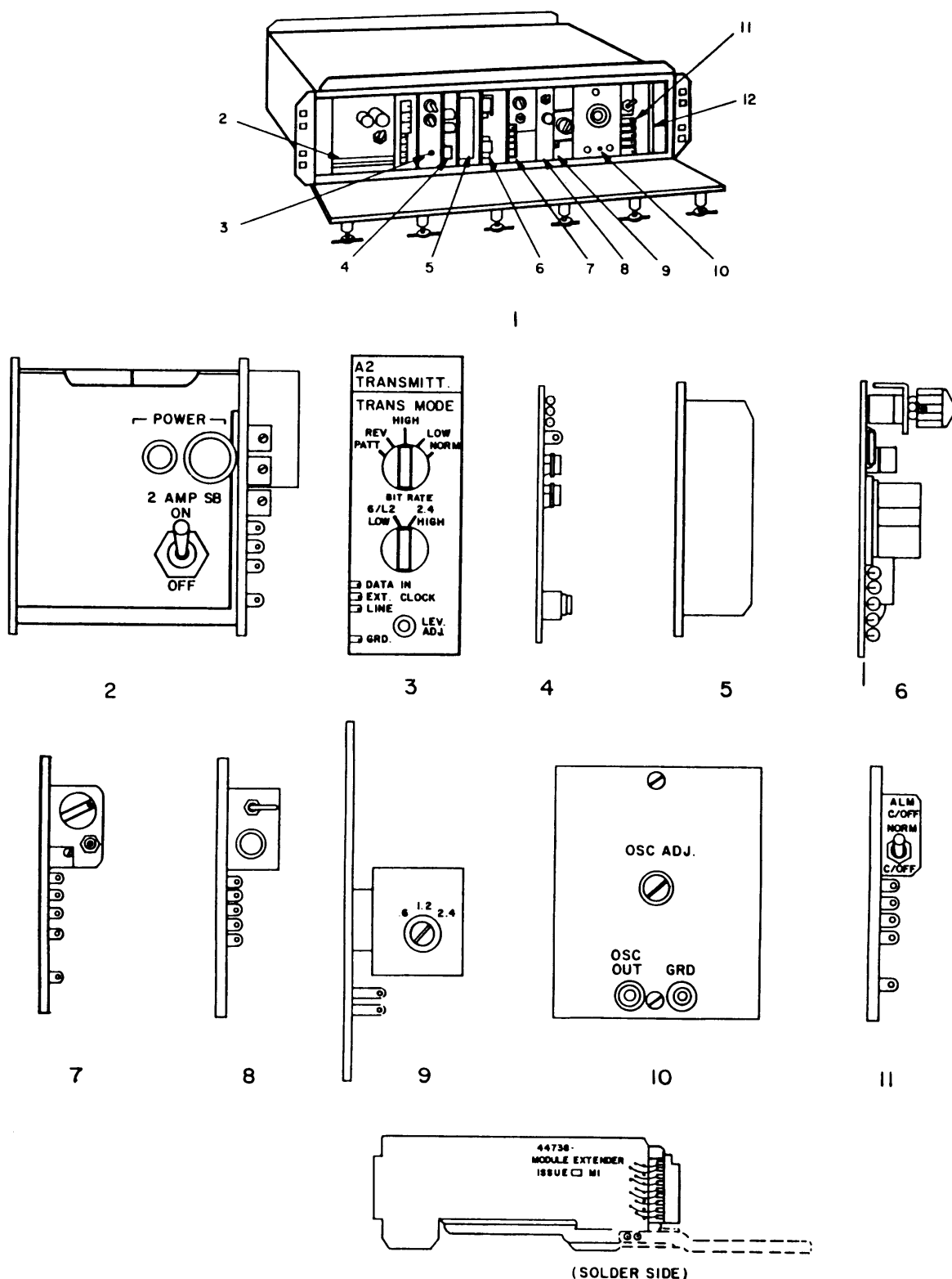
Figure B-1. Components of end item - MODEM MD-701(*)/UY.
