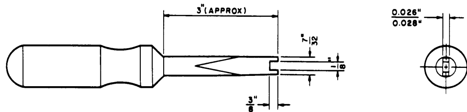
Figure 3. Straddle screwdriver, fabrication details.
