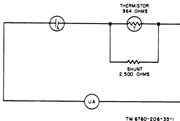
Figure 2, Lightmeter circuit, schematic diagram.
