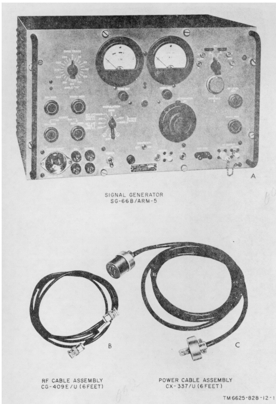
Figure 1-1. Test set, Radio AN/ARM-5A, less running spares.
