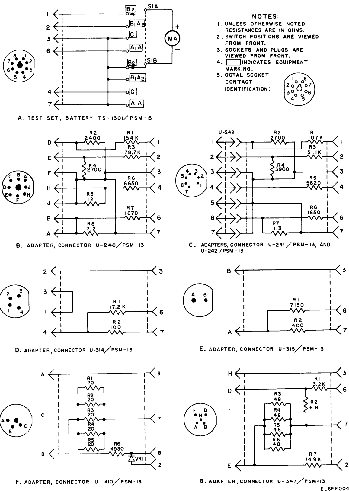
Figure 4-1. Schematic diagram.
