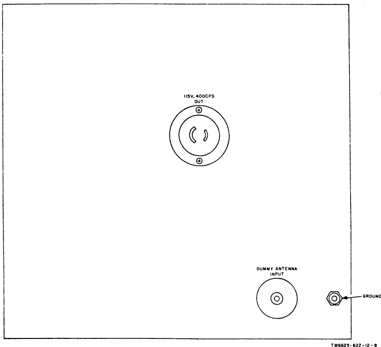
Figure 2-4. Test unit rear panel connectors.
