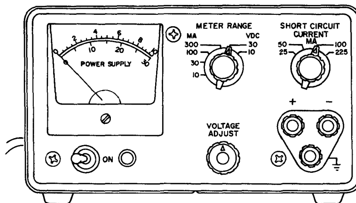
Figure 3. Power Supply PP-3514/U, controls, indicators, and terminals.
