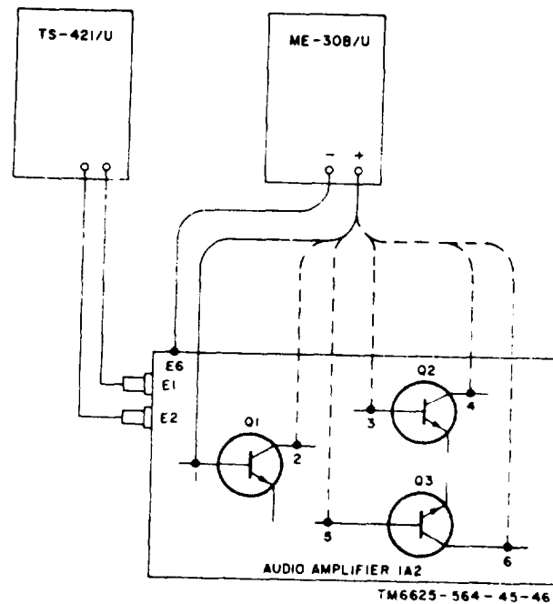
Figure 2-18. Radio set simulator, audio amplifier 1A2 stage gain test setup diagram.
