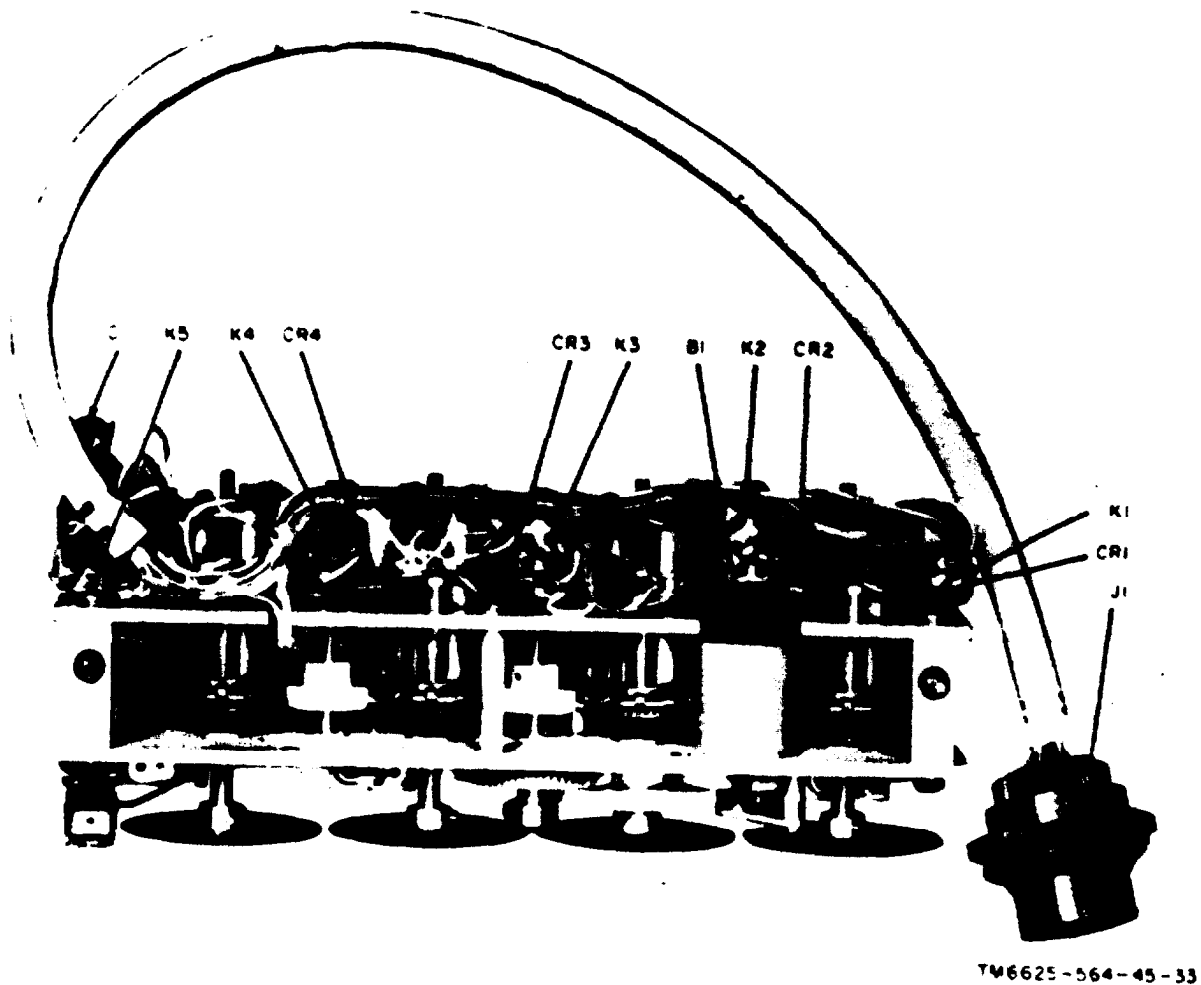
Figure 2-3. Radio set simulator readout mechanism 1A6, bottom view, showing location of parts.
