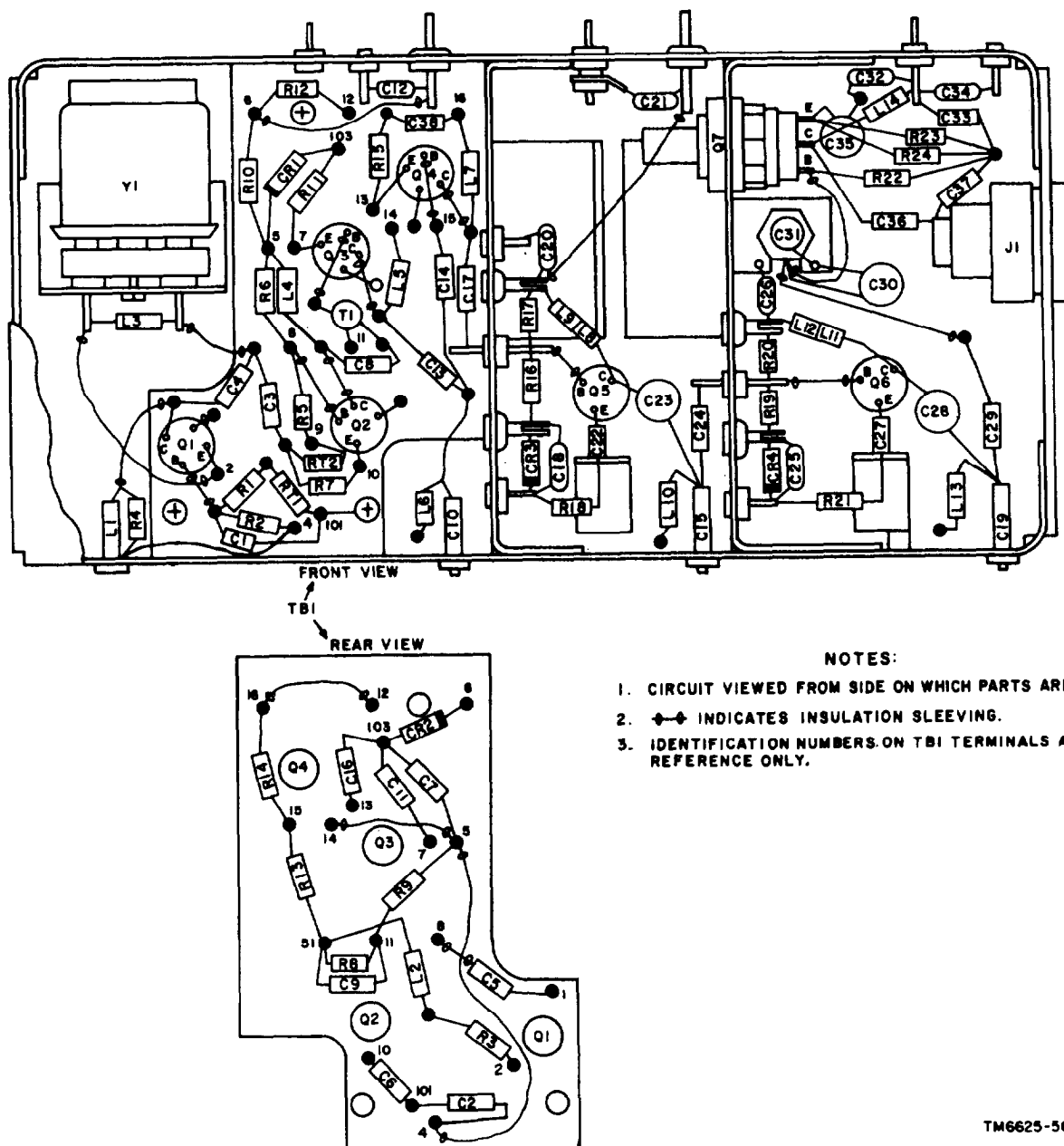
Figure 4-14.1 Radio set simulator, uhf generator 1A5 (MK-731A/ARC-51X only), wiring diagram.
