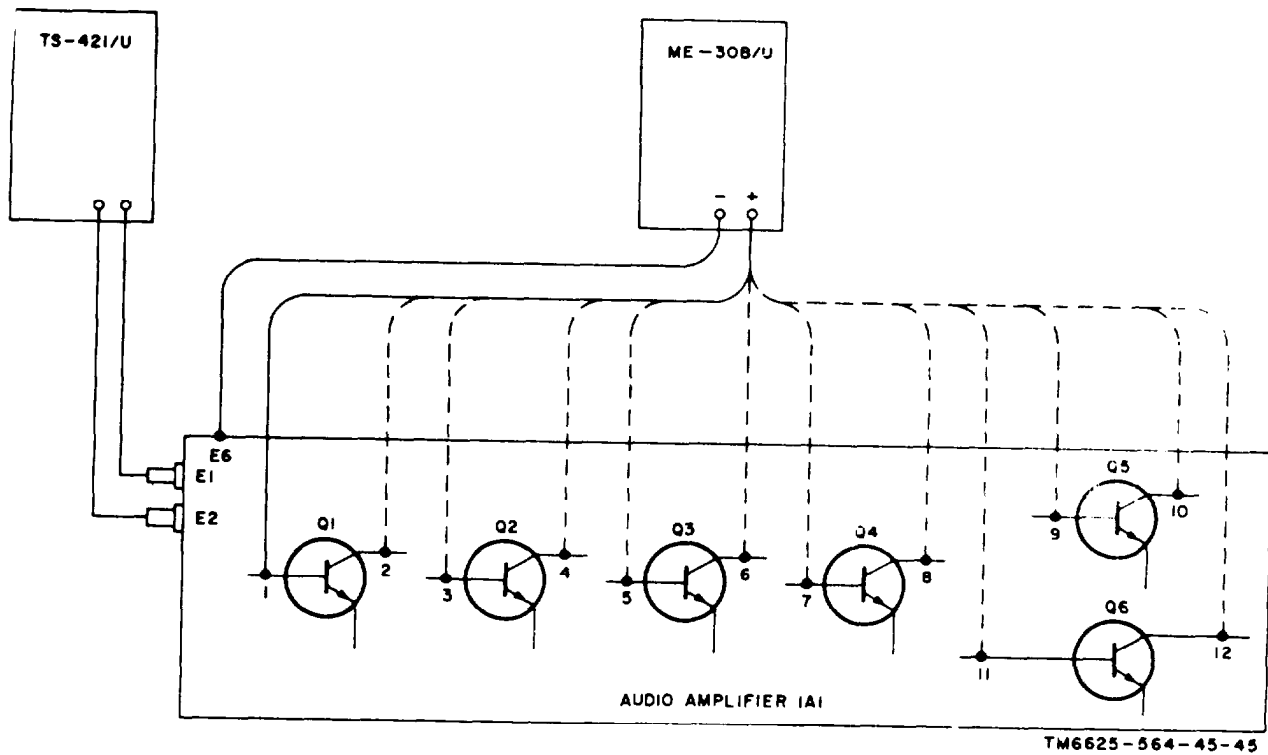
Figure 2-17. Radio set simulator, audio amplifier 1A1 stage gain test setup diagram.
