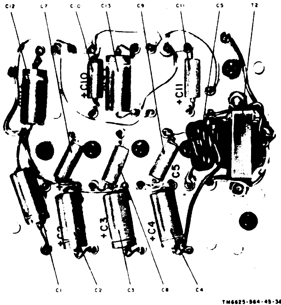
Figure 4-8. Radio set simulator TB1 of audio amplifier 1A1, rear view, showing location of parts.
