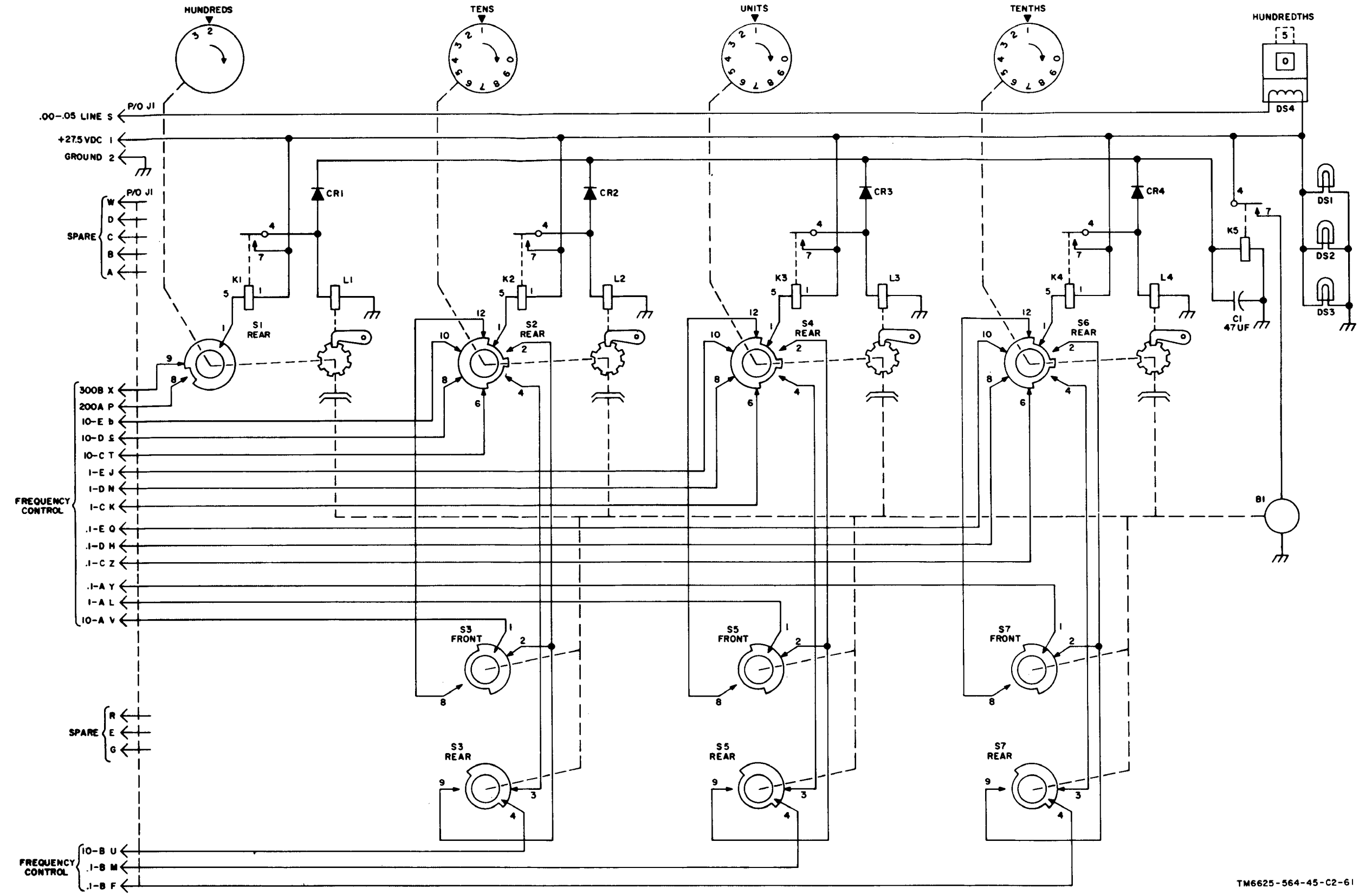
Figure 4-9.1 Radio set simulator readout mechanism (MK-731A/ARC-51X), schematic diagram.
