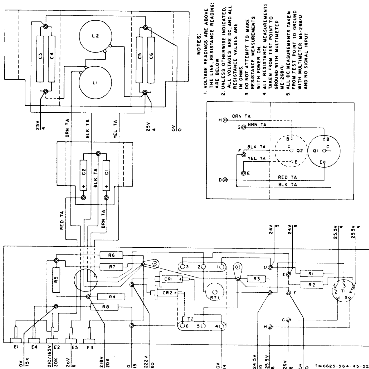
Figure 2-15 Radio set simulator, audio amplifier 1A2, voltage and resistance measurement diagram
