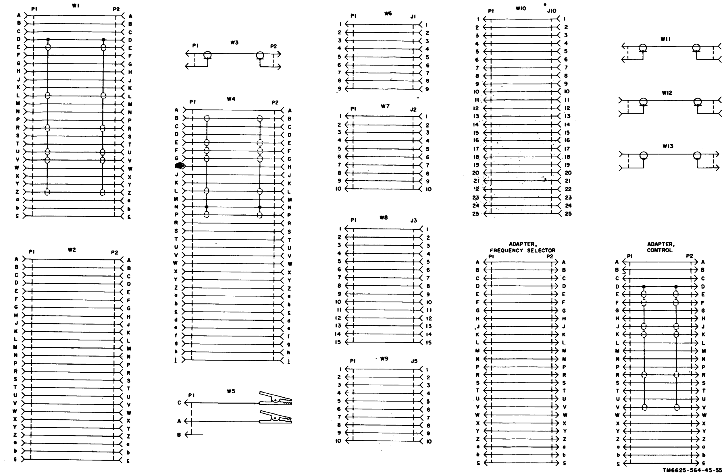
Figure 4-18. Cables W1 through W13 and cable adapters, schematic diagrams.
