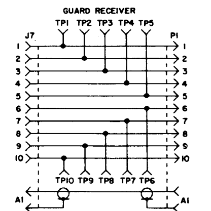
Figure 4-19. Rigid module extenders, schematic diagrams.
