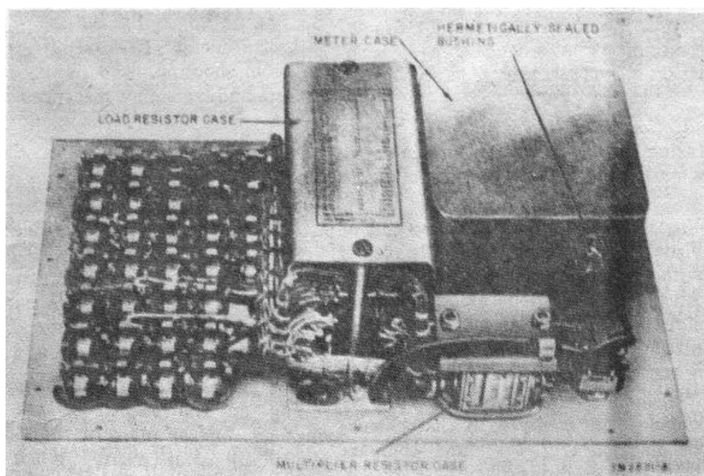
Figure 4-2. Battery Tester TS-183/U , parts location
