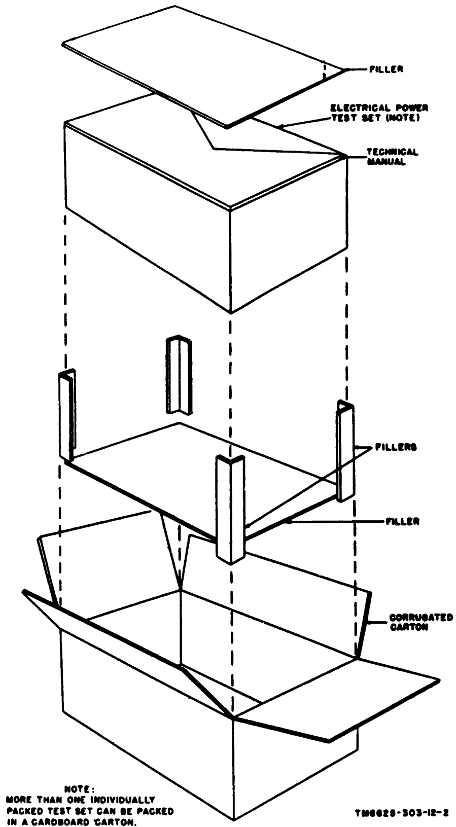
Figure 2. Typical packing.
