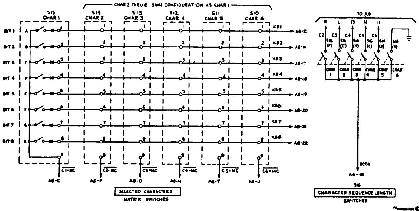
Fig. 51 - Schematic/Wiring Diagram - Selected Character Switches
