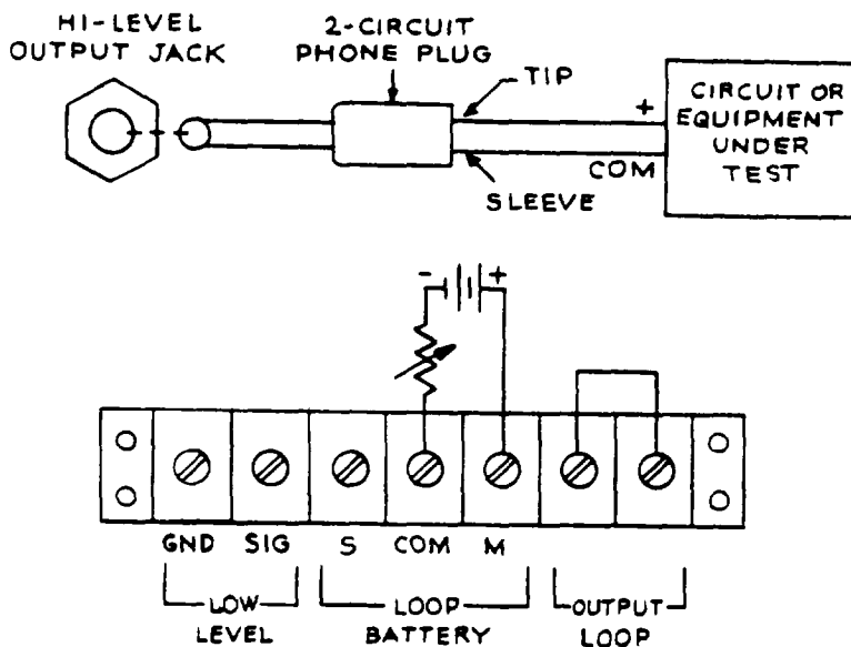
Fig. 7 - High-Level Neutral Operation, Positive Tip, Using Front-Panel Phone Jack for Connection to Loop or Equipment
