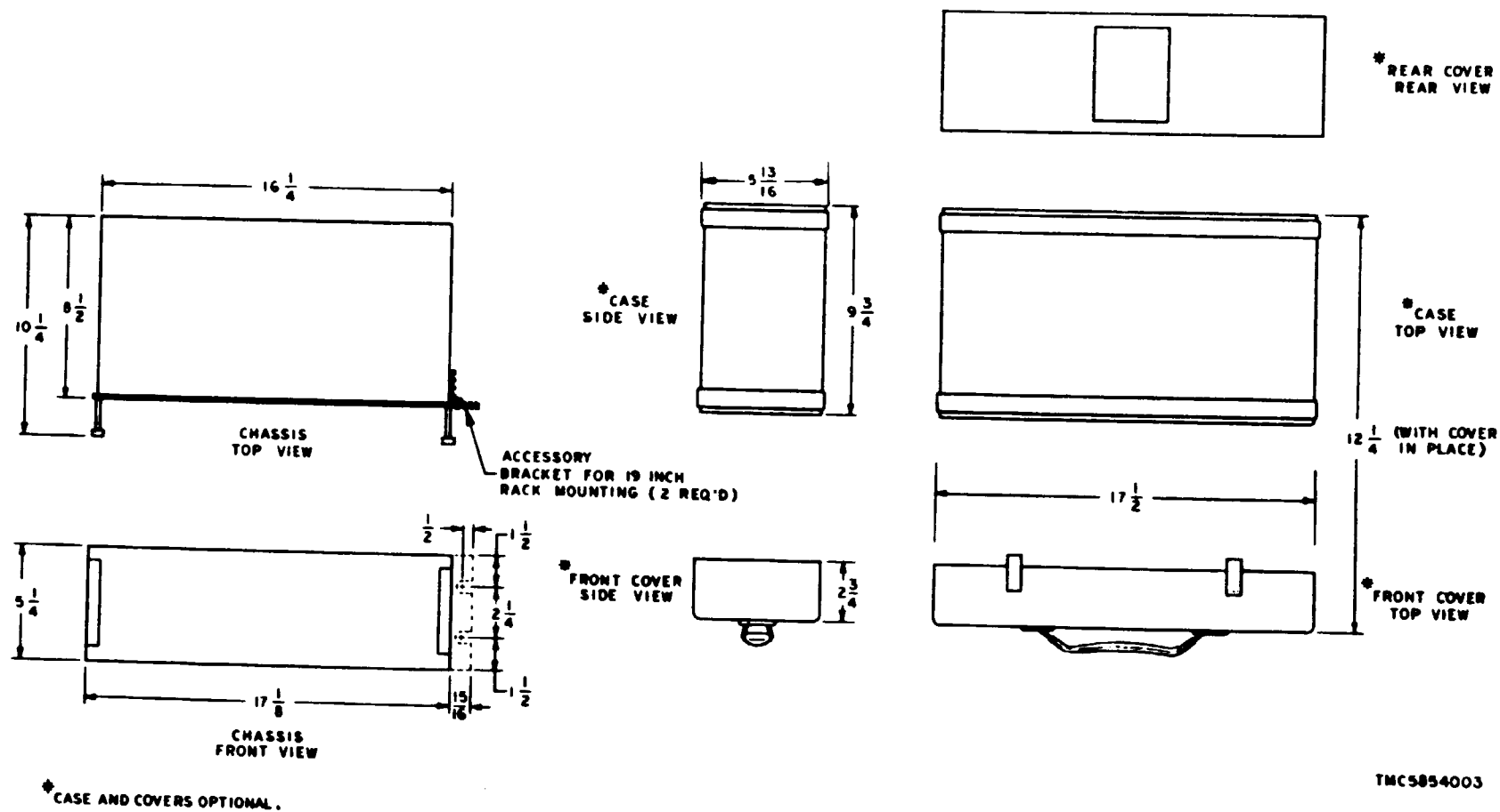
Fig. 6 - Outline Drawing - Pattern Generator
