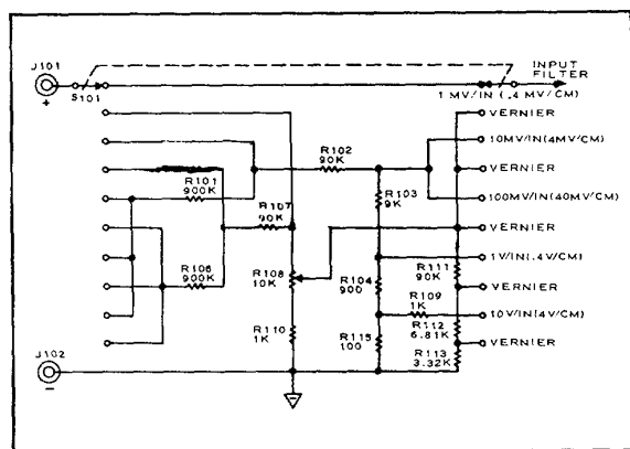
FIGURE 4-3. RANGE SELECTOR
