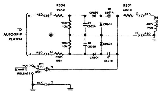
FIGURE 4-14. AUTOGRIP POWER SUPPLY
