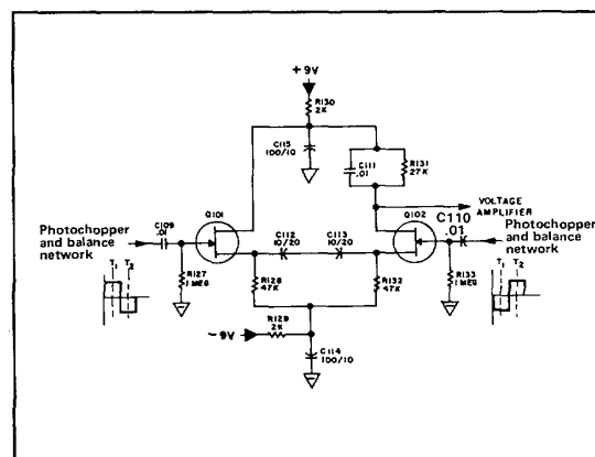
FIGURE 4-8. DIFFERENTIAL AMPLIFIER
