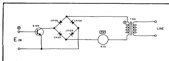
FIGURE 4-11. MOTOR CONTROL AND DEMODULATOR
