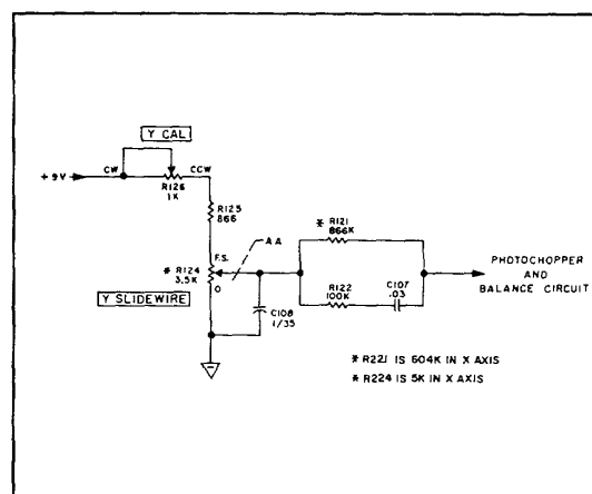
FIGURE 4-6. SLIDEWIRE AND DAMPING CIRCUIT
