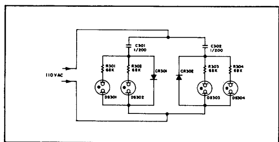
FIGURE 4-13. NEON DRIVER
