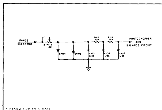
FIGURE 4-4. INPUT FILTER
