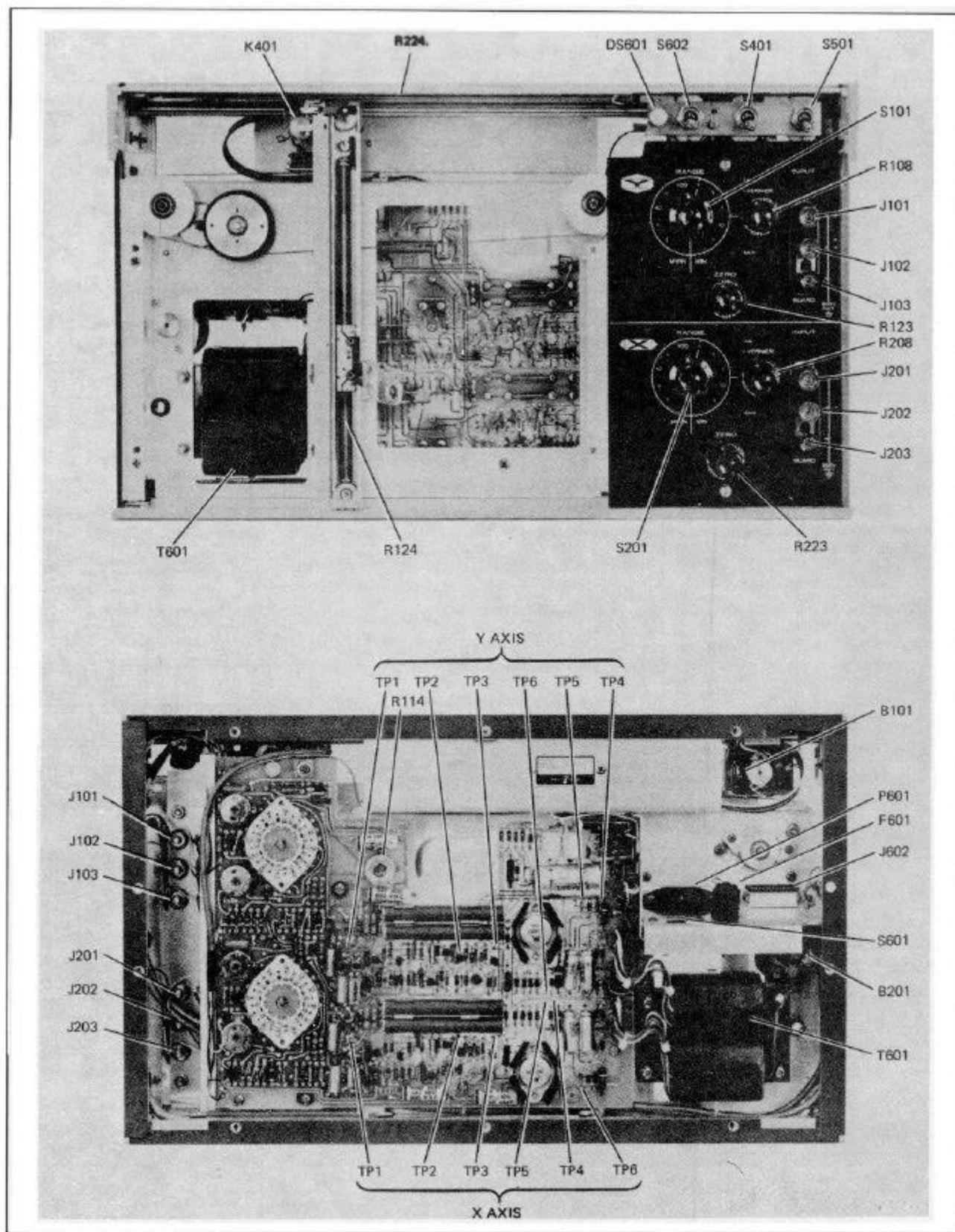
FIGURE 7-1. COMPONENT IDENTIFICATION-FRAME
