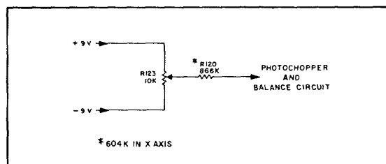
FIGURE 4-5. ZERO CIRCUIT
