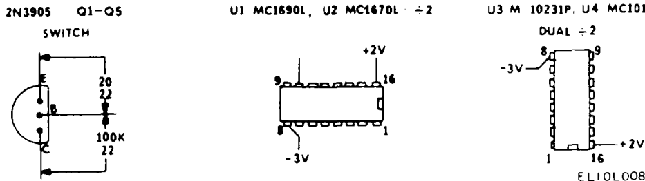
Figure 7-5. Rf divider board A8A1, circuit measurements
