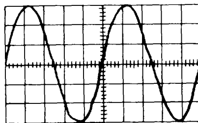
(b) OSCILLOSCOPE DISPLAY OF A7U1TP1 VERTICAL: 5V/DIV AC COUPLED HORIZONTAL: 5MSEC/DIV
