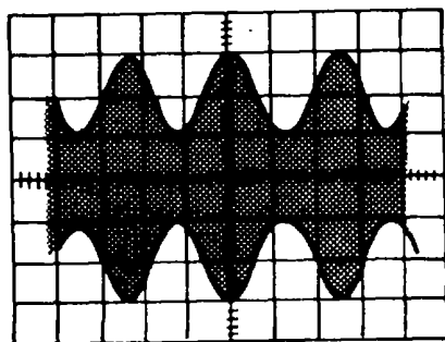
(e) OSCILLOSCOPE DISPLAY OF 50% A.M.
