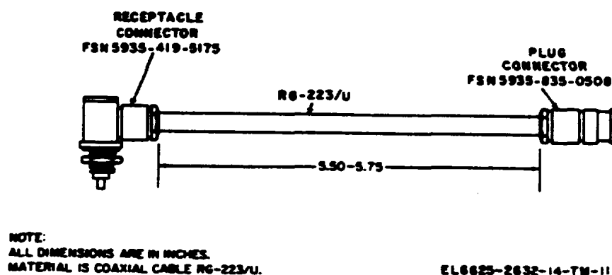
Figure 5-5. Cable assembly fabrication details.
