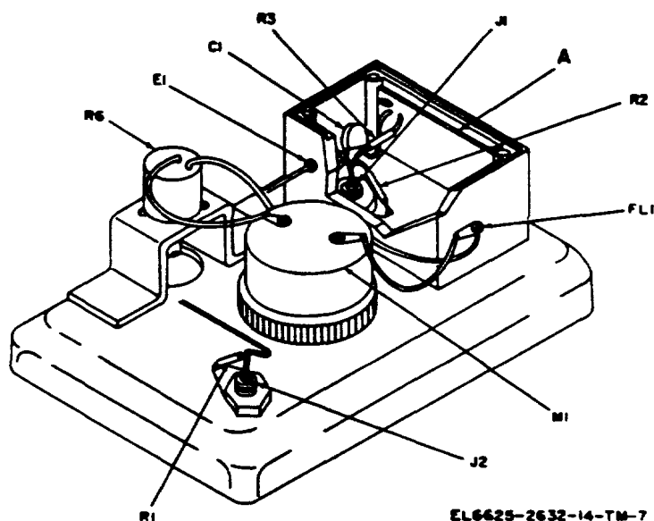
Figure 5-1. Radio Test Set AN/PRM-2 component identification.
