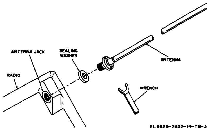
Figure 2-1. Antenna removal from Radio Set AN/PRC-90.
